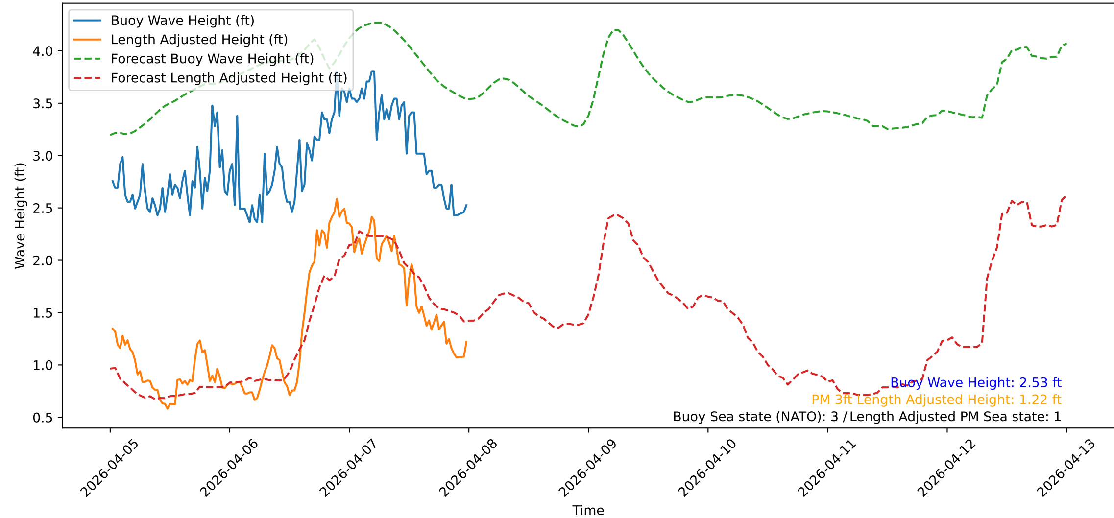
Wave Heights over Time for Green Beach at 2026-04-08 00:21:09
