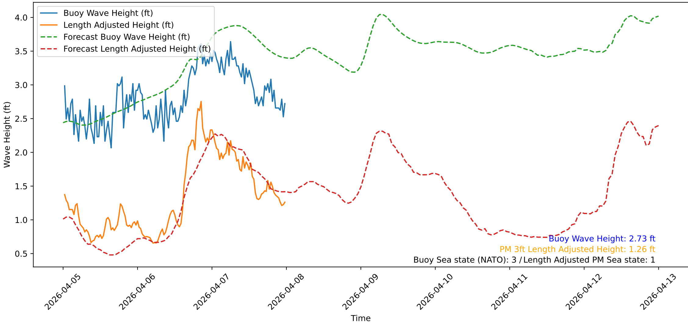
Wave Heights over Time for Oceanside Harbor at 2026-04-08 00:20:31
