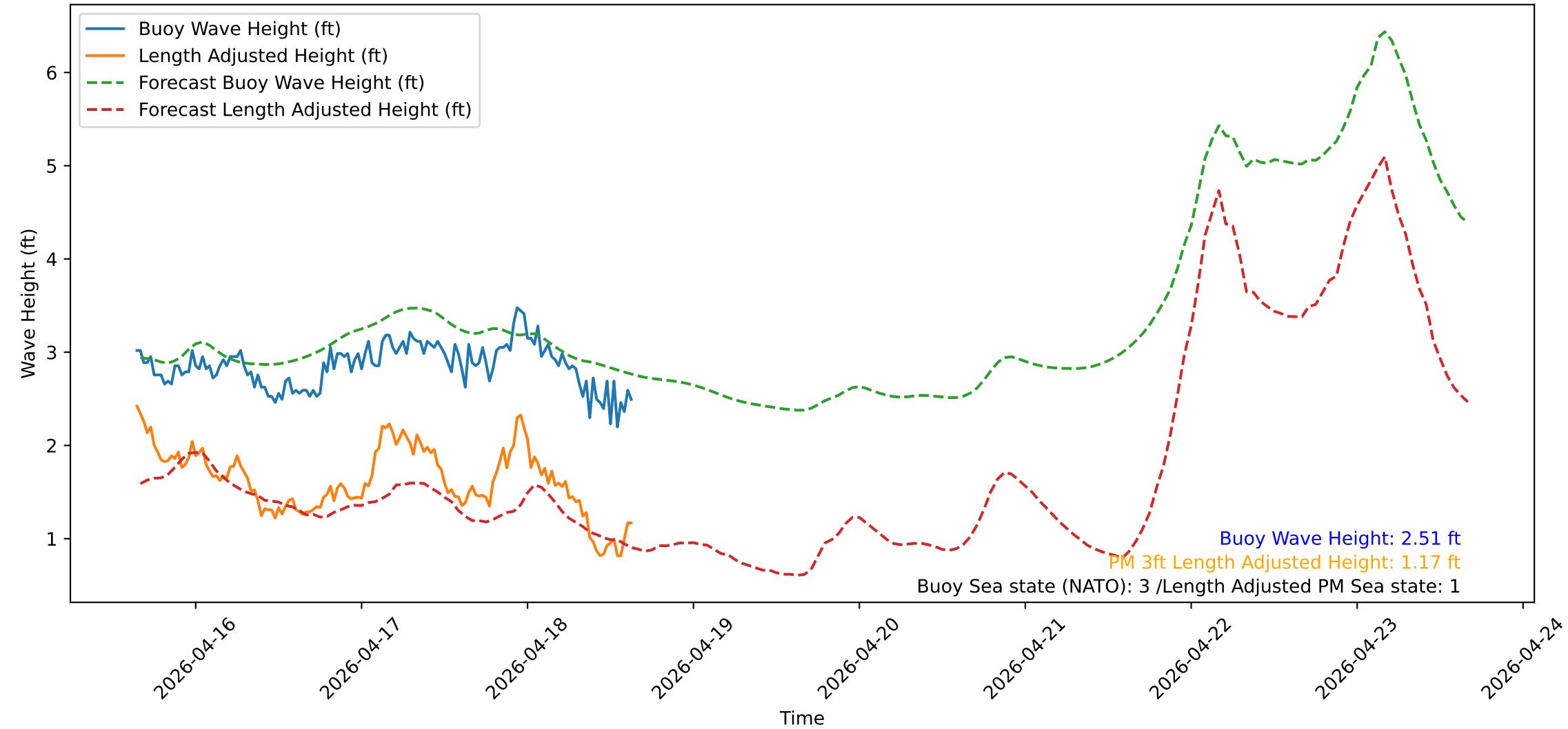
Wave Heights over Time for Green Beach at 2026-04-18 15:41:14
