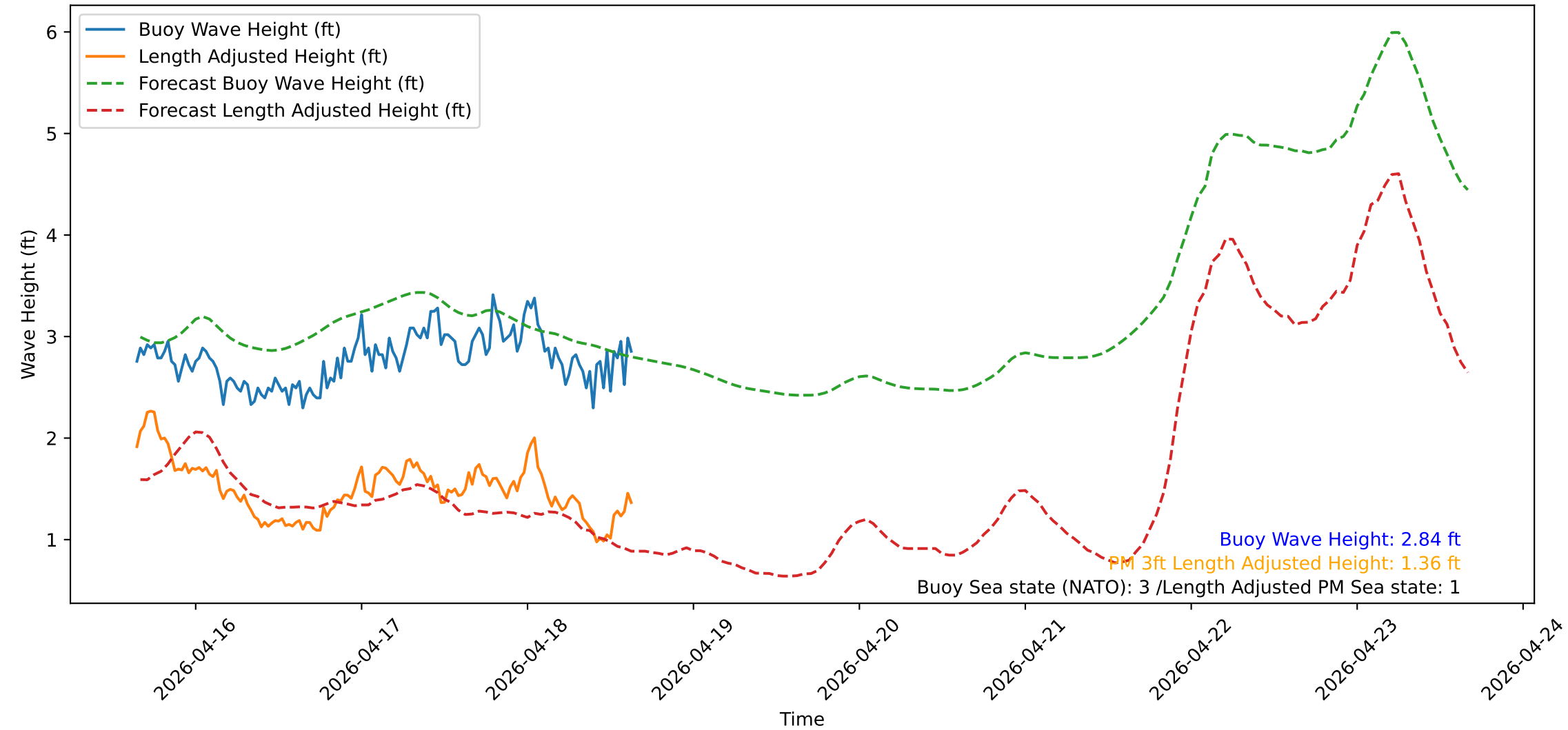
Wave Heights over Time for Oceanside Harbor at 2026-04-18 15:40:32
