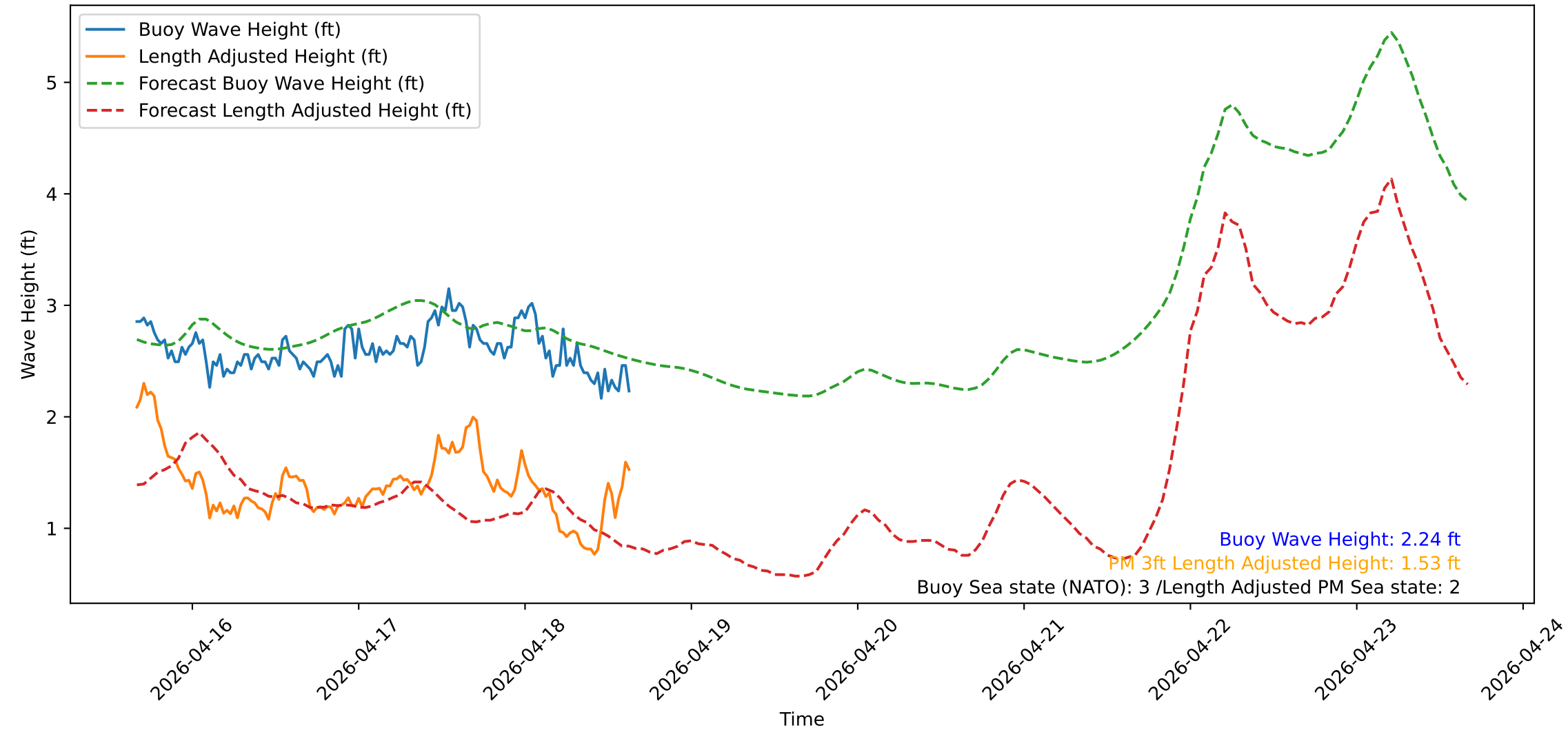
Wave Heights over Time for Red Beach at 2026-04-18 15:40:51
