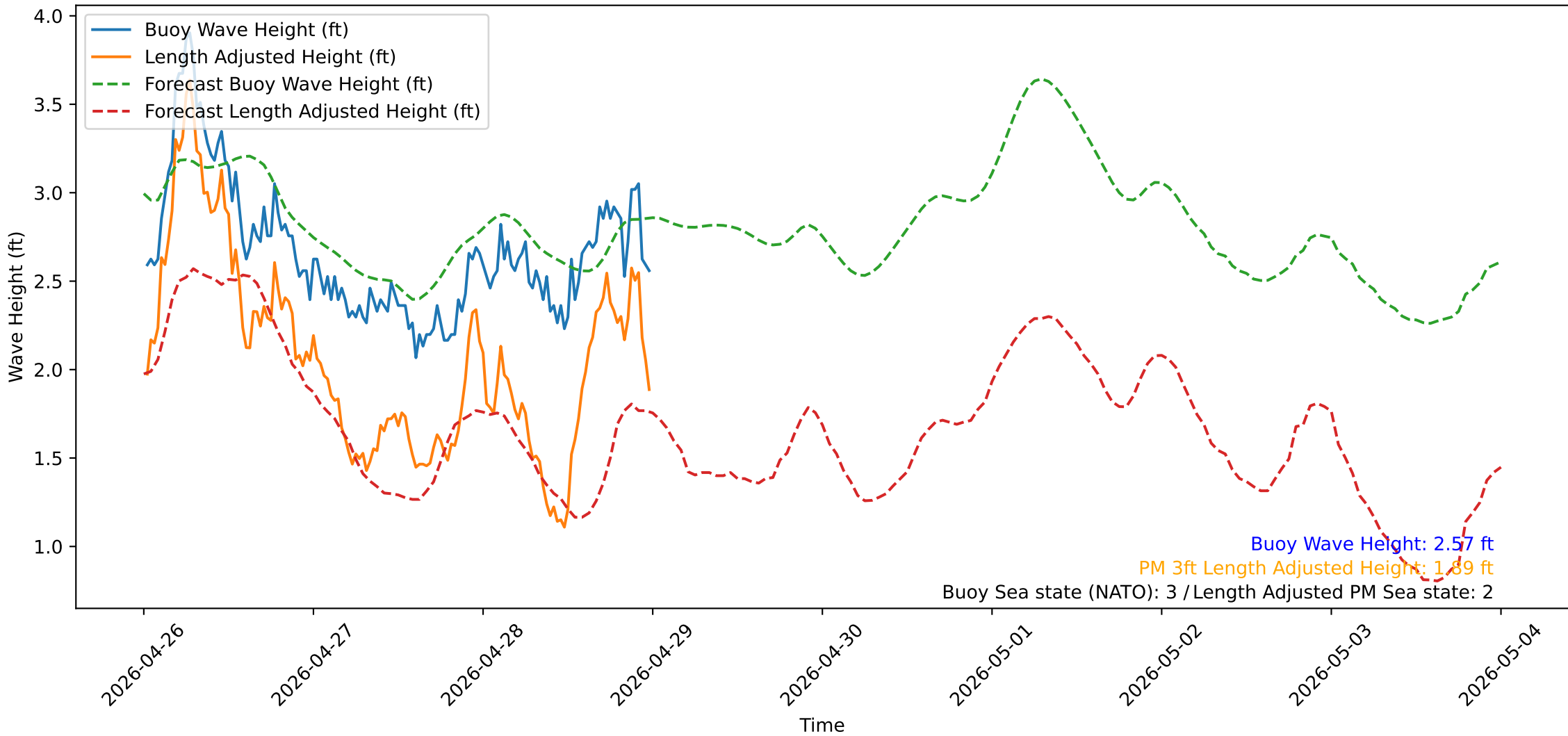
Wave Heights over Time for Oceanside Harbor at 2026-04-29 00:20:31
