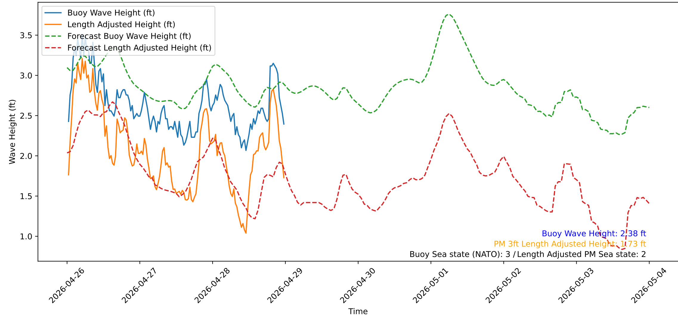
Wave Heights over Time for Green Beach at 2026-04-29 00:21:14
