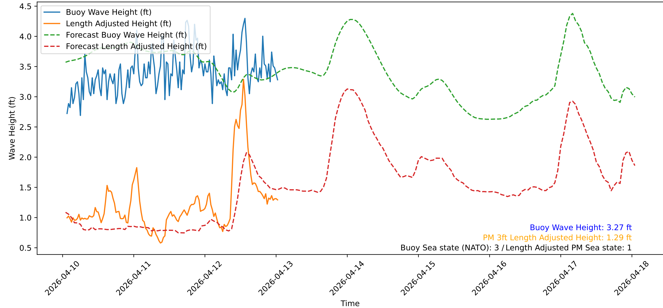
Wave Heights over Time for Red Beach at 2026-04-13 01:10:50
