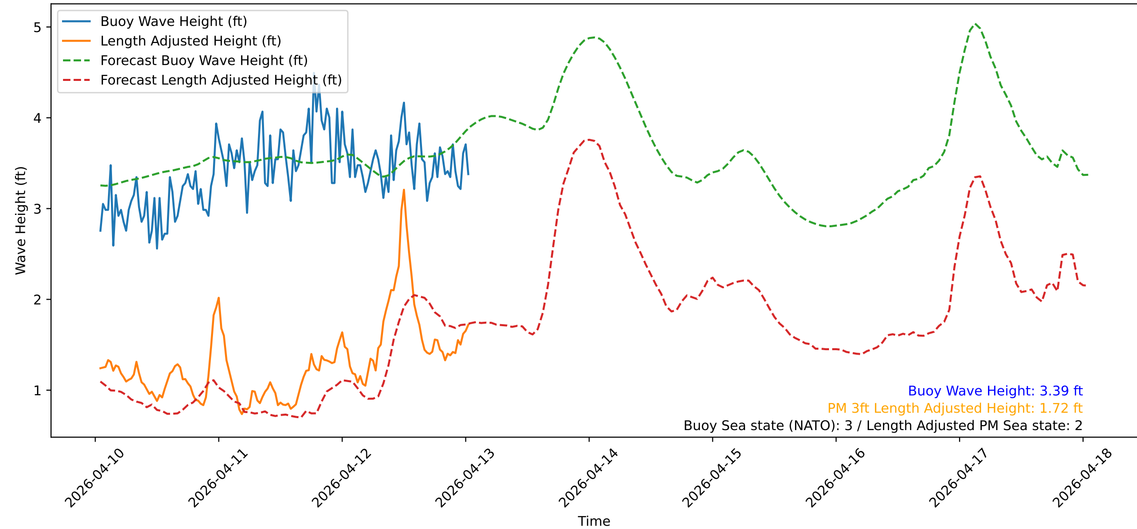
Wave Heights over Time for Green Beach at 2026-04-13 01:11:12
