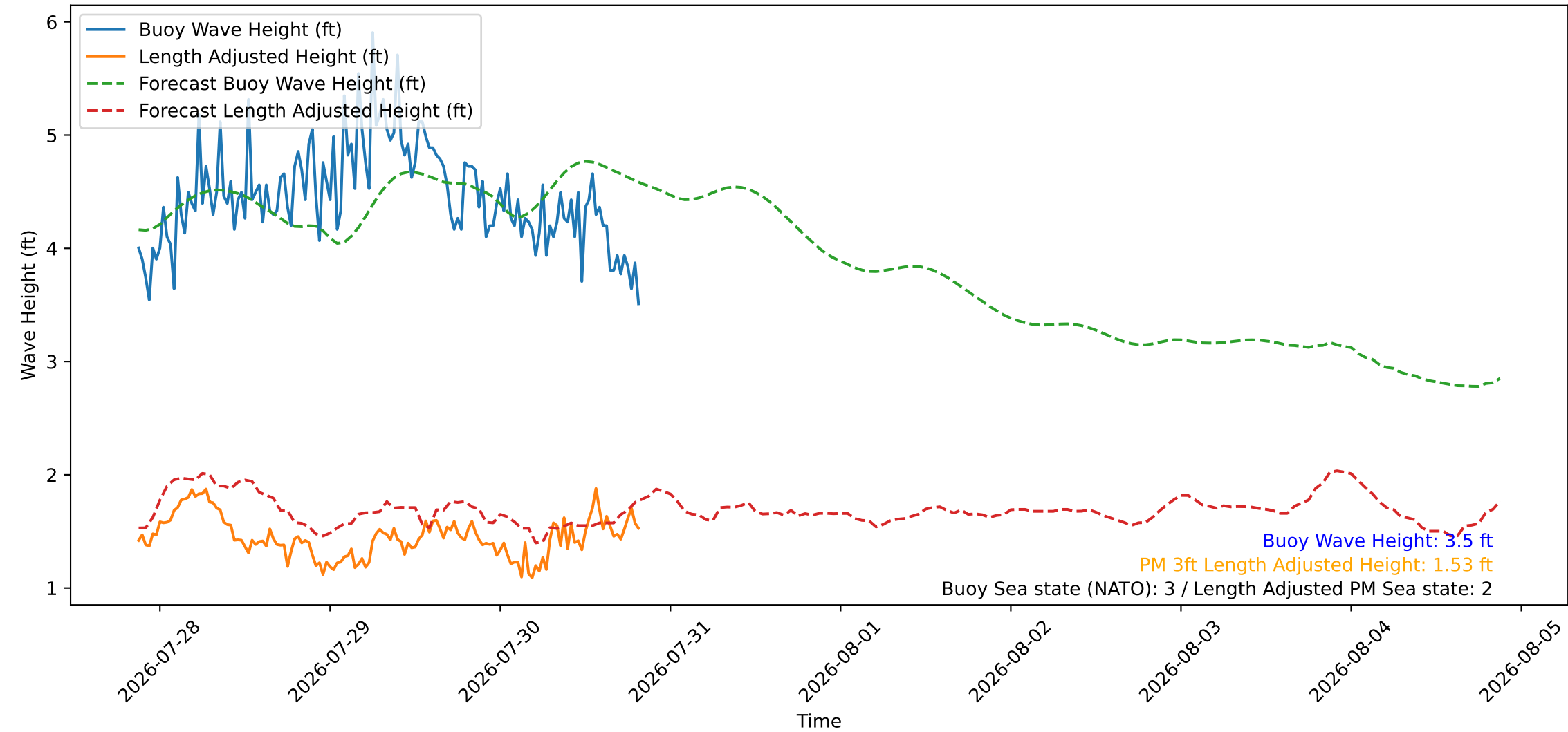
Wave Heights over Time for Oceanside Harbor at 2026-07-30 21:00:26
