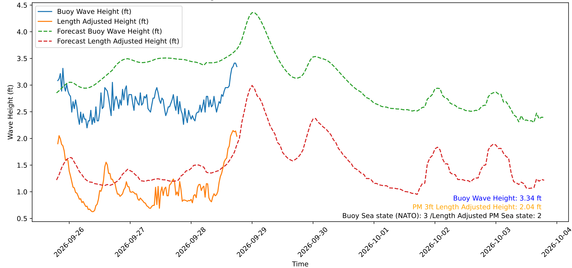
Wave Heights over Time for Red Beach at 2026-09-28 19:00:48
