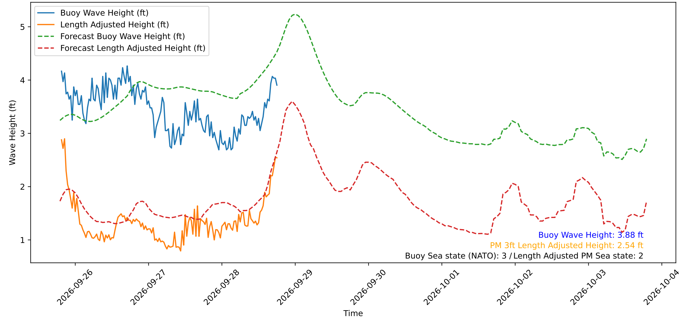
Wave Heights over Time for Green Beach at 2026-09-28 19:01:11
