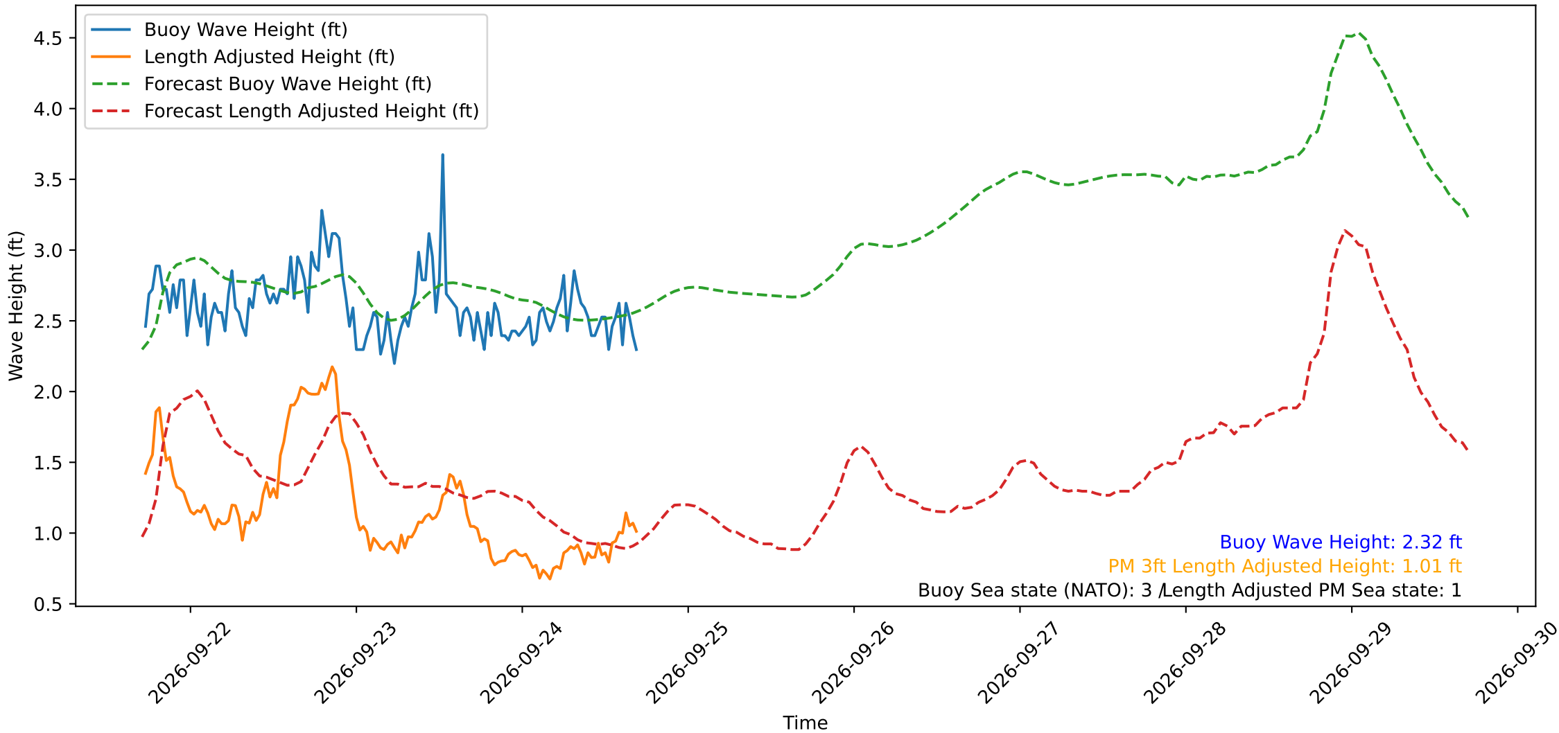
Wave Heights over Time for Red Beach at 2026-09-24 17:20:50
