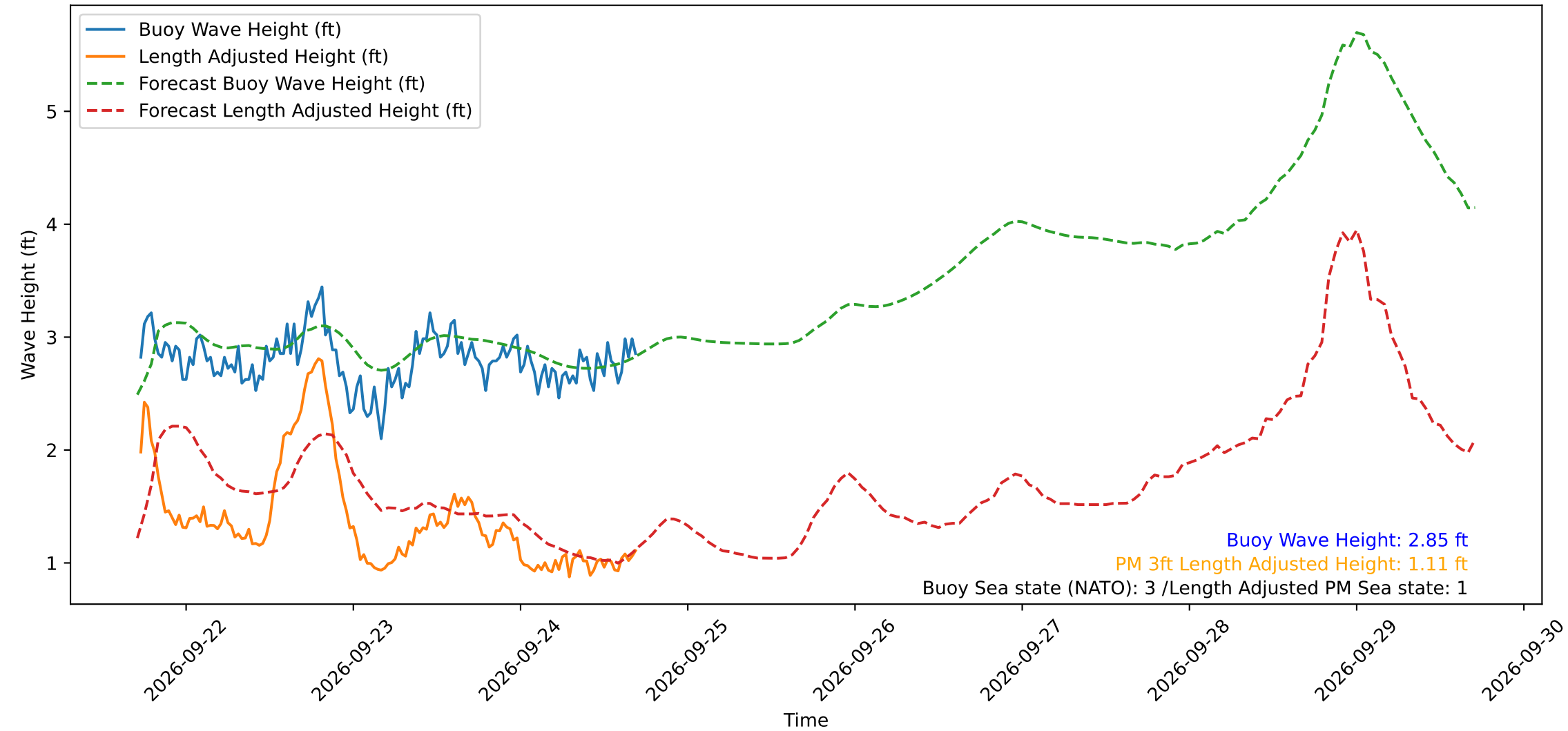
Wave Heights over Time for Green Beach at 2026-09-24 17:21:14
