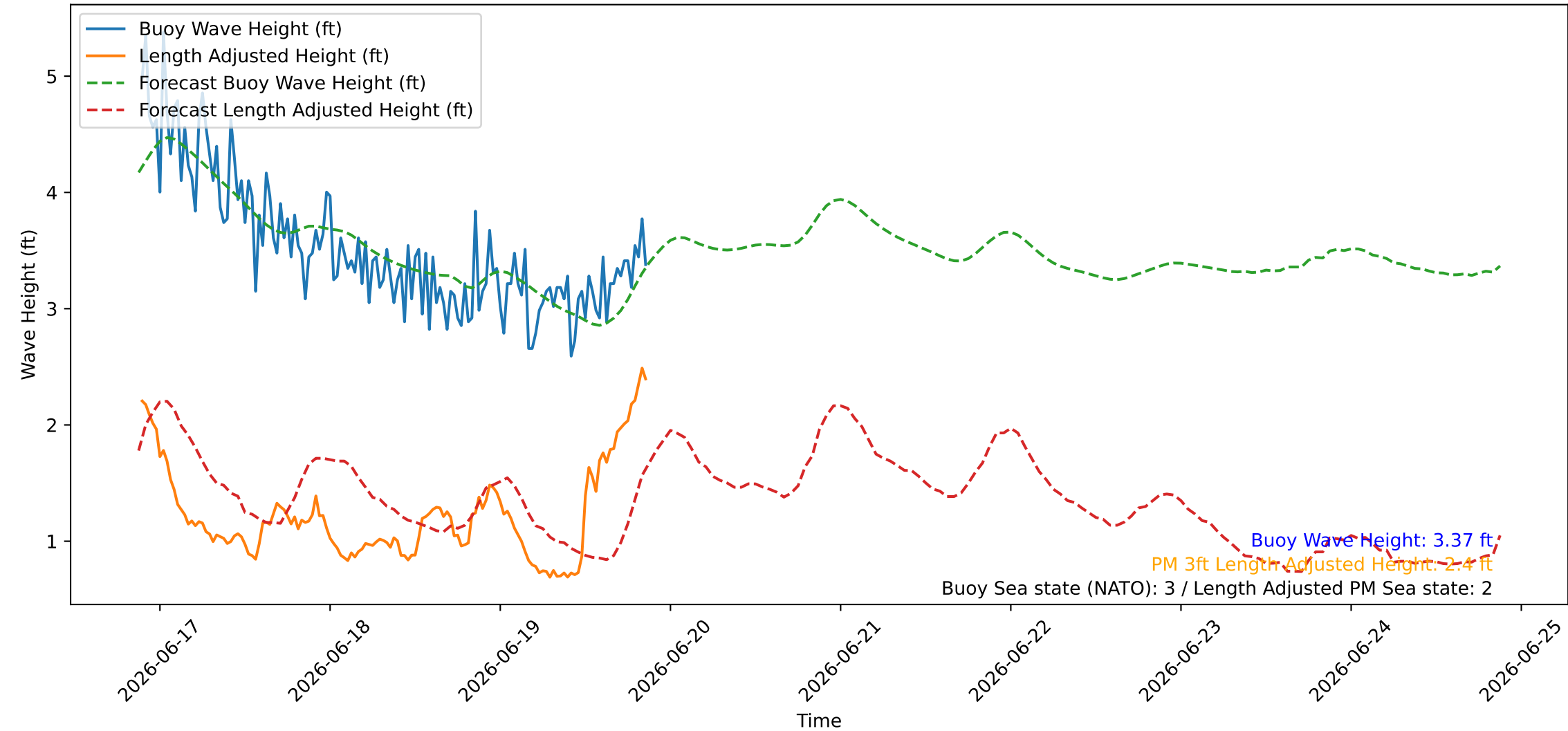
Wave Heights over Time for Red Beach at 2026-06-19 21:20:47
