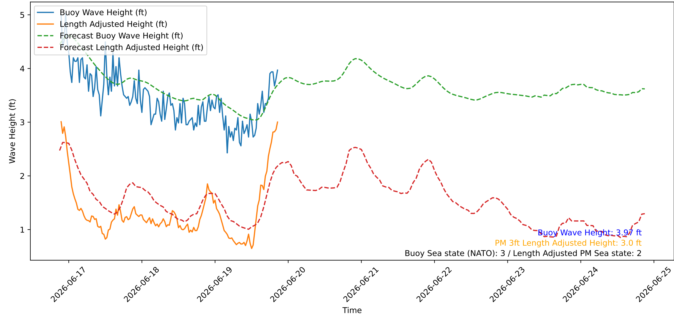
Wave Heights over Time for Green Beach at 2026-06-19 21:21:10
