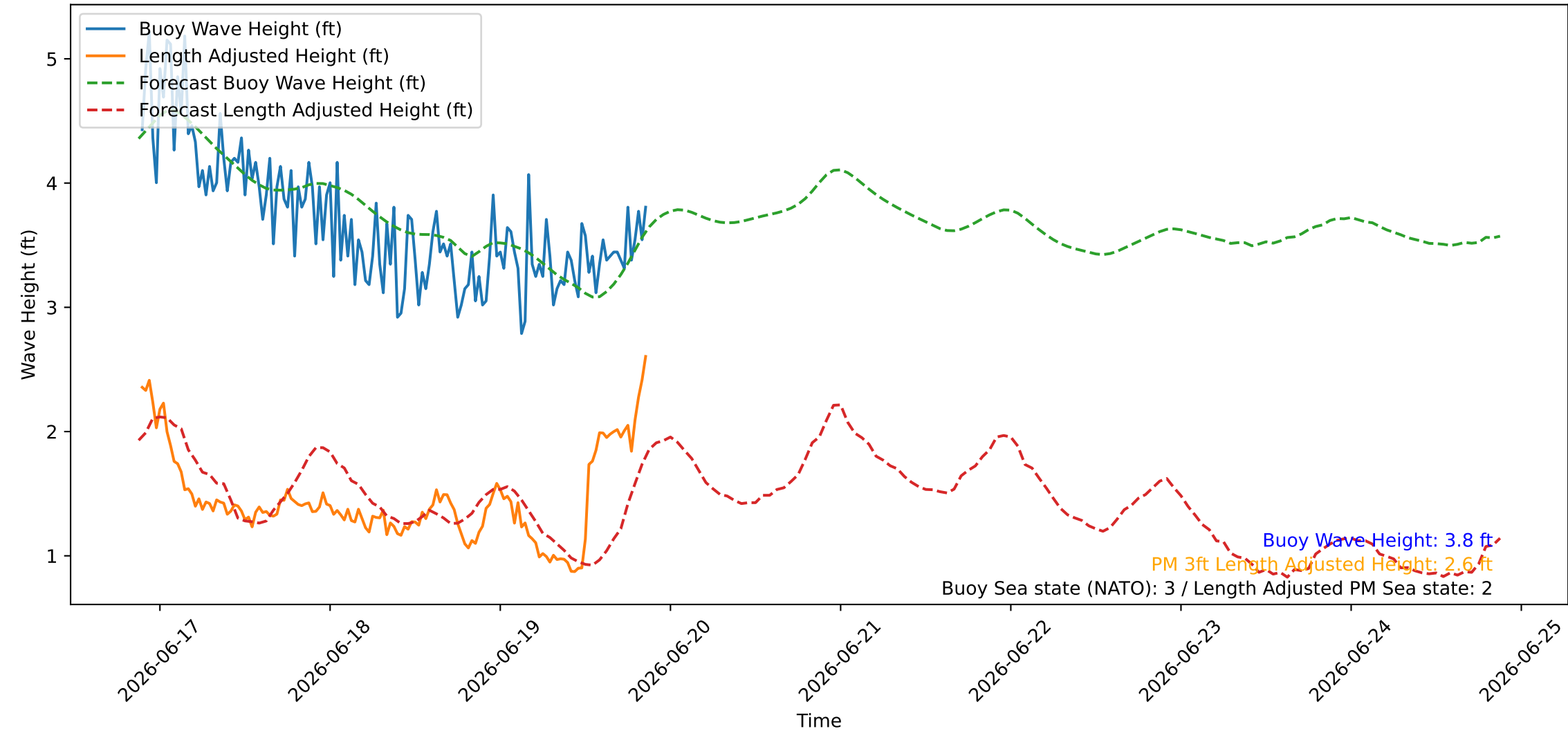
Wave Heights over Time for Oceanside Harbor at 2026-06-19 21:20:26
