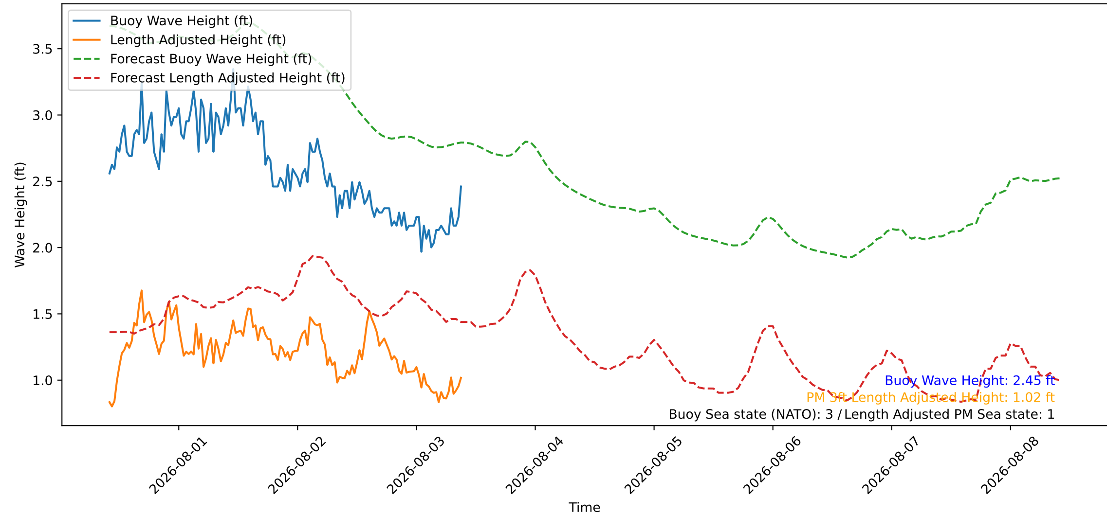
Wave Heights over Time for Red Beach at 2026-08-03 09:50:46
