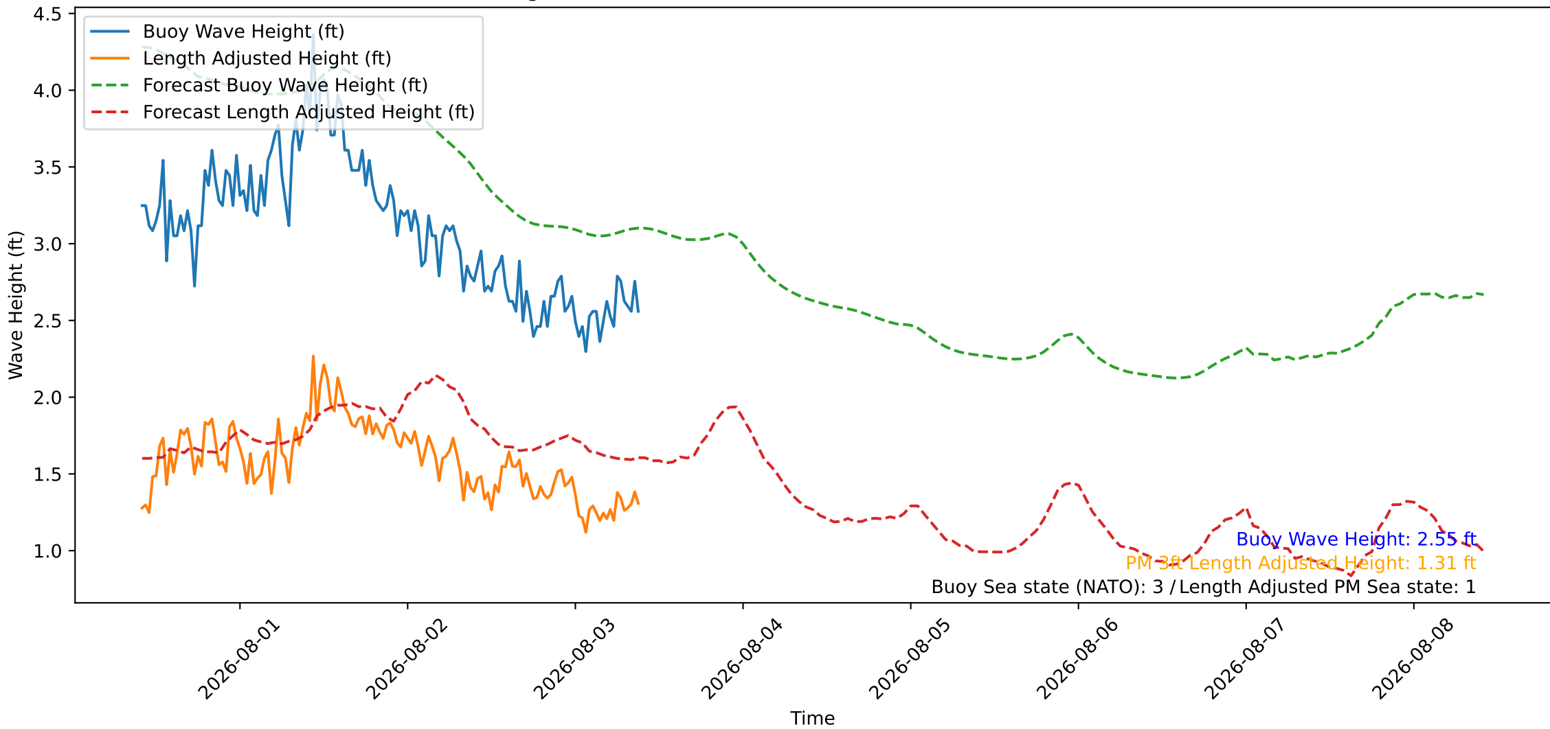
Wave Heights over Time for Oceanside Harbor at 2026-08-03 09:50:26
