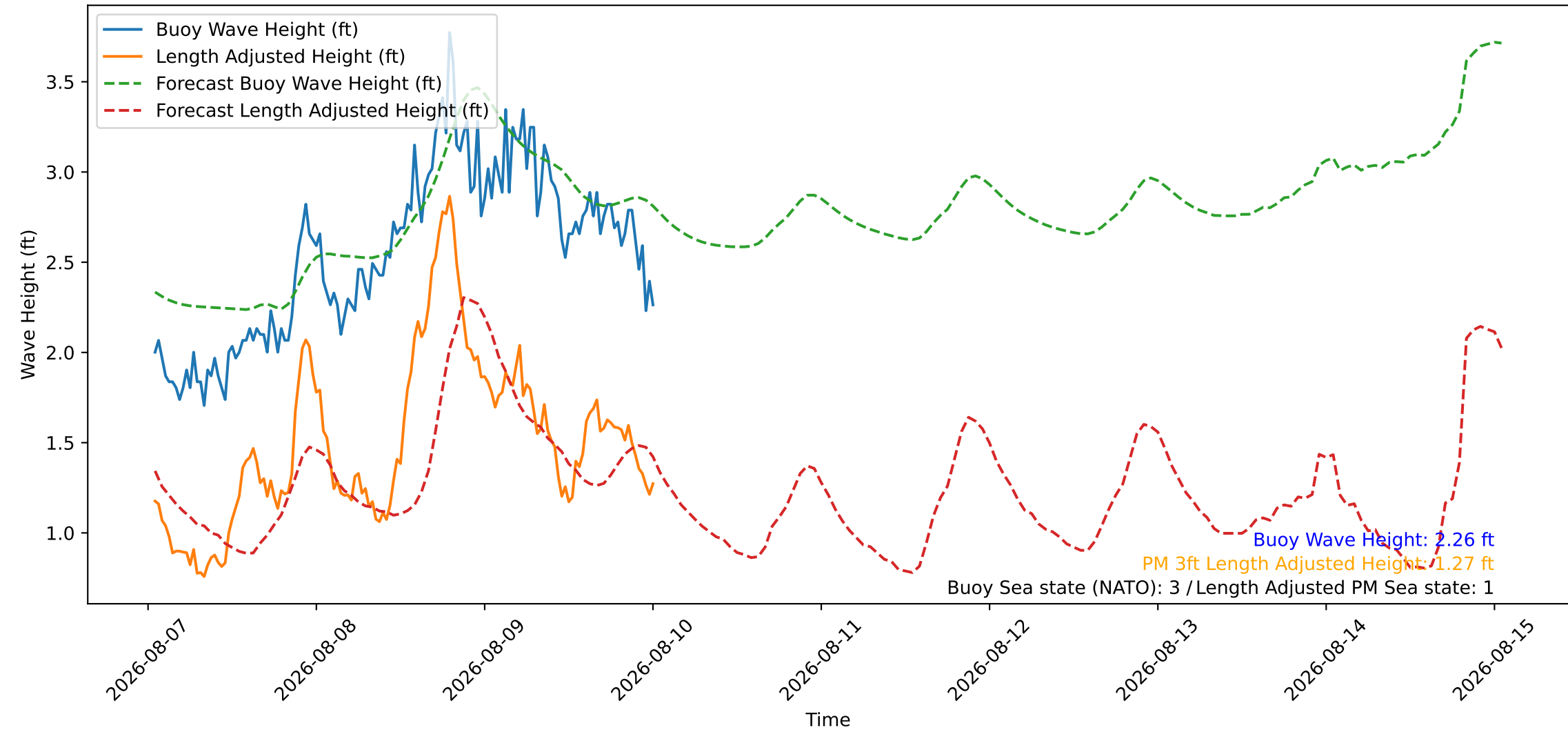
Wave Heights over Time for Green Beach at 2026-08-10 00:51:09
