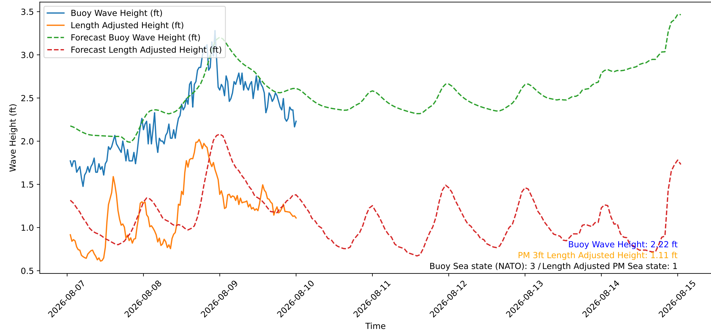
Wave Heights over Time for Red Beach at 2026-08-10 00:50:47
