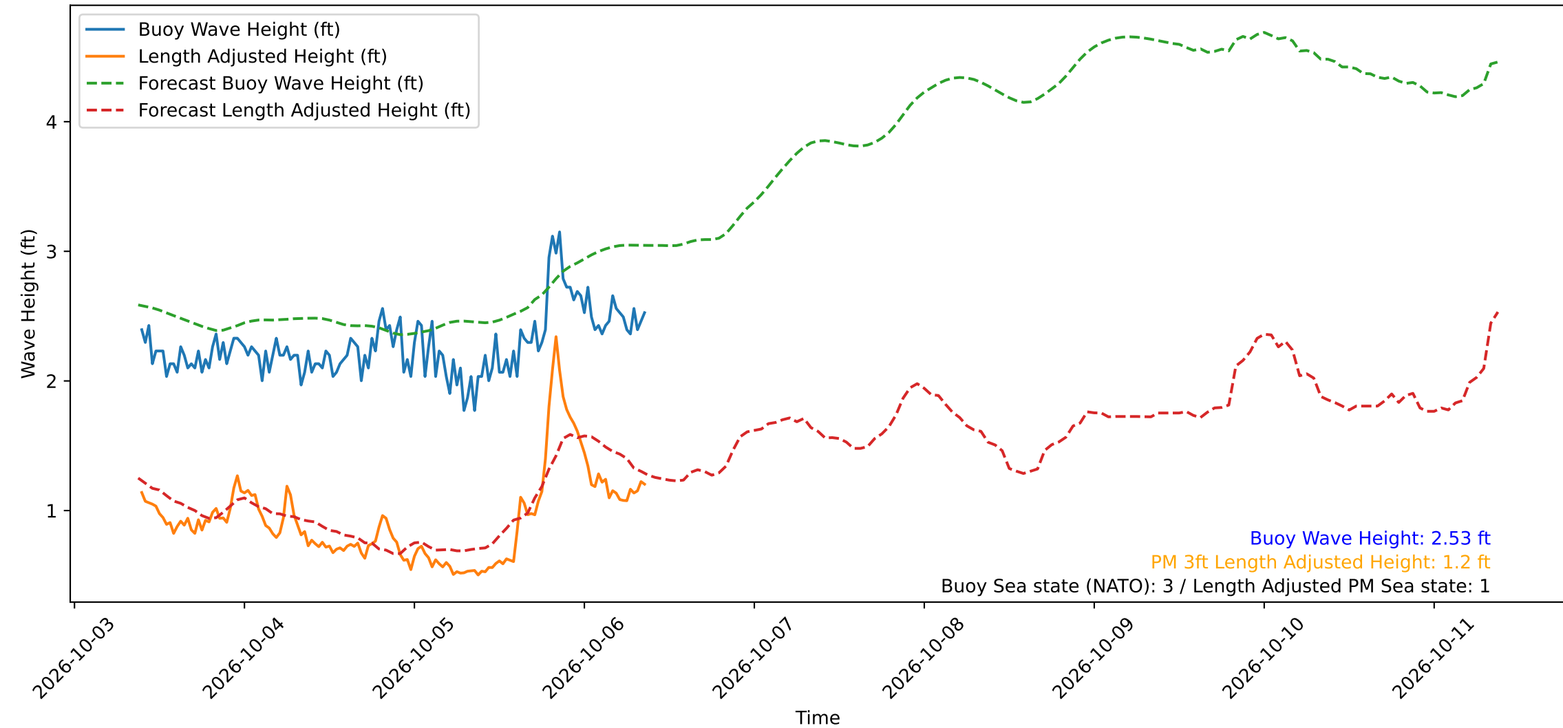
Wave Heights over Time for Green Beach at 2026-10-06 09:11:12
