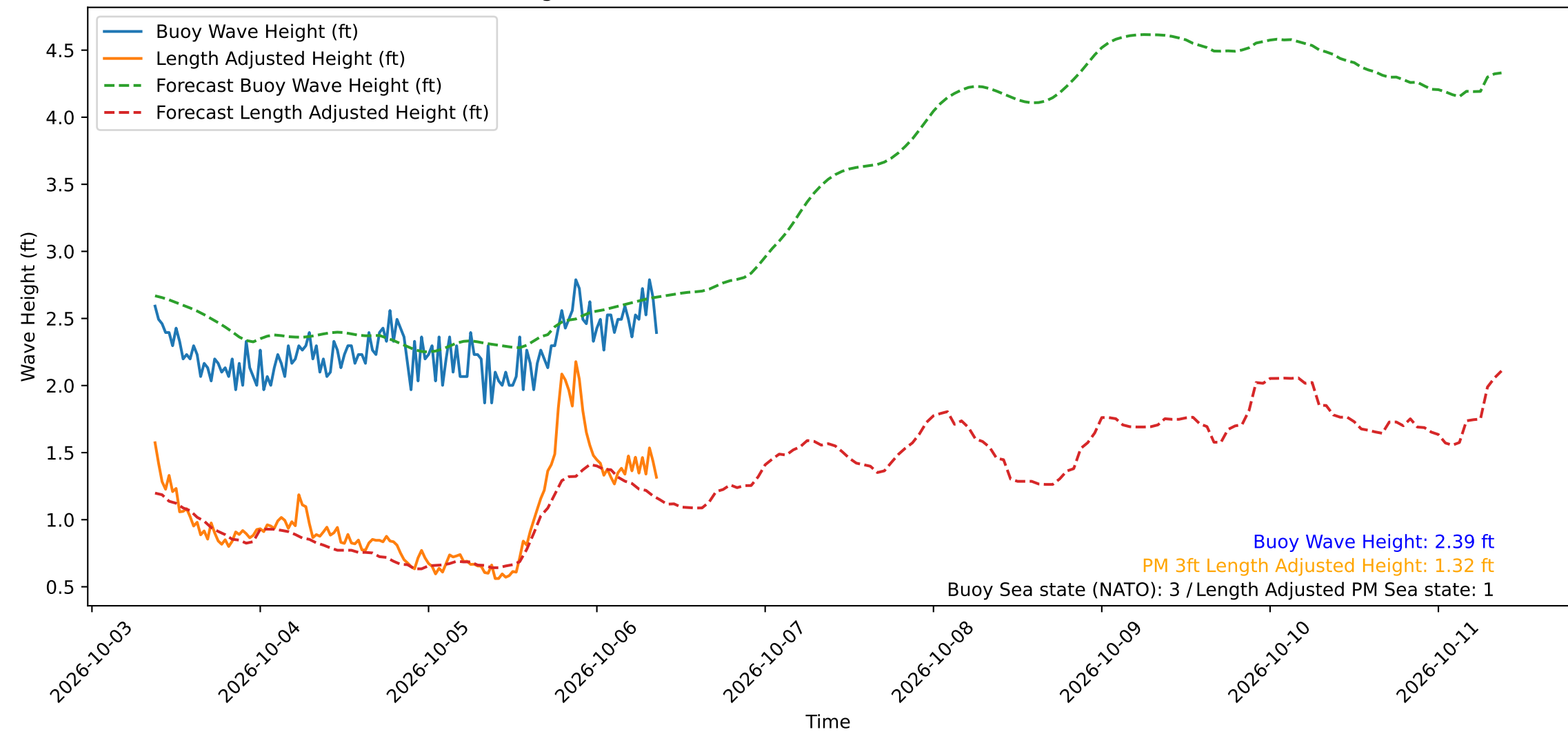
Wave Heights over Time for Oceanside Harbor at 2026-10-06 09:10:30
