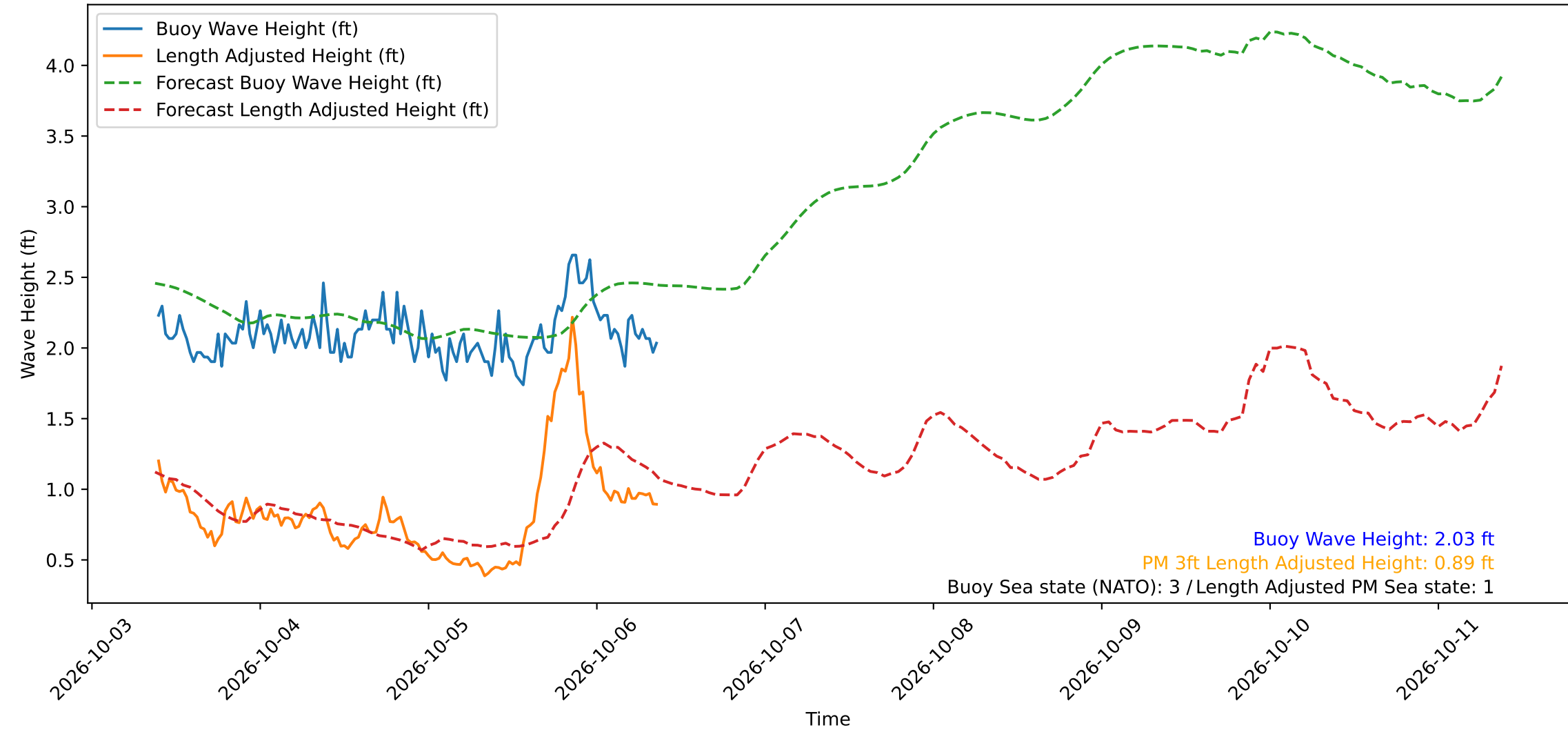
Wave Heights over Time for Red Beach at 2026-10-06 09:10:50
