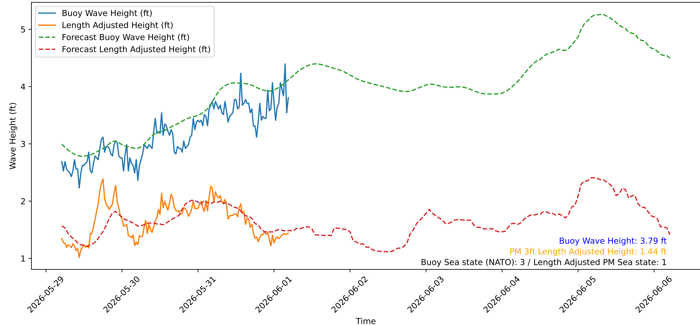
Wave Heights over Time for Oceanside Harbor at 2026-06-01 05:10:26
