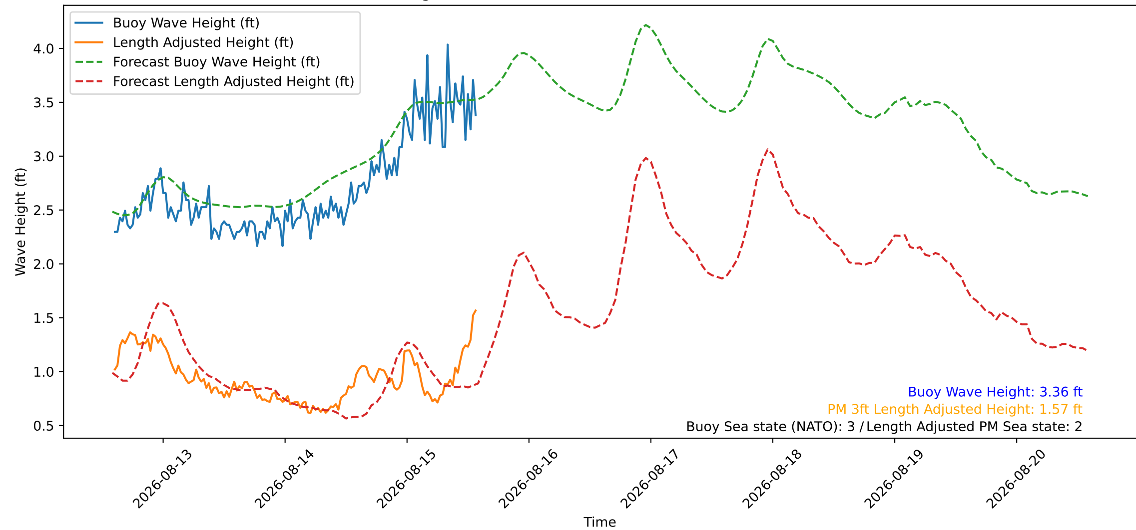
Wave Heights over Time for Red Beach at 2026-08-15 14:20:48
