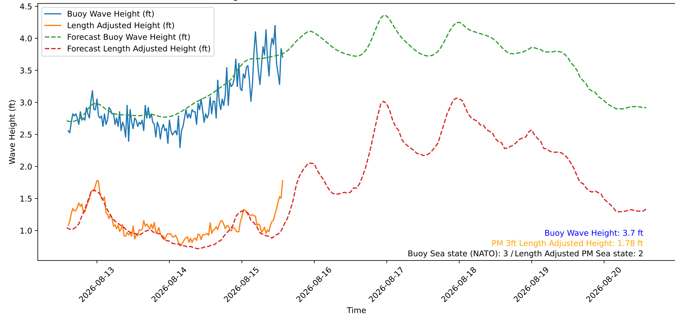
Wave Heights over Time for Oceanside Harbor at 2026-08-15 14:20:26
