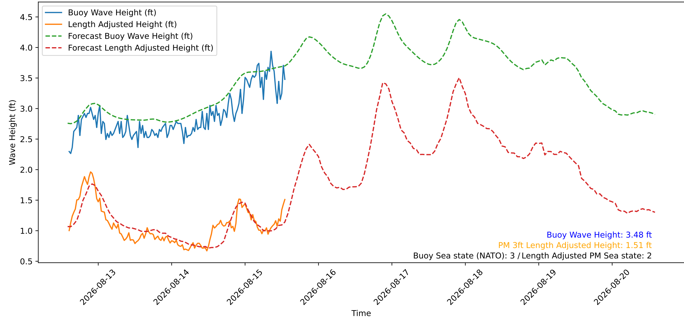
Wave Heights over Time for Green Beach at 2026-08-15 14:21:10
