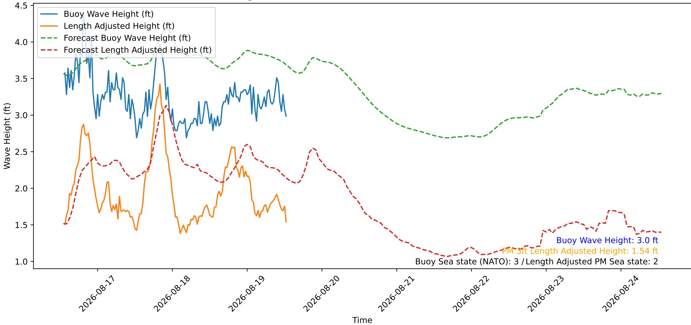
Wave Heights over Time for Green Beach at 2026-08-19 13:11:10
