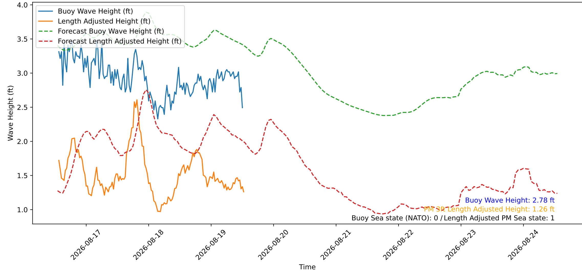
Wave Heights over Time for Red Beach at 2026-08-19 13:10:47
