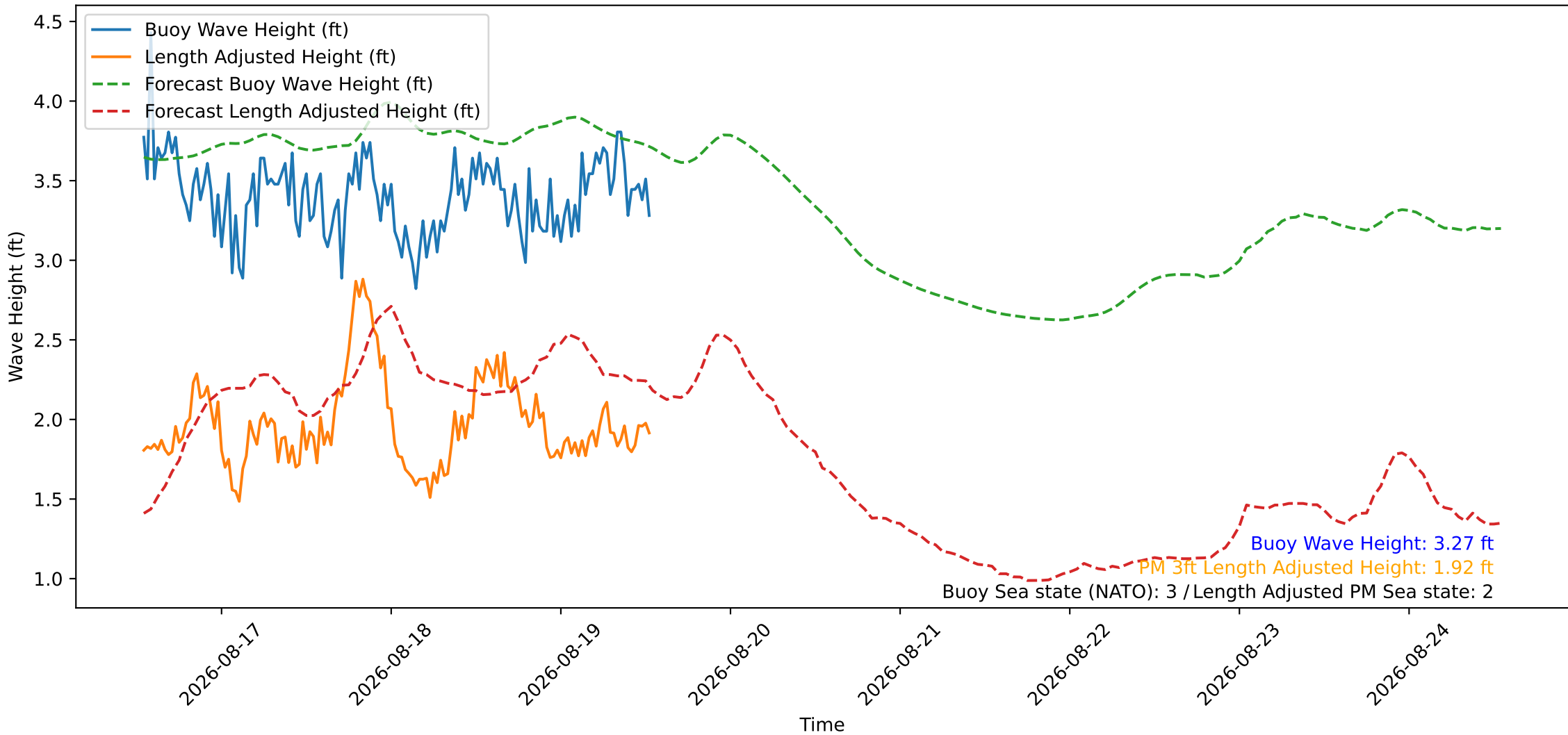
Wave Heights over Time for Oceanside Harbor at 2026-08-19 13:10:27
