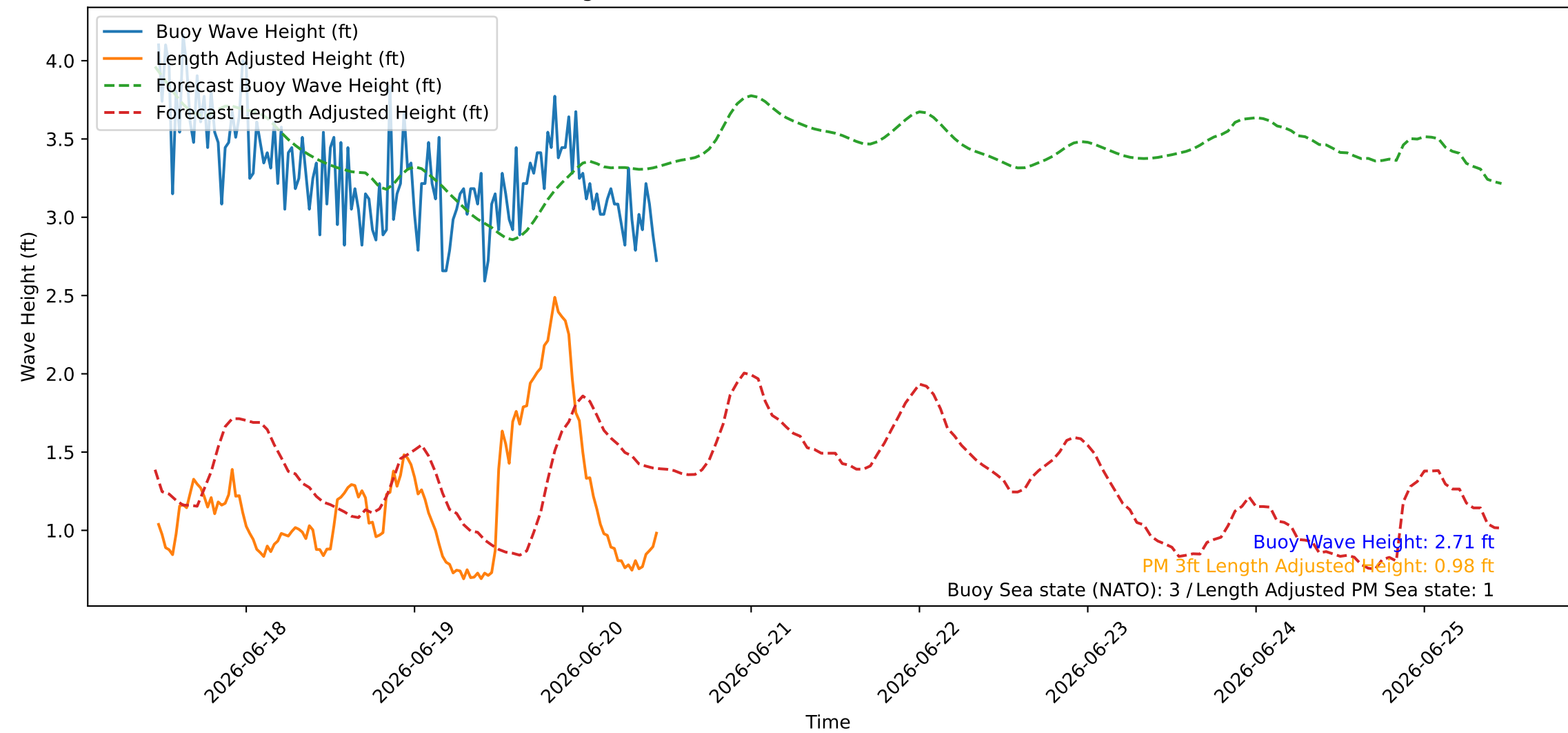
Wave Heights over Time for Red Beach at 2026-06-20 11:10:45
