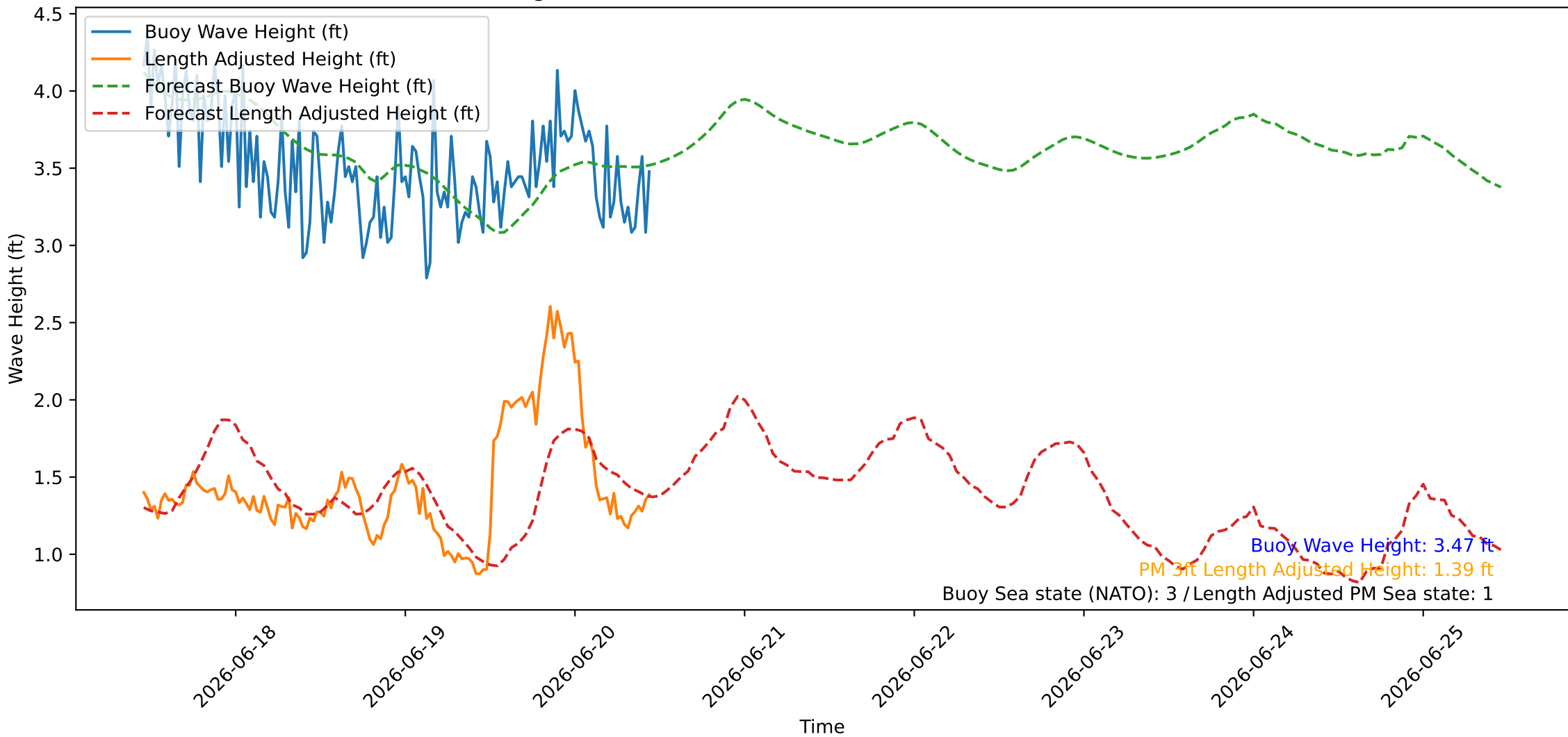
Wave Heights over Time for Oceanside Harbor at 2026-06-20 11:10:26
