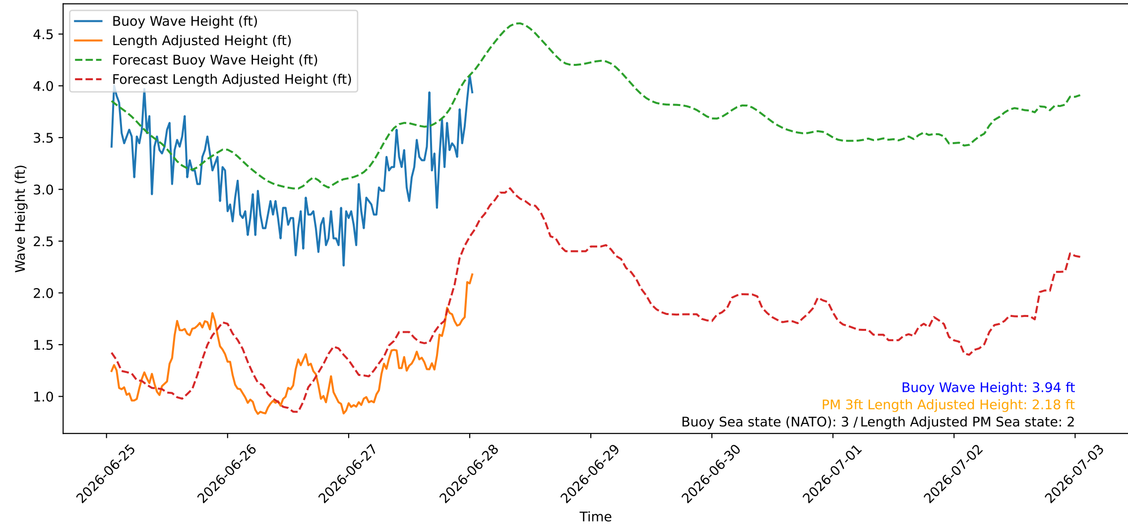
Wave Heights over Time for Green Beach at 2026-06-28 01:11:08
