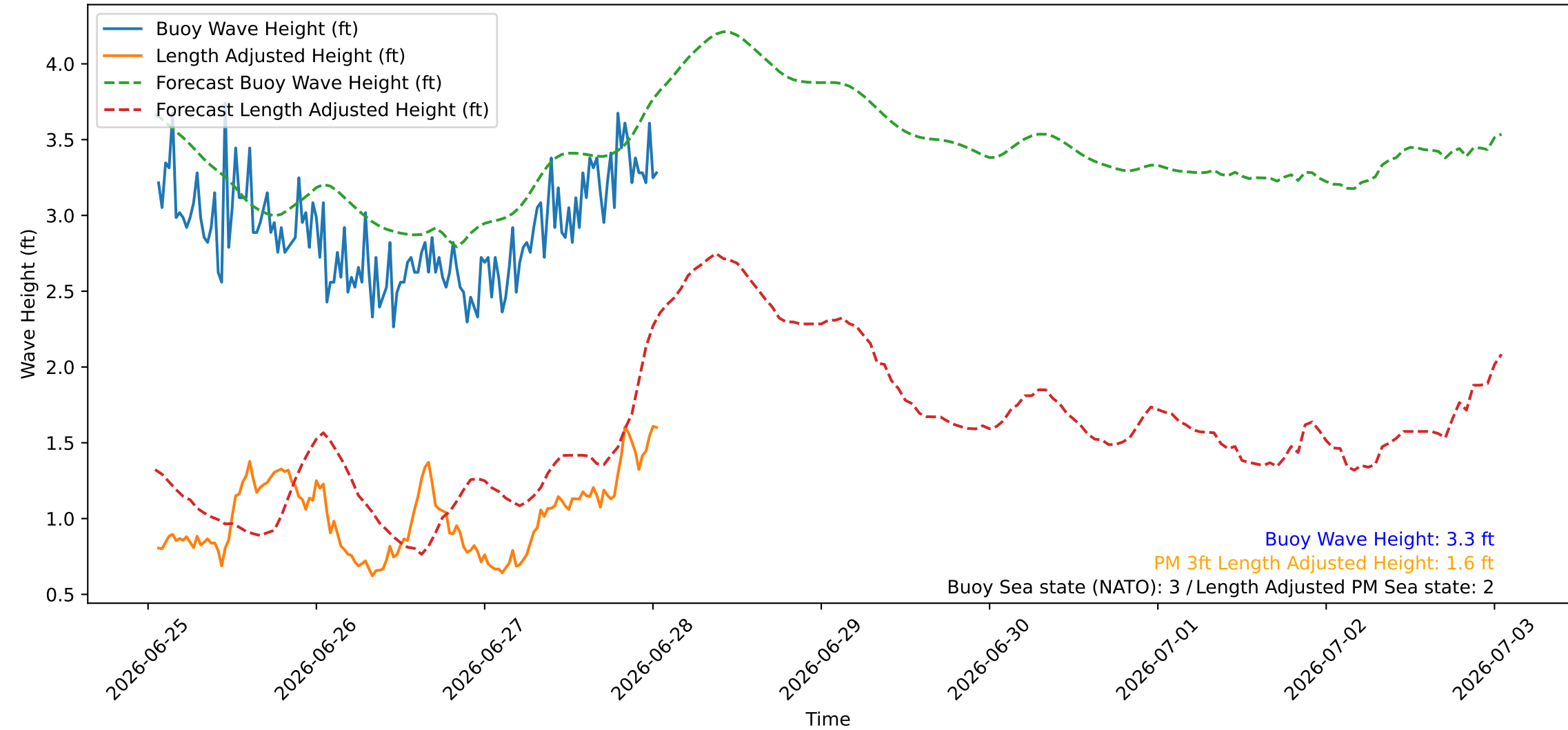
Wave Heights over Time for Red Beach at 2026-06-28 01:10:45
