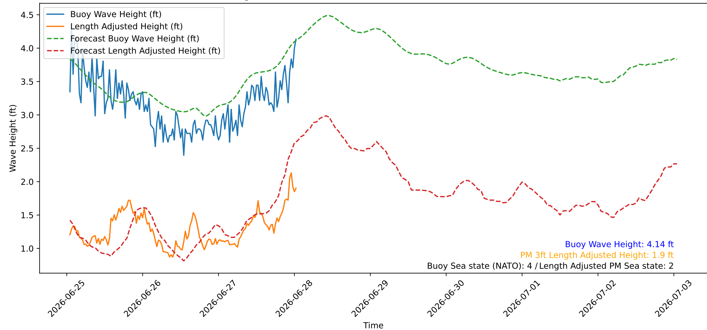
Wave Heights over Time for Oceanside Harbor at 2026-06-28 01:10:27
