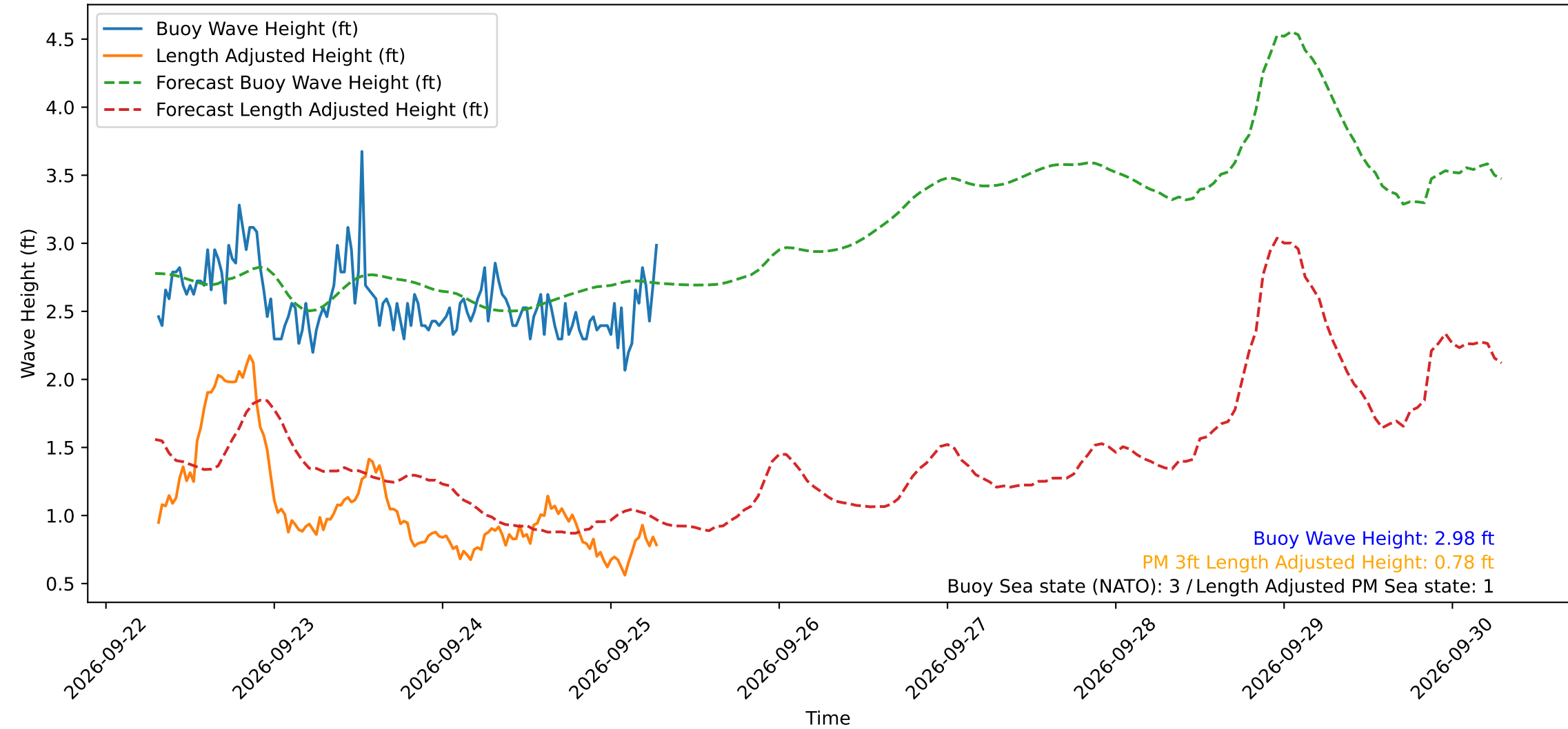
Wave Heights over Time for Red Beach at 2026-09-25 07:20:50
