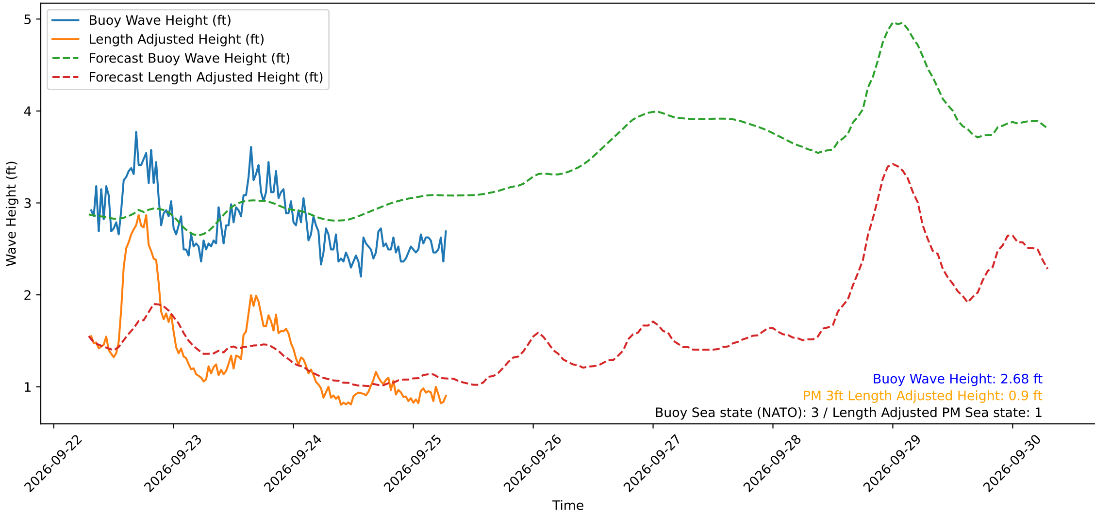
Wave Heights over Time for Oceanside Harbor at 2026-09-25 07:20:29
