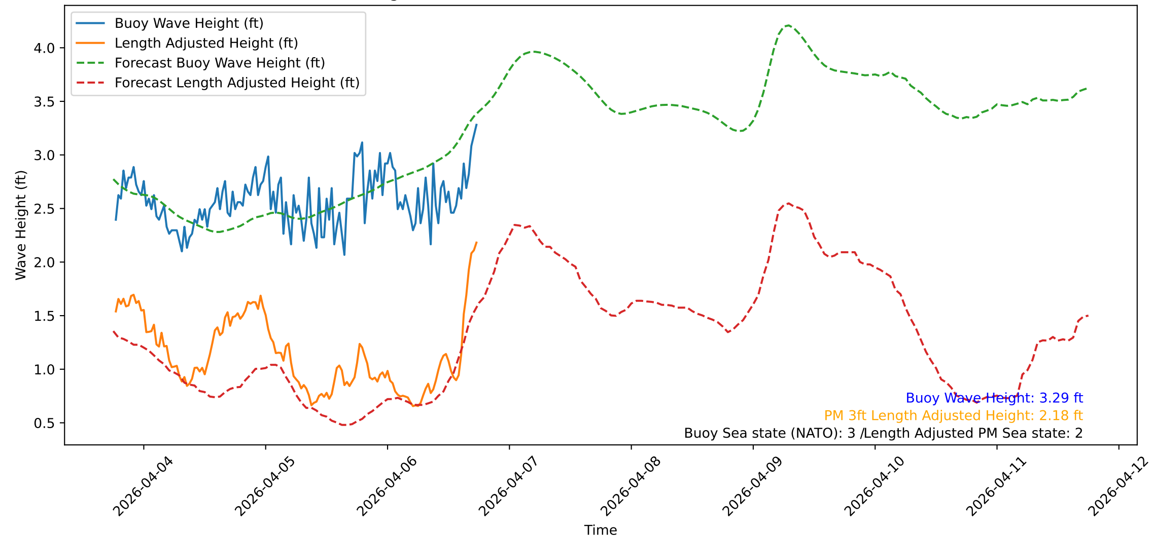
Wave Heights over Time for Oceanside Harbor at 2026-04-06 18:20:31
