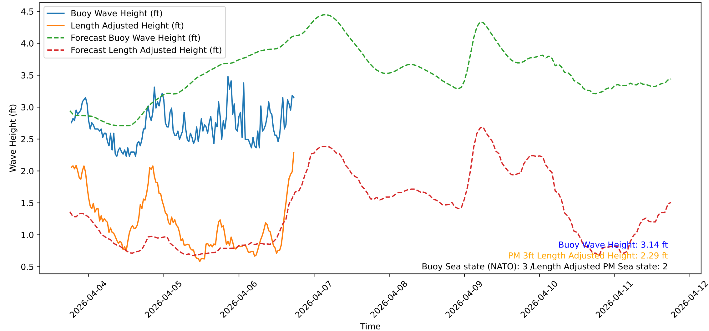
Wave Heights over Time for Green Beach at 2026-04-06 18:21:10
