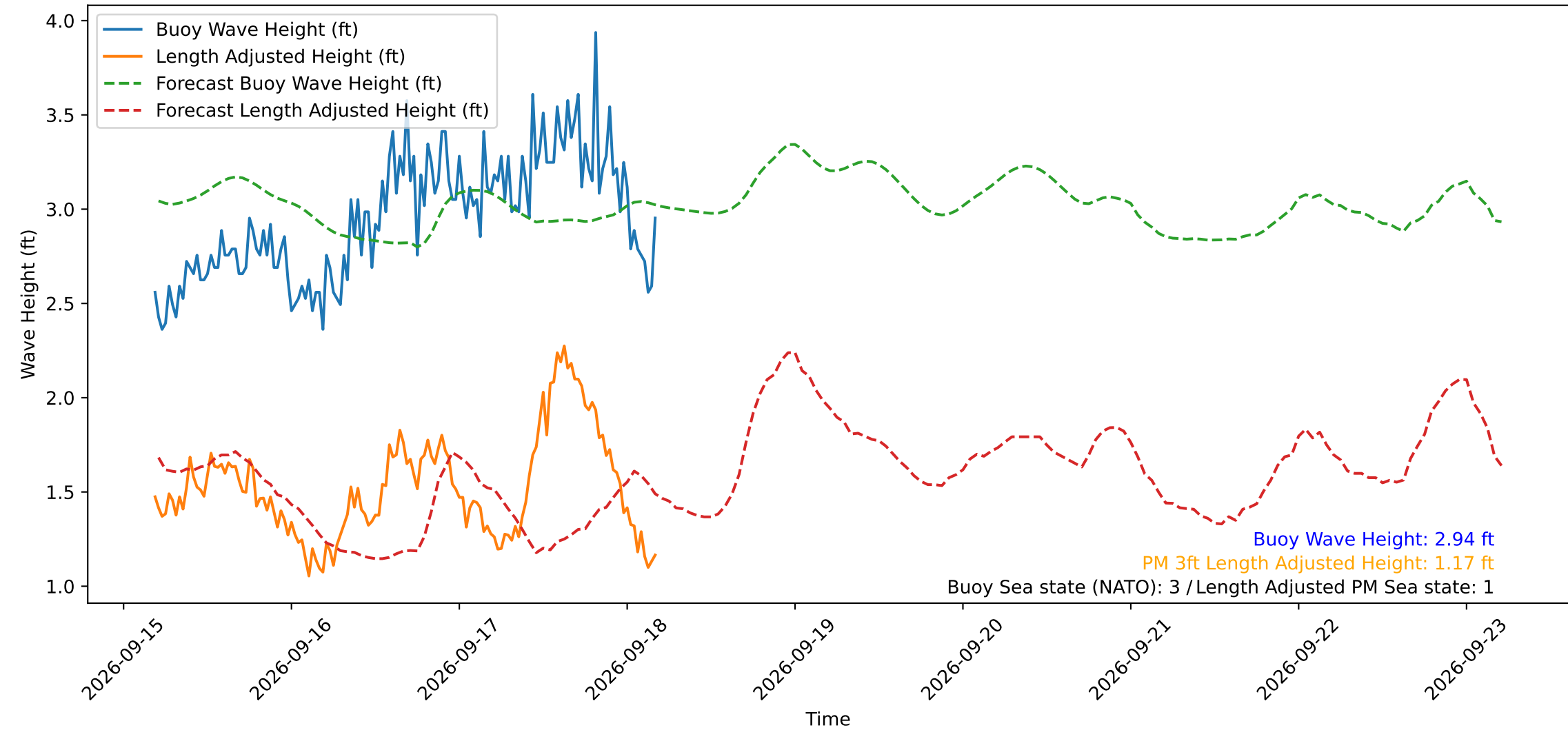
Wave Heights over Time for Oceanside Harbor at 2026-09-18 04:30:29
