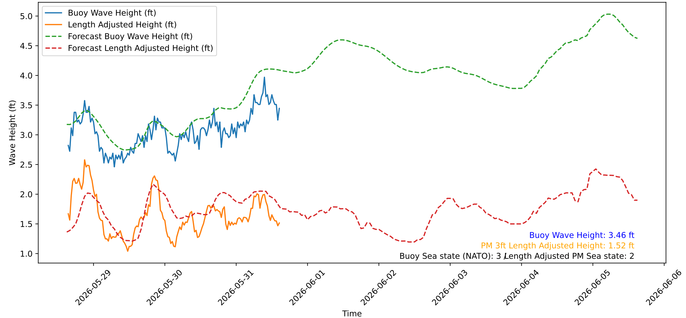
Wave Heights over Time for Green Beach at 2026-05-31 15:21:09
