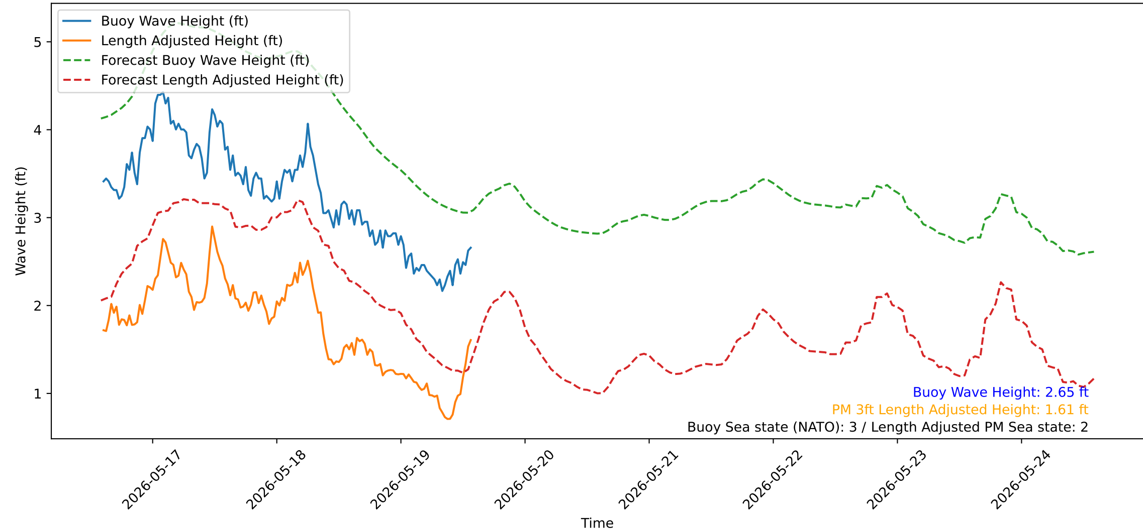
Wave Heights over Time for Green Beach at 2026-05-19 14:21:15
