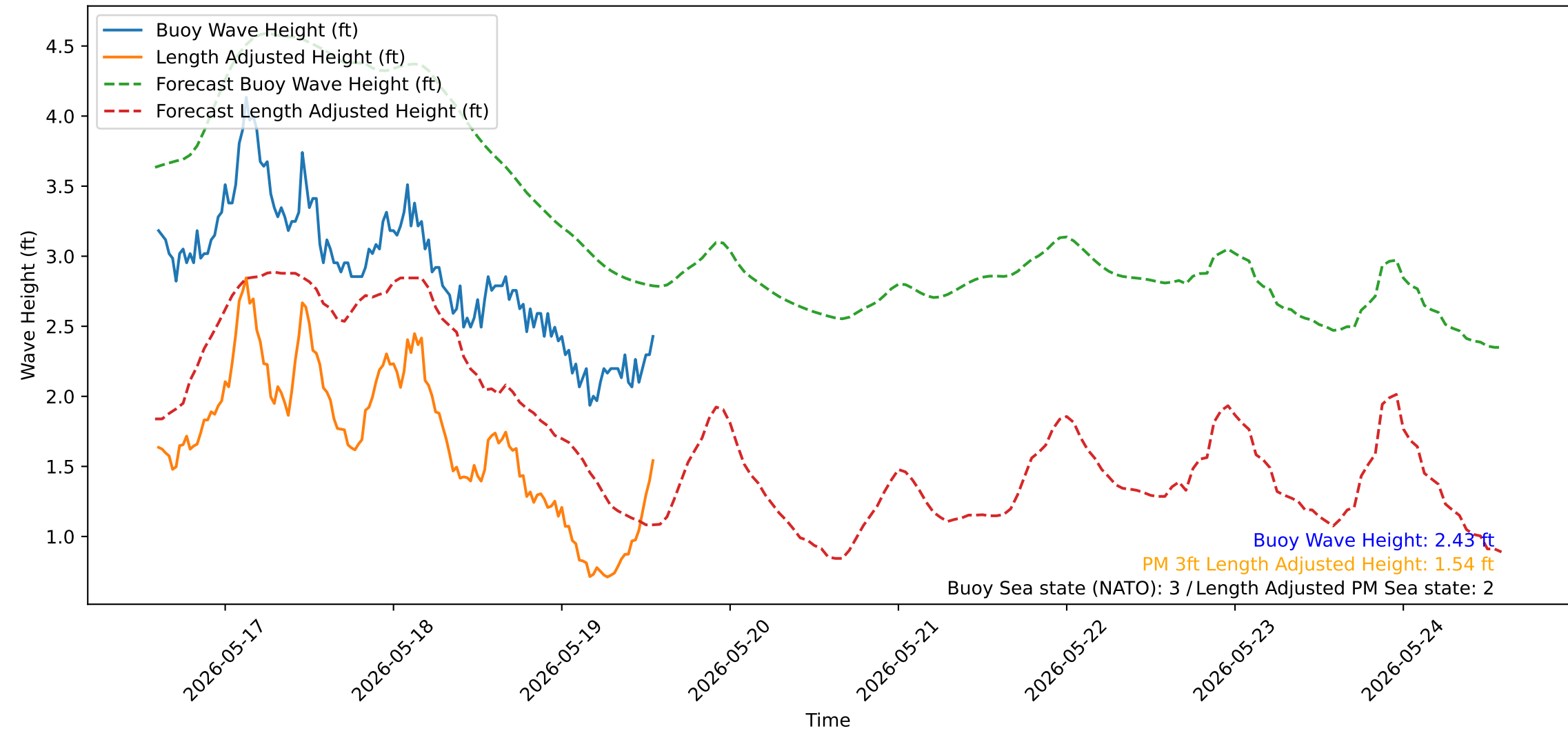
Wave Heights over Time for Red Beach at 2026-05-19 14:20:52
