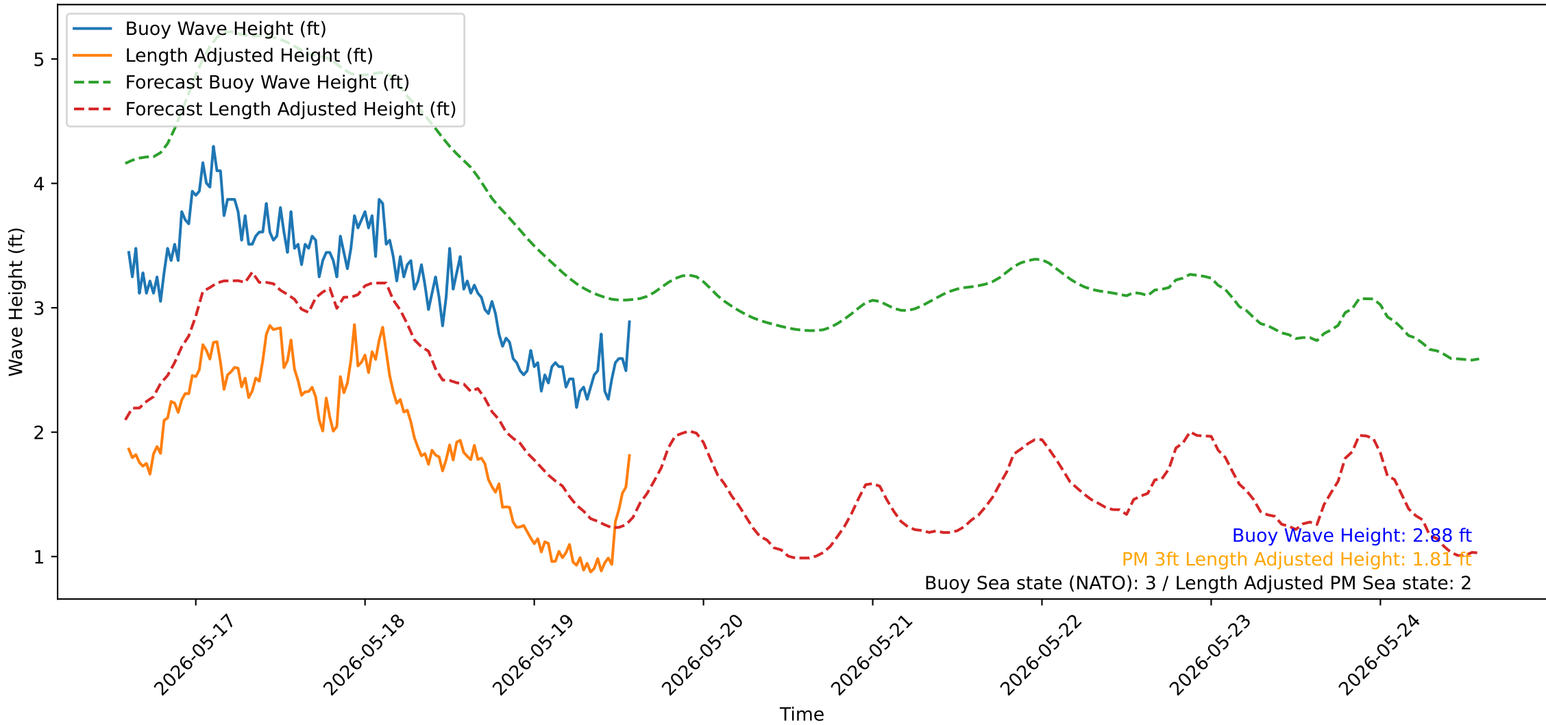
Wave Heights over Time for Oceanside Harbor at 2026-05-19 14:20:32
