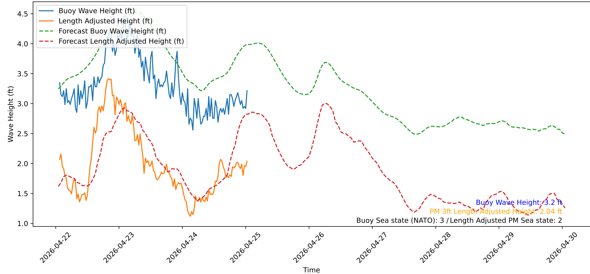
Wave Heights over Time for Oceanside Harbor at 2026-04-25 01:20:31
