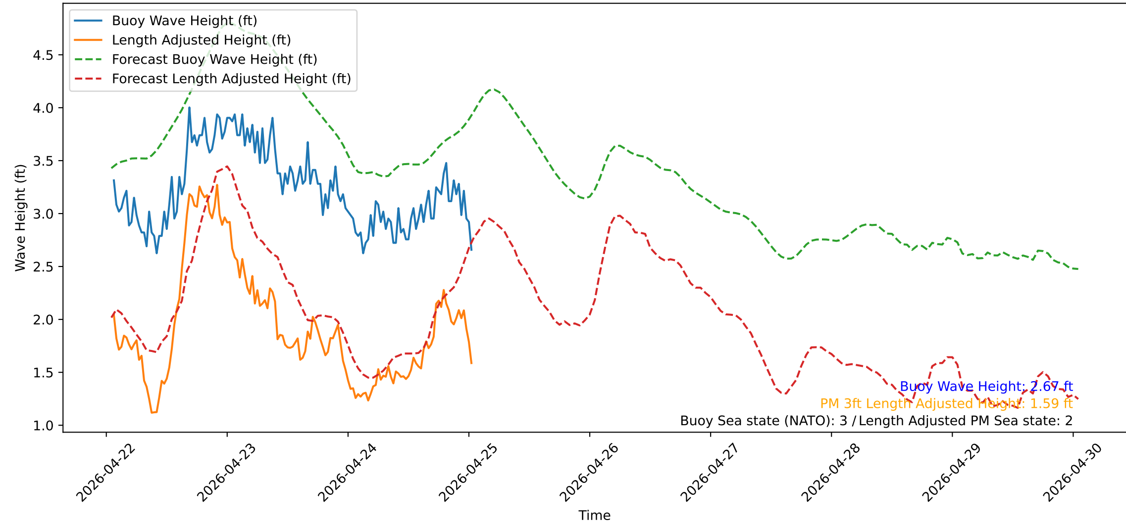
Wave Heights over Time for Green Beach at 2026-04-25 01:21:14
