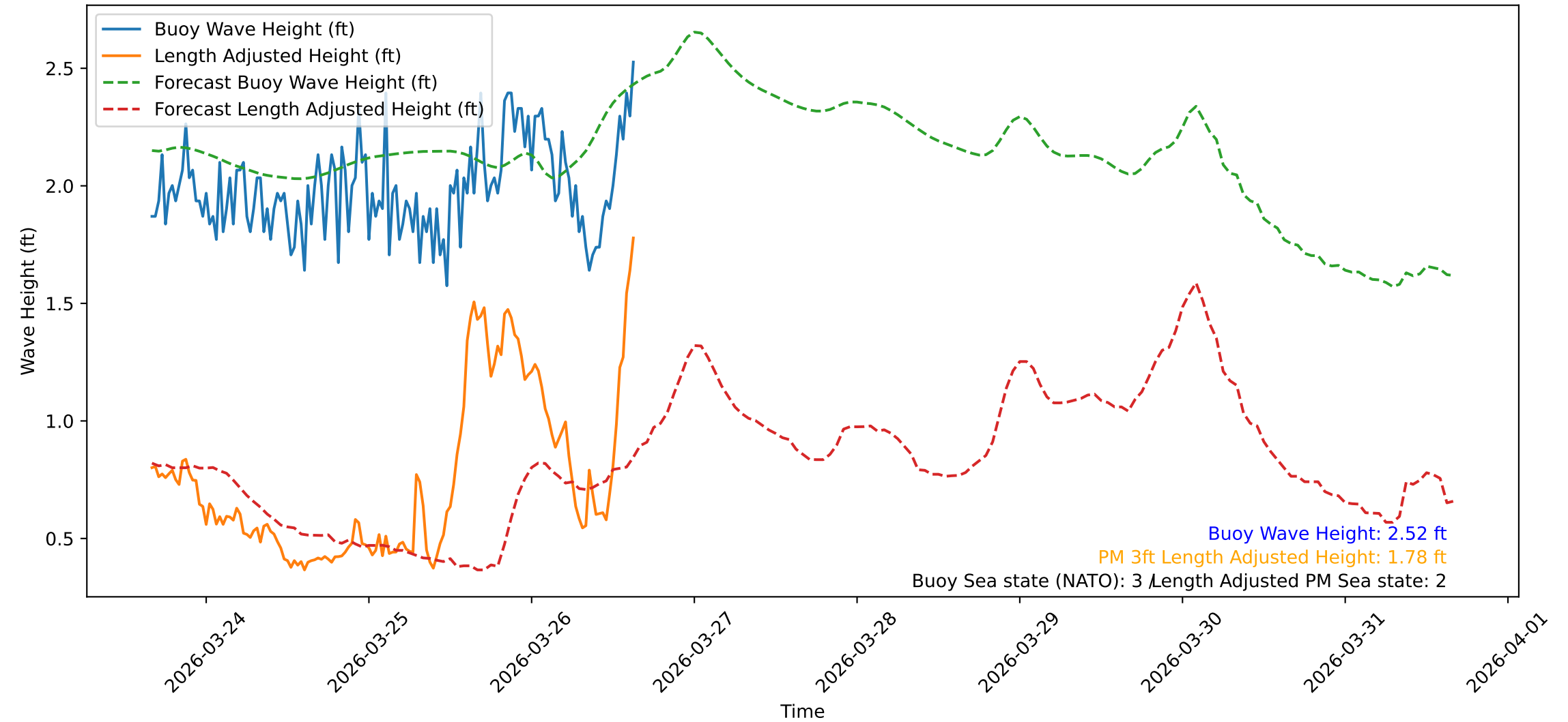
Wave Heights over Time for Red Beach at 2026-03-26 15:50:48
