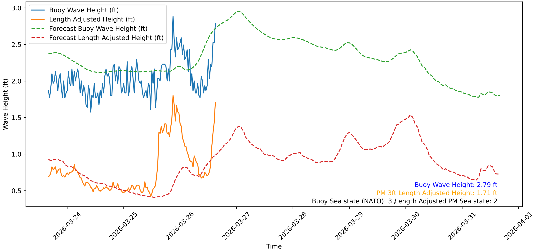
Wave Heights over Time for Oceanside Harbor at 2026-03-26 15:50:32
