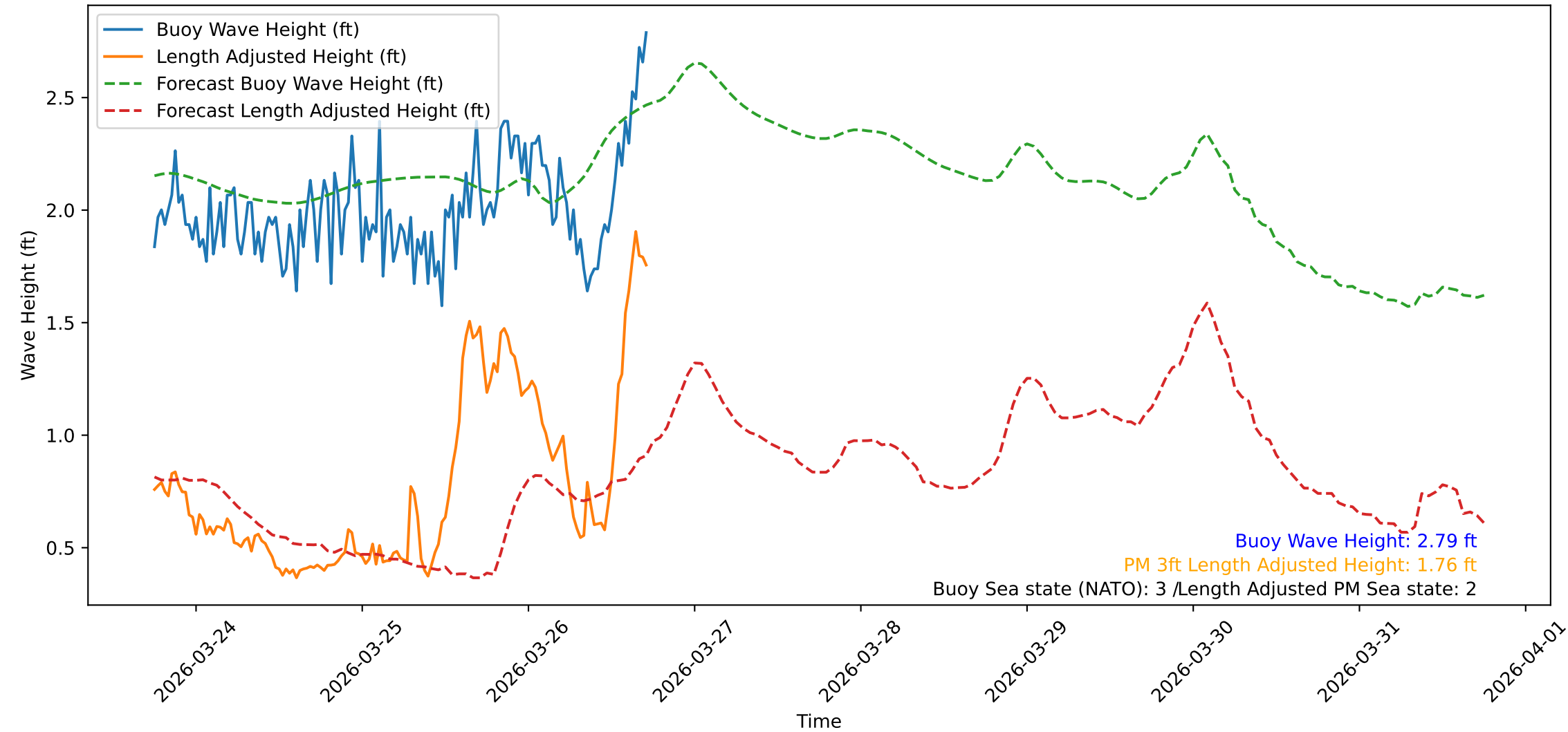
Wave Heights over Time for Red Beach at 2026-03-26 17:40:47
