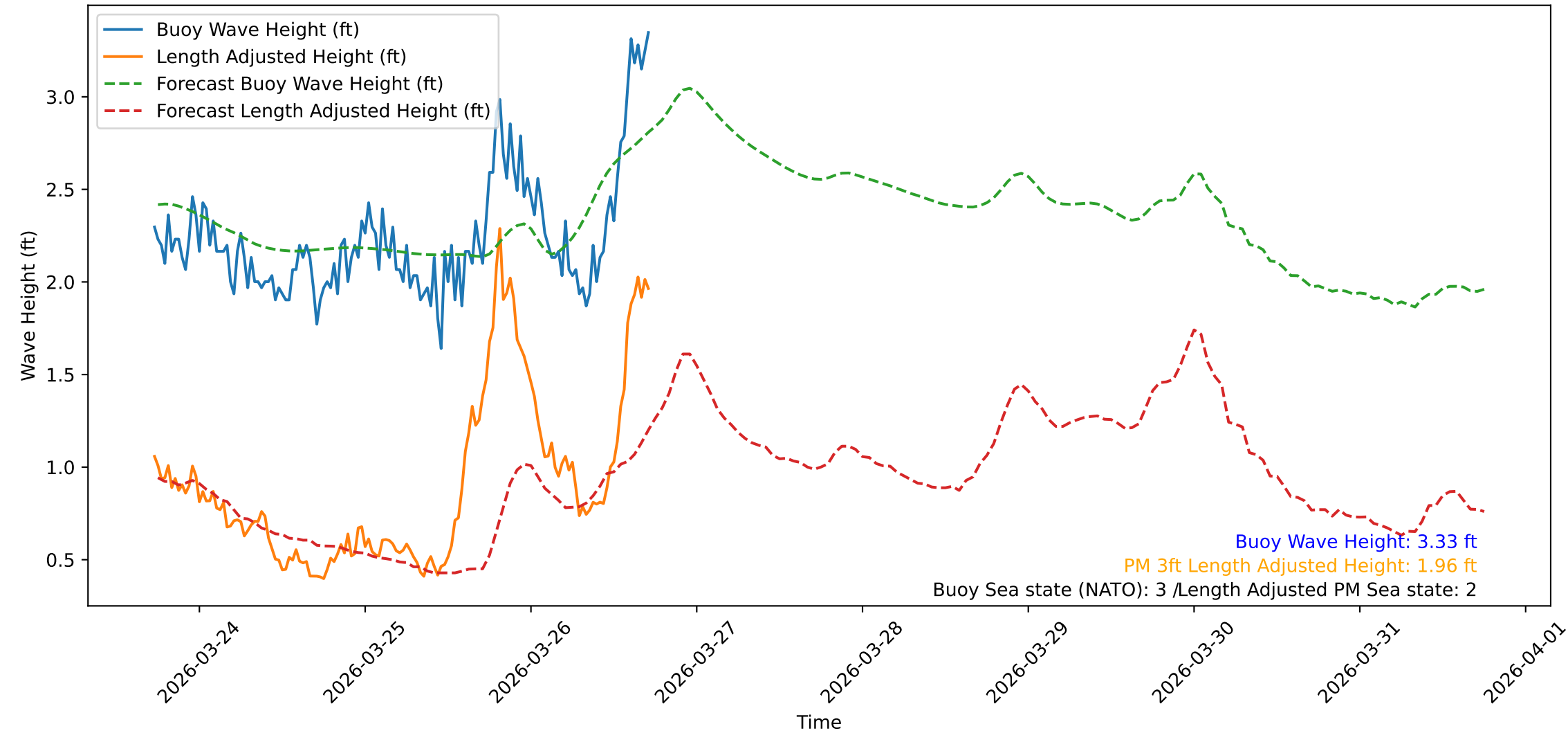
Wave Heights over Time for Green Beach at 2026-03-26 17:41:09
