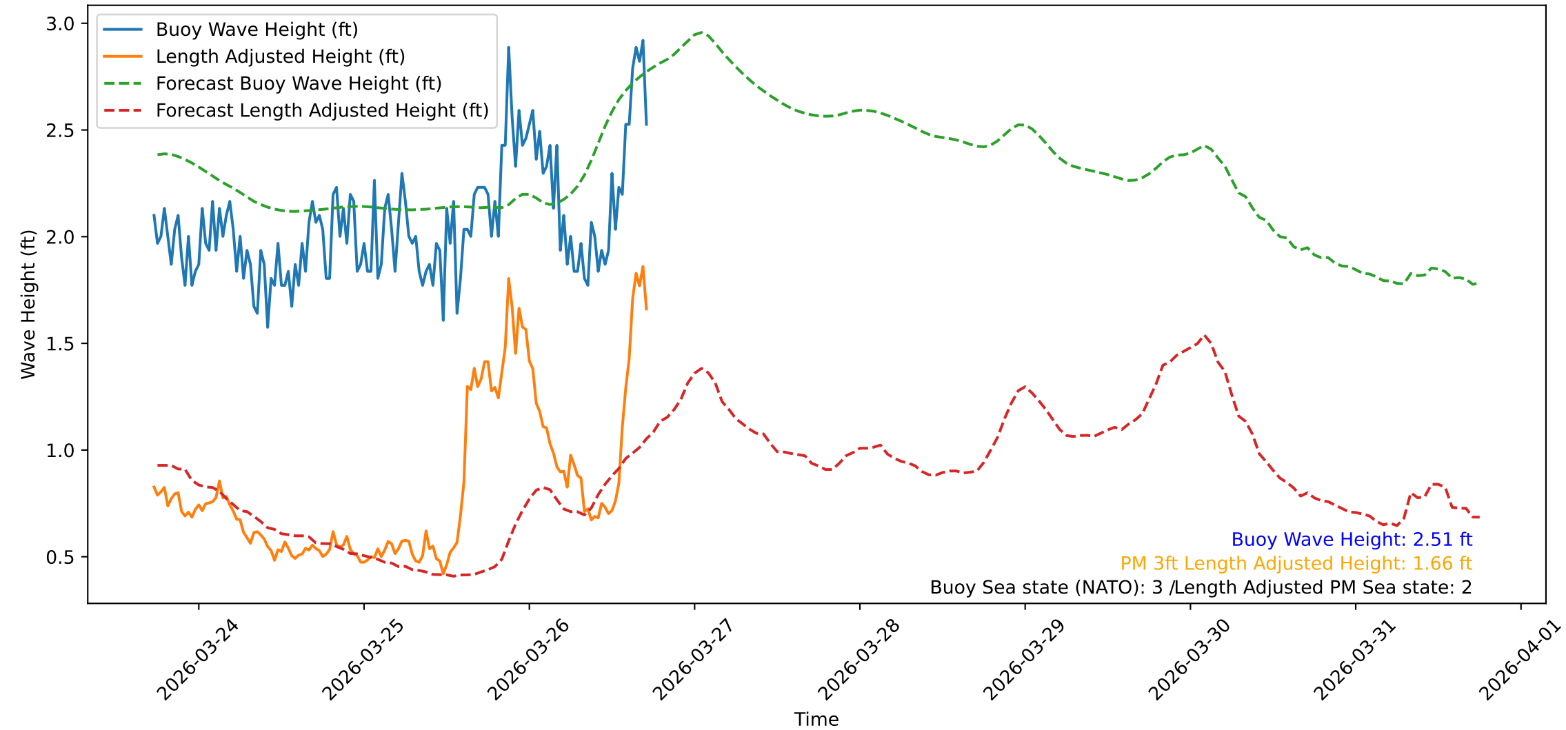
Wave Heights over Time for Oceanside Harbor at 2026-03-26 17:40:32
