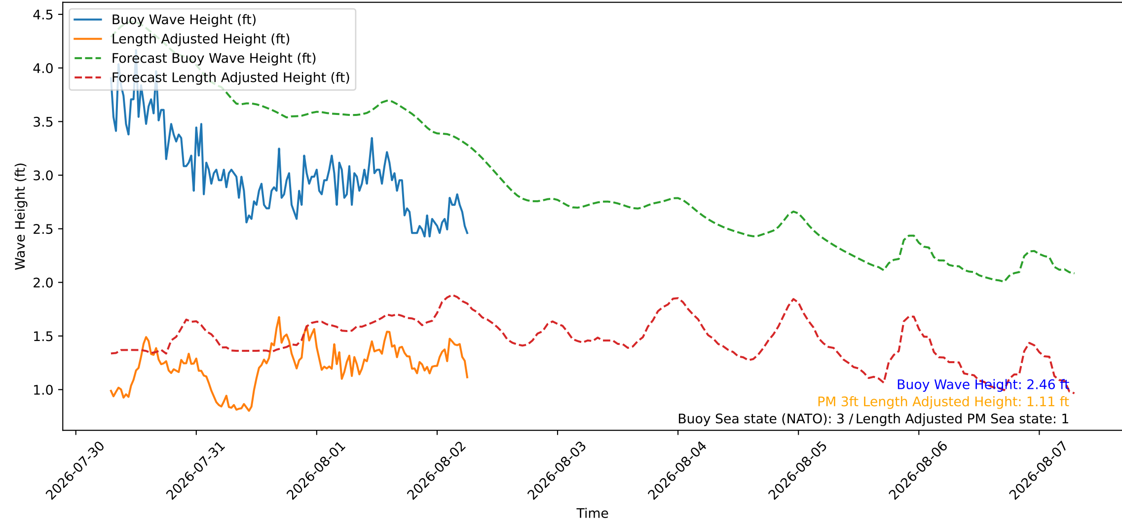
Wave Heights over Time for Red Beach at 2026-08-02 06:40:46
