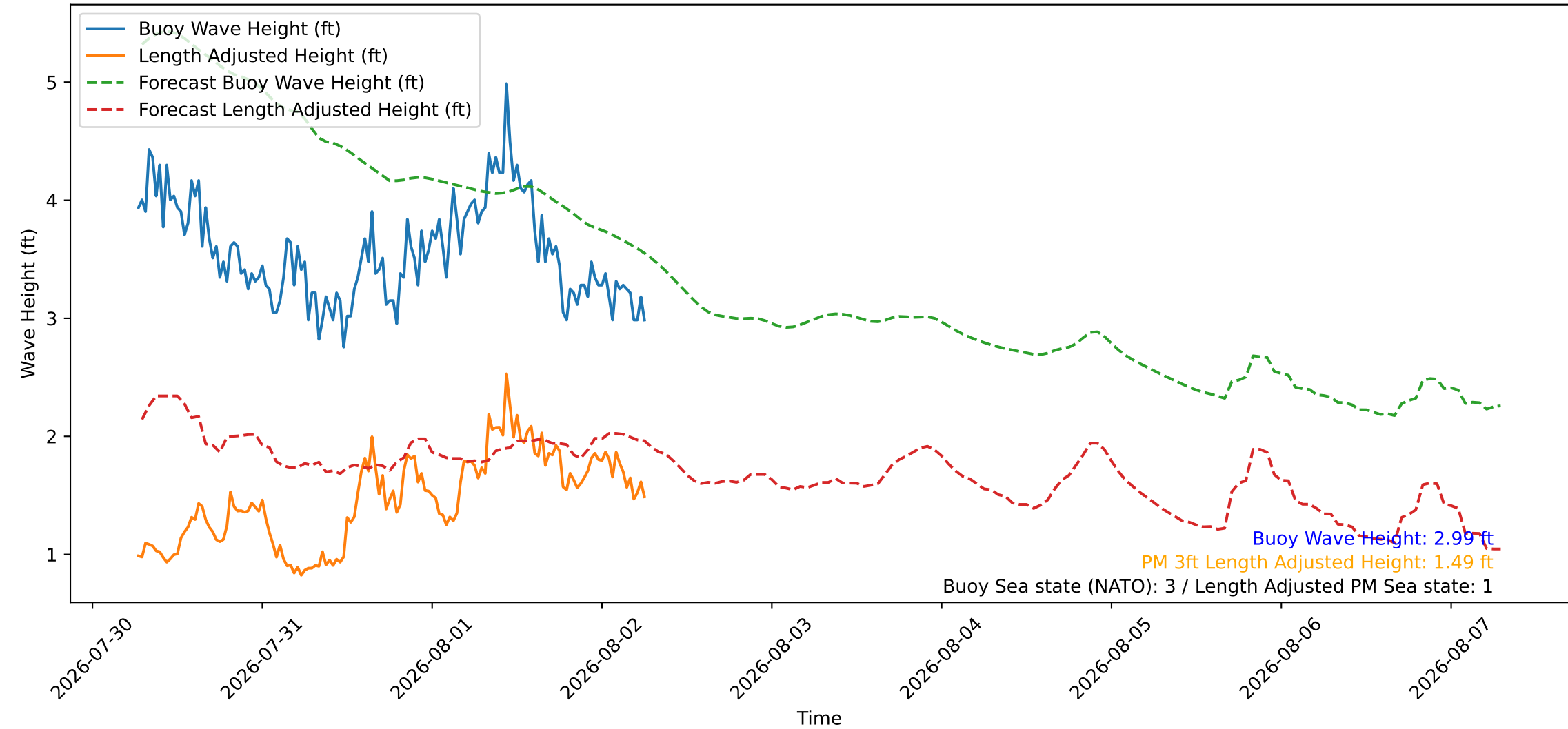
Wave Heights over Time for Green Beach at 2026-08-02 06:41:08
