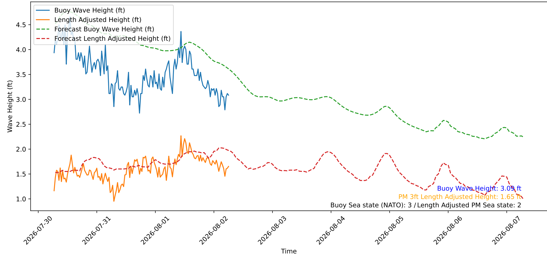
Wave Heights over Time for Oceanside Harbor at 2026-08-02 06:40:26
