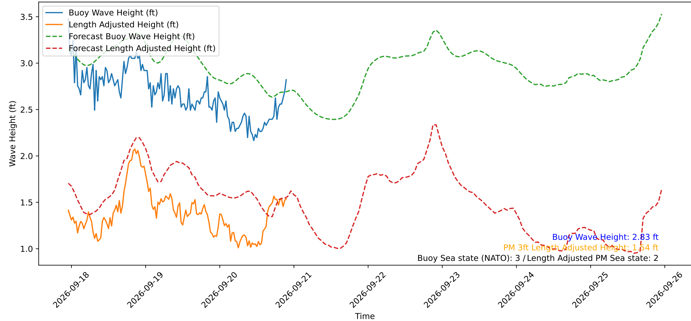
Wave Heights over Time for Green Beach at 2026-09-20 22:31:11
