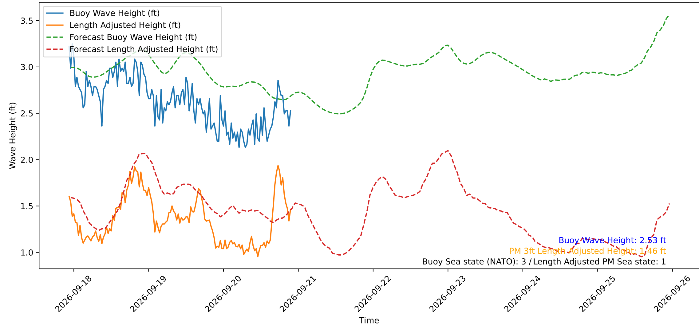
Wave Heights over Time for Oceanside Harbor at 2026-09-20 22:30:29
