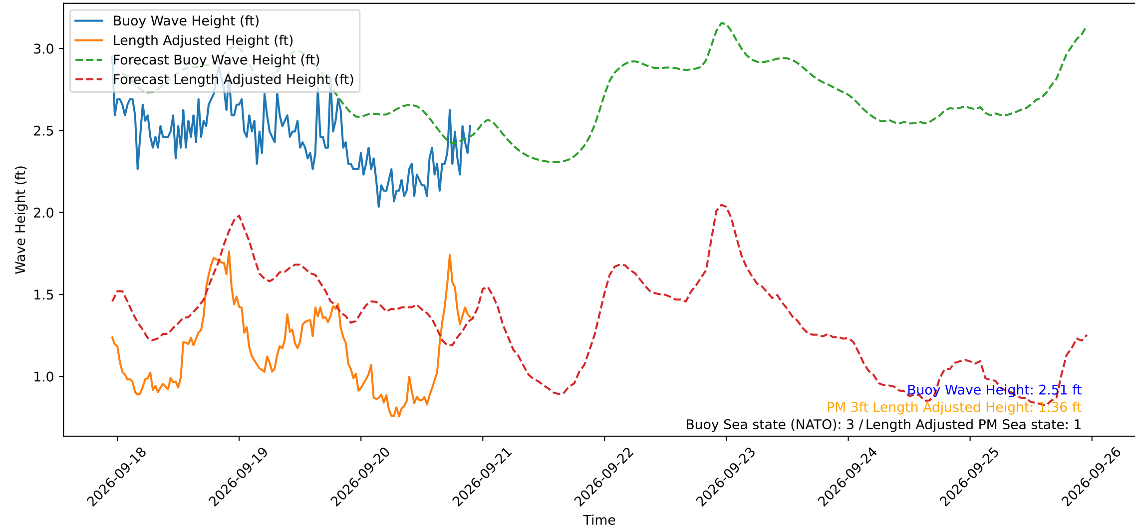
Wave Heights over Time for Red Beach at 2026-09-20 22:30:48
