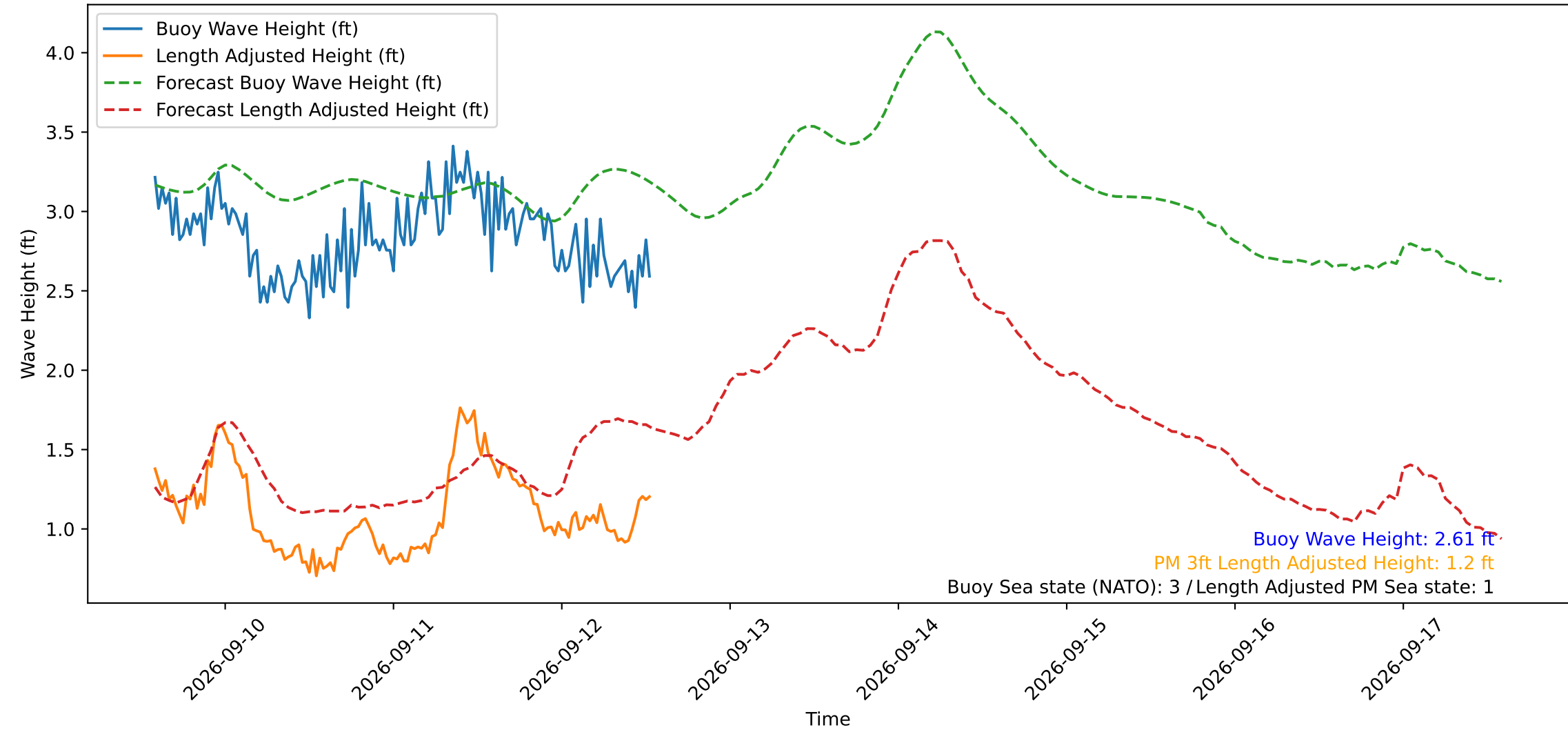
Wave Heights over Time for Red Beach at 2026-09-12 13:50:50
