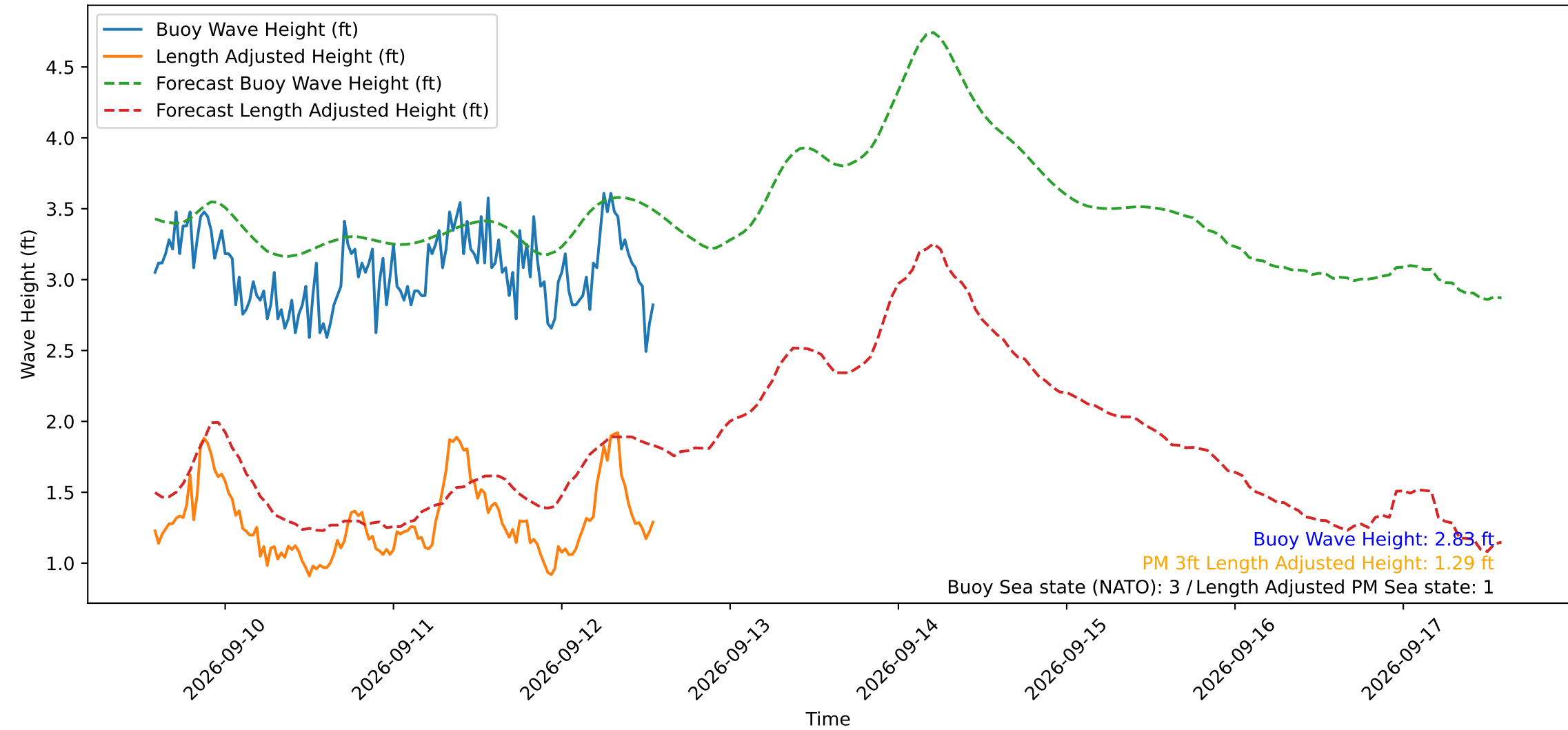
Wave Heights over Time for Green Beach at 2026-09-12 13:51:13
