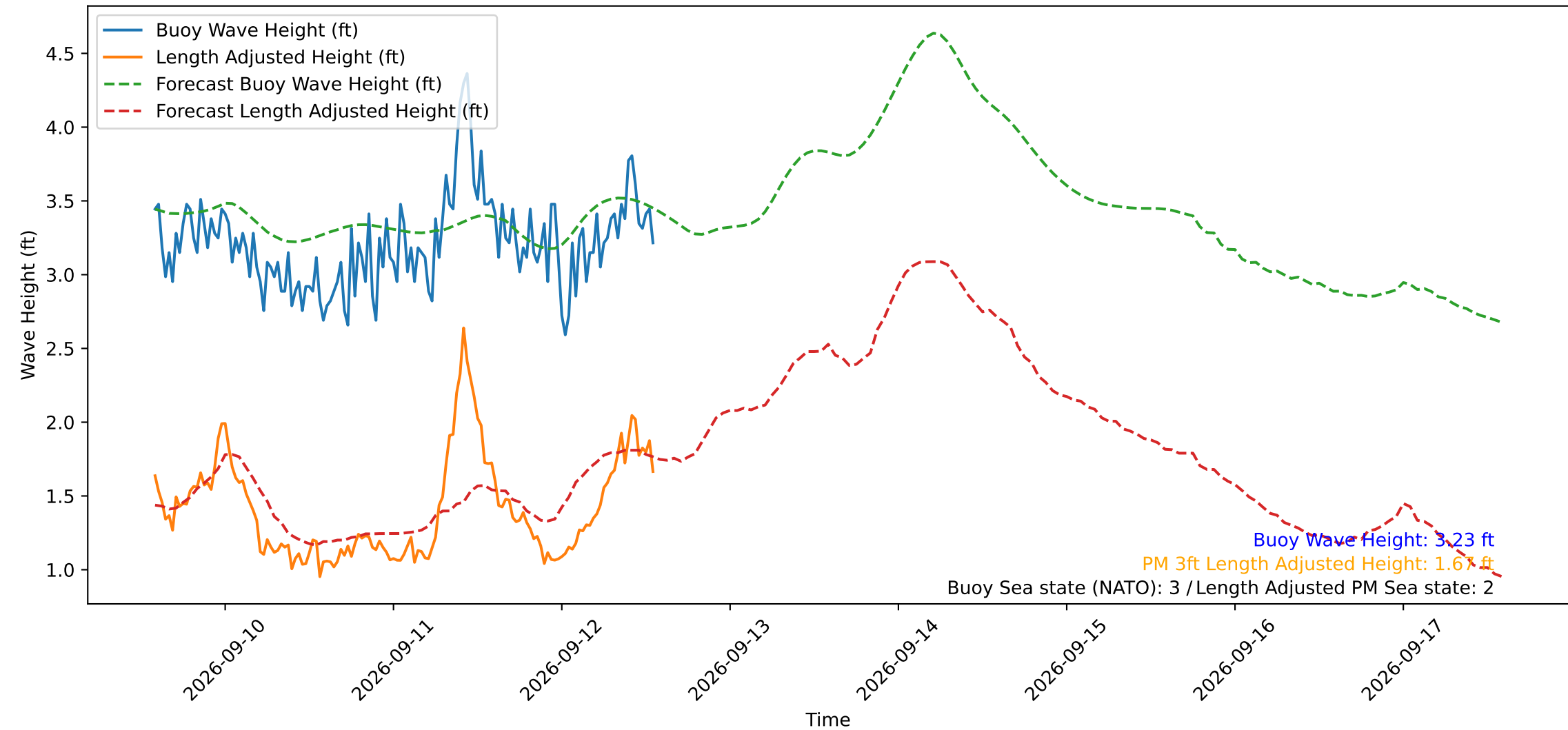
Wave Heights over Time for Oceanside Harbor at 2026-09-12 13:50:29
