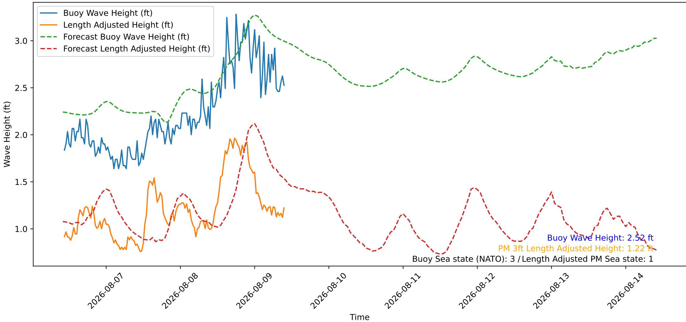
Wave Heights over Time for Oceanside Harbor at 2026-08-09 10:20:26
