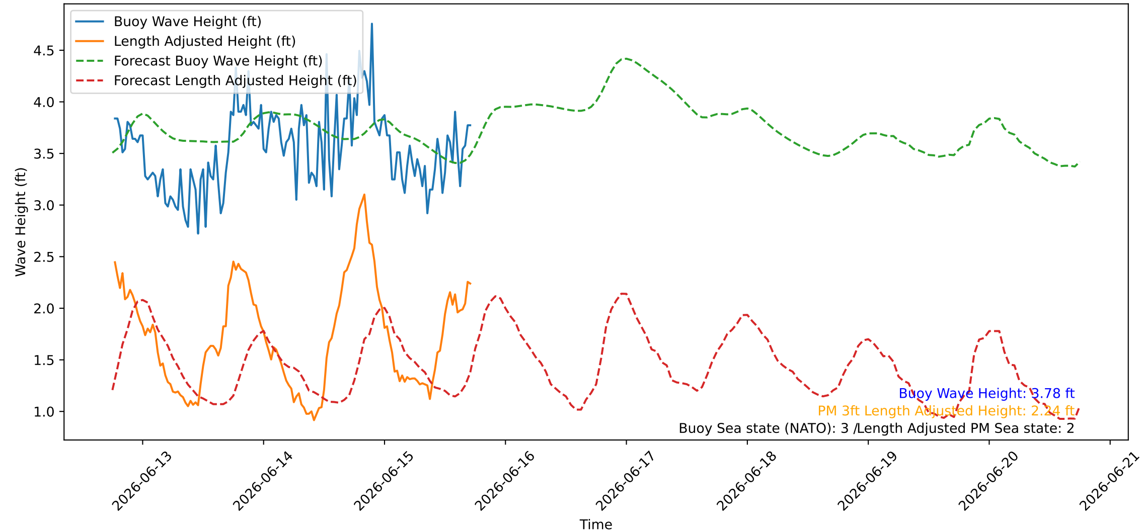
Wave Heights over Time for Red Beach at 2026-06-15 18:00:45
