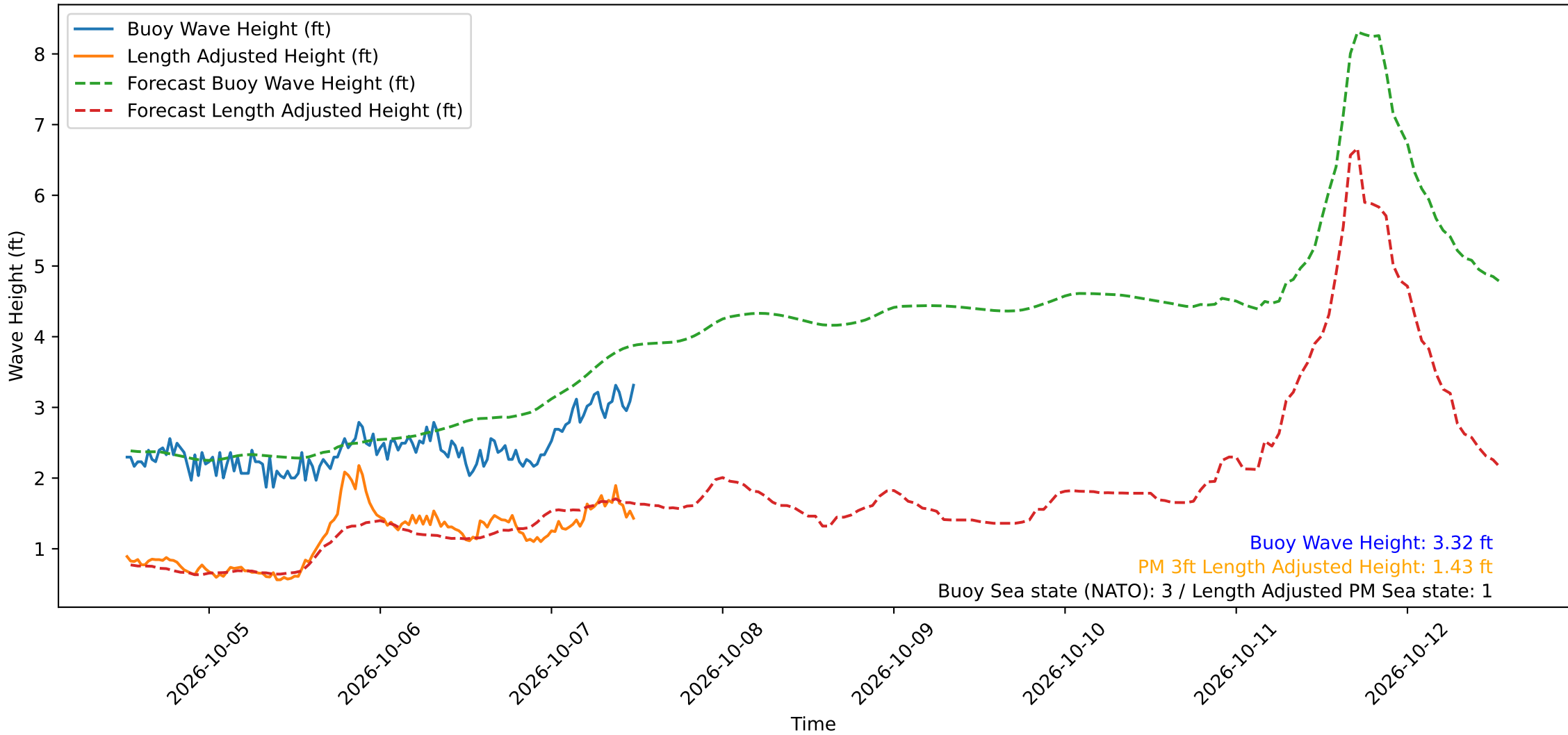
Wave Heights over Time for Oceanside Harbor at 2026-10-07 12:30:31
