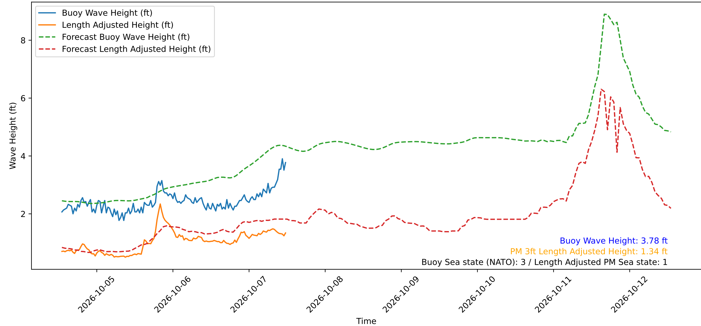
Wave Heights over Time for Green Beach at 2026-10-07 12:31:14
