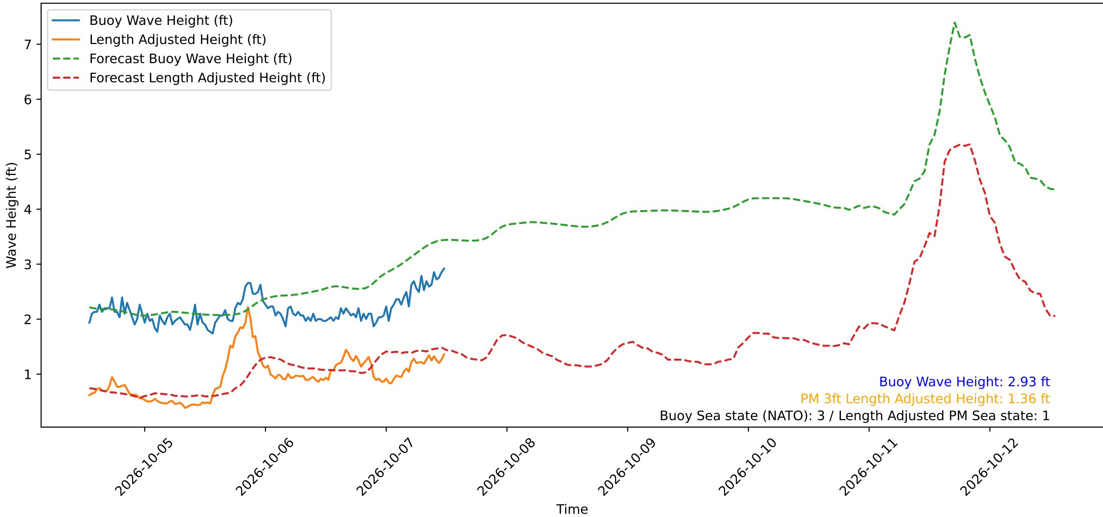
Wave Heights over Time for Red Beach at 2026-10-07 12:30:50
