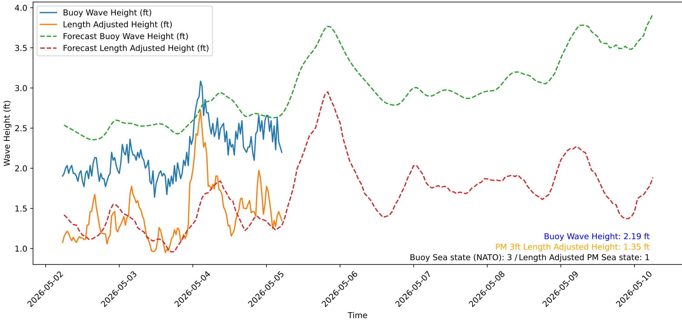
Wave Heights over Time for Oceanside Harbor at 2026-05-05 05:30:32
