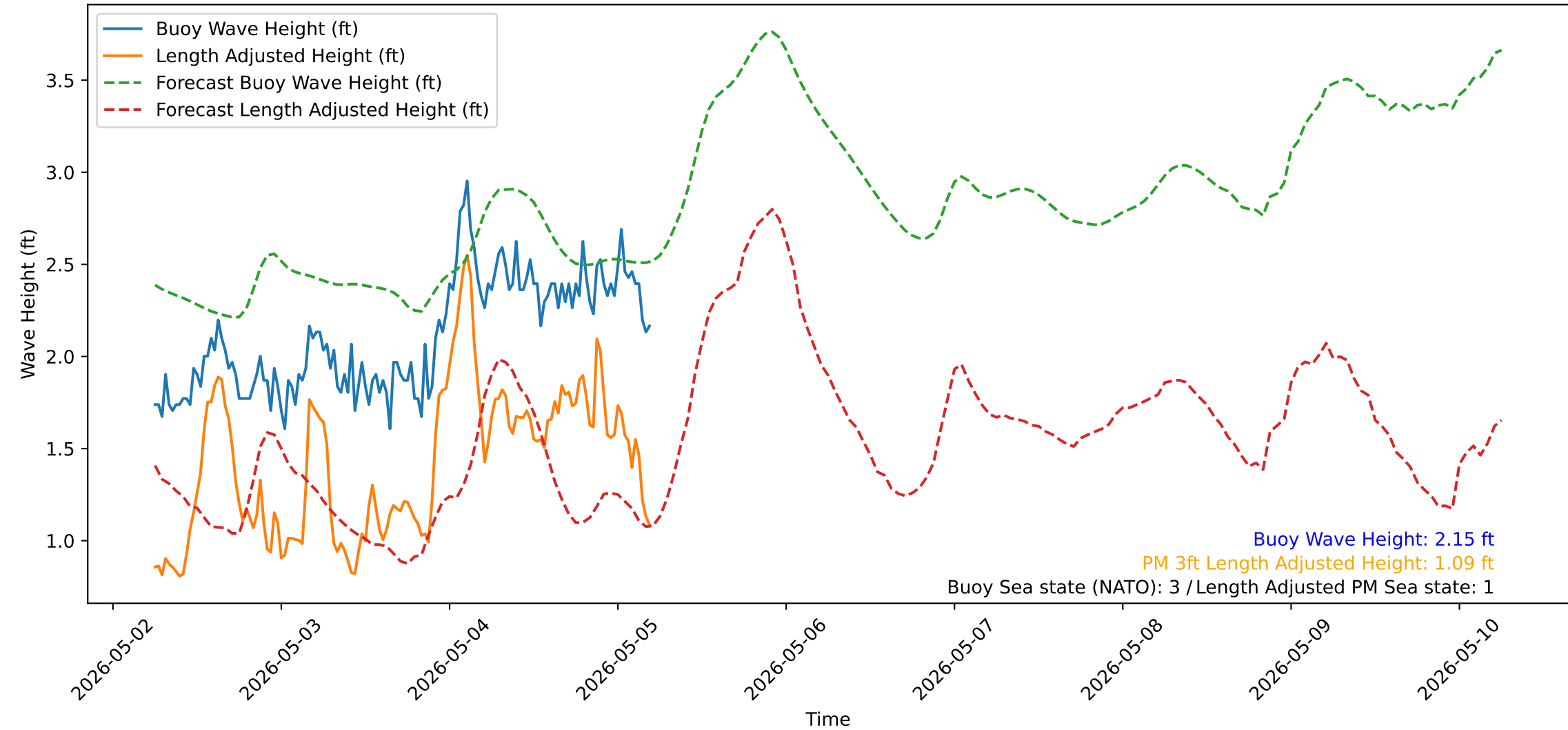
Wave Heights over Time for Red Beach at 2026-05-05 05:30:51
