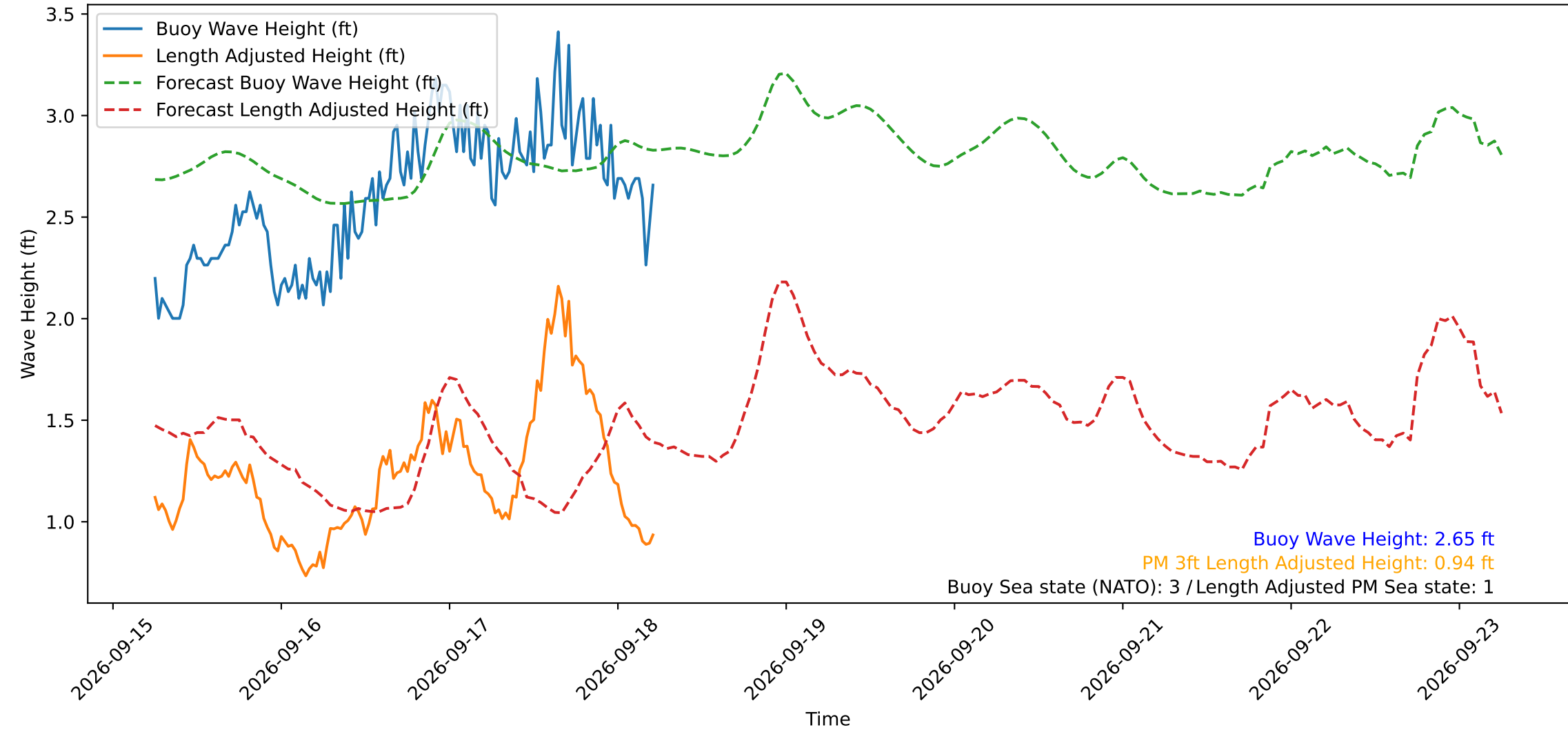
Wave Heights over Time for Red Beach at 2026-09-18 05:40:49
