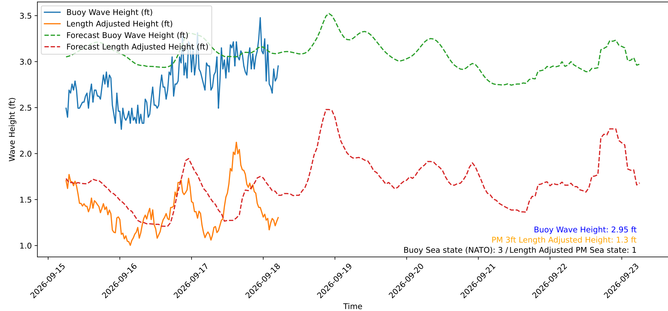
Wave Heights over Time for Green Beach at 2026-09-18 05:41:11
