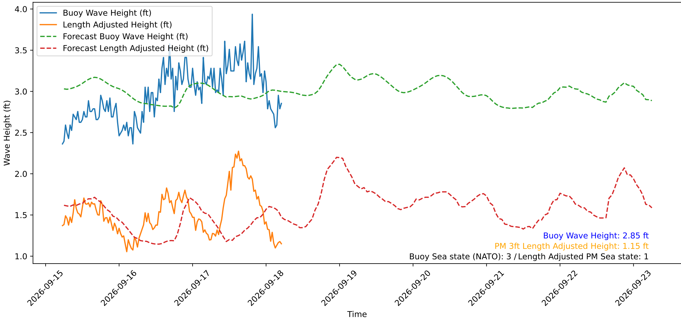
Wave Heights over Time for Oceanside Harbor at 2026-09-18 05:40:29
