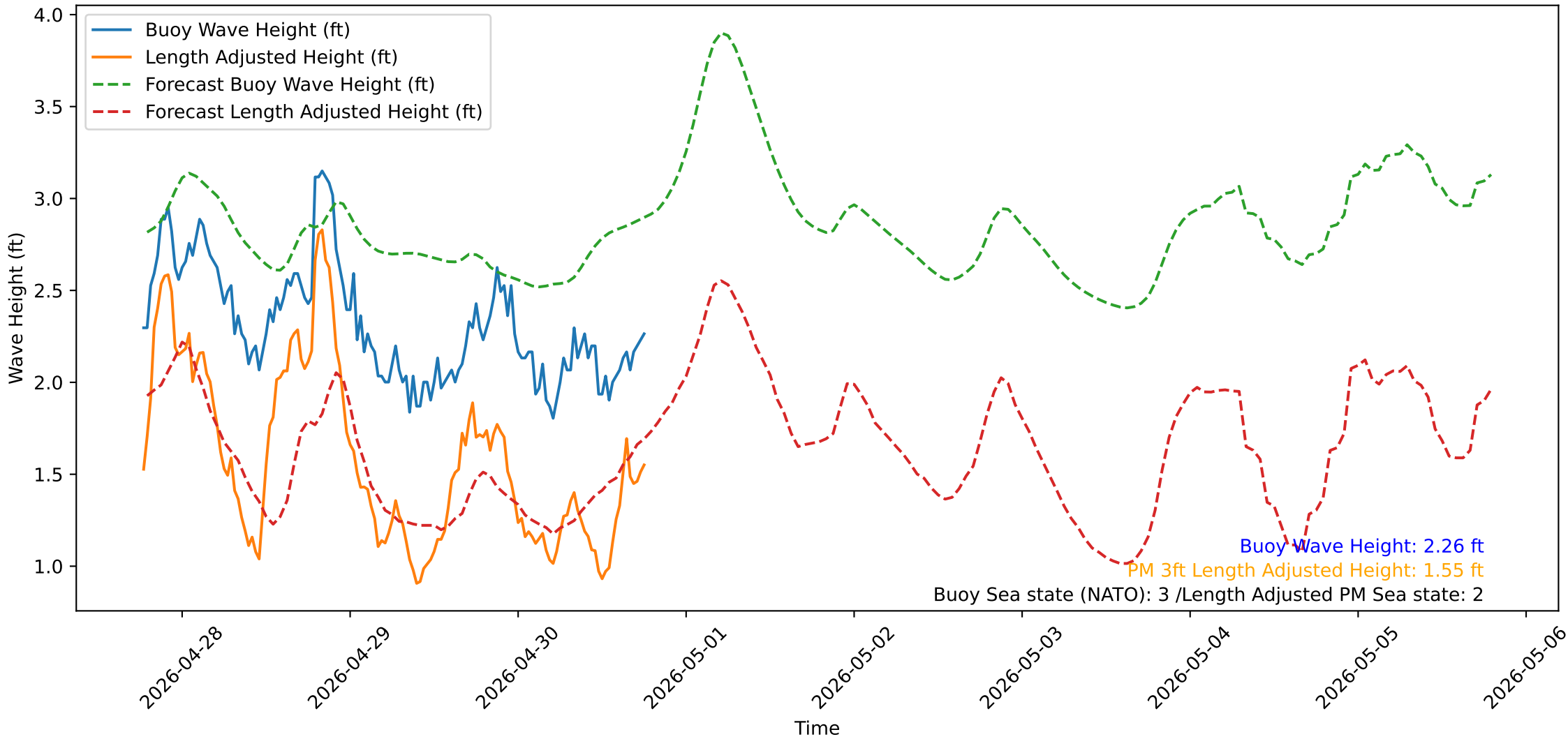
Wave Heights over Time for Green Beach at 2026-04-30 18:41:13
