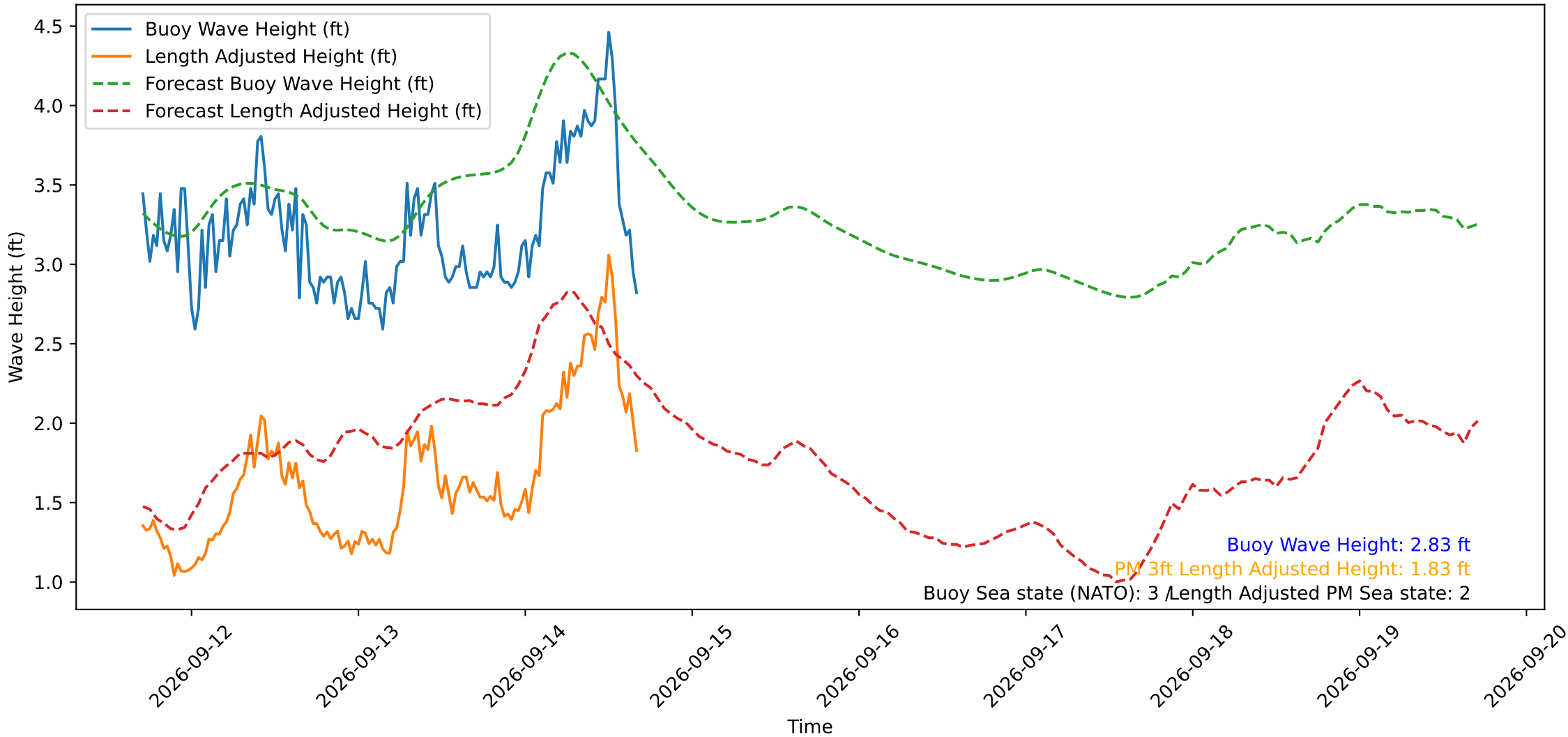
Wave Heights over Time for Oceanside Harbor at 2026-09-14 16:50:29
