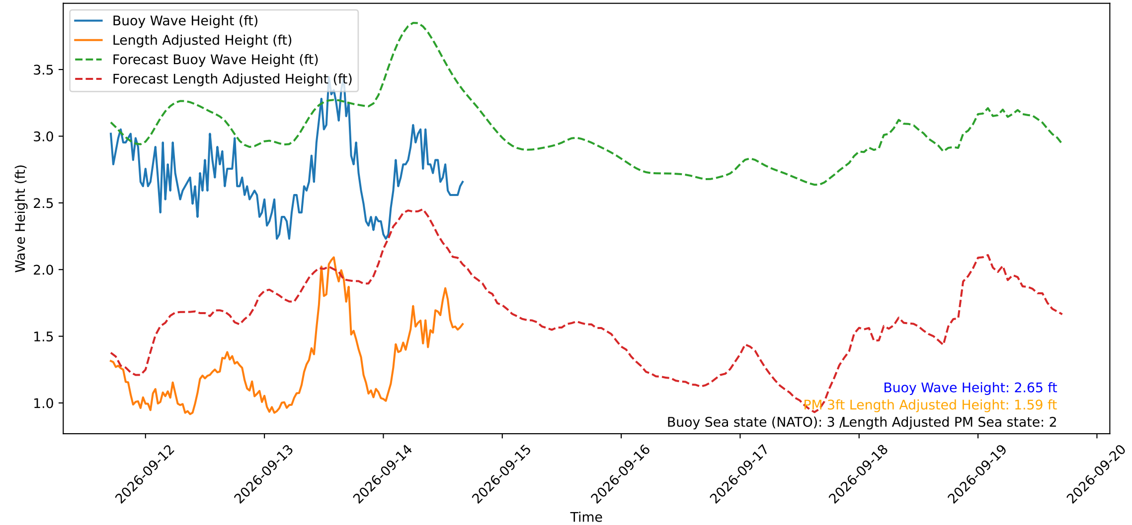
Wave Heights over Time for Red Beach at 2026-09-14 16:50:50
