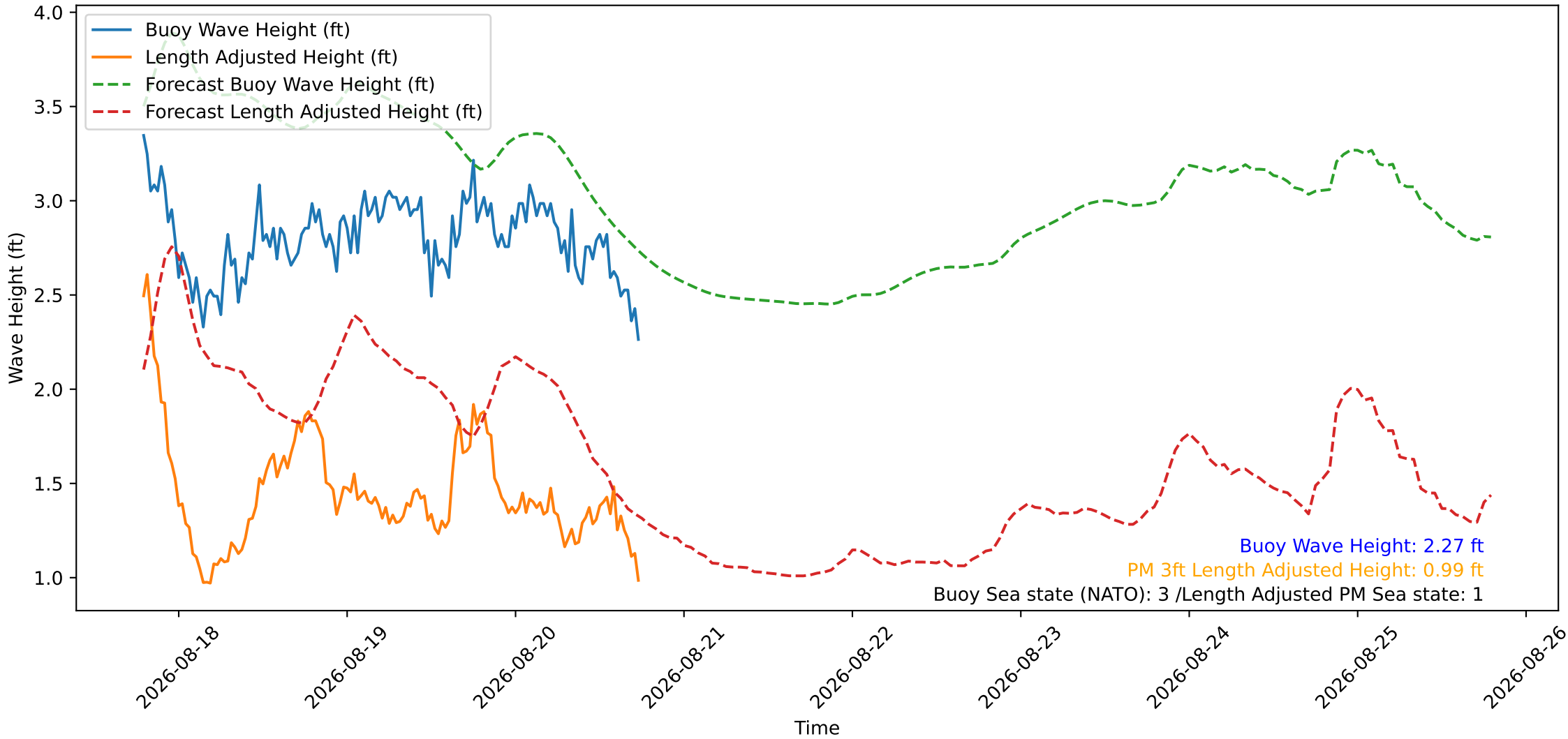
Wave Heights over Time for Red Beach at 2026-08-20 18:40:45
