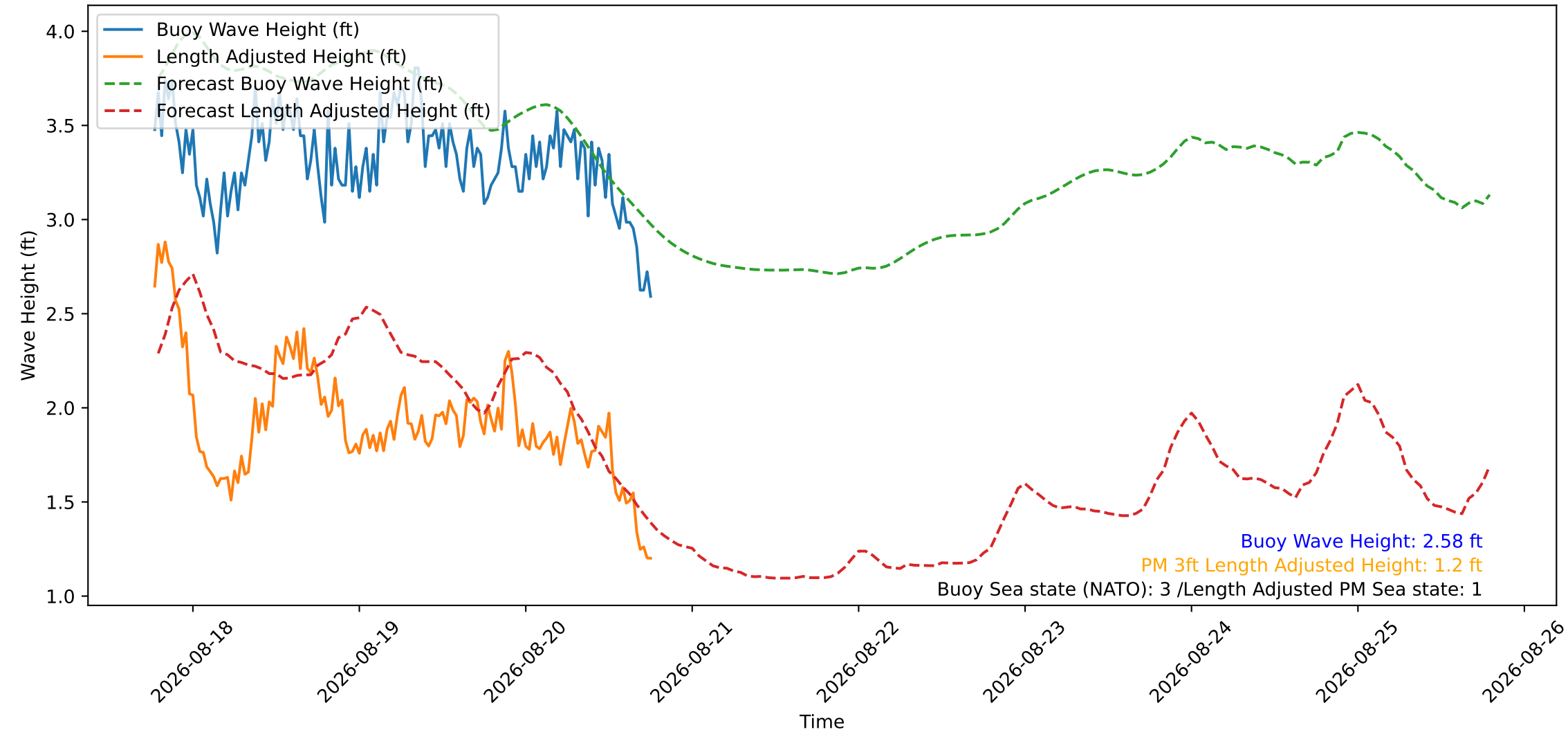
Wave Heights over Time for Oceanside Harbor at 2026-08-20 18:40:26
