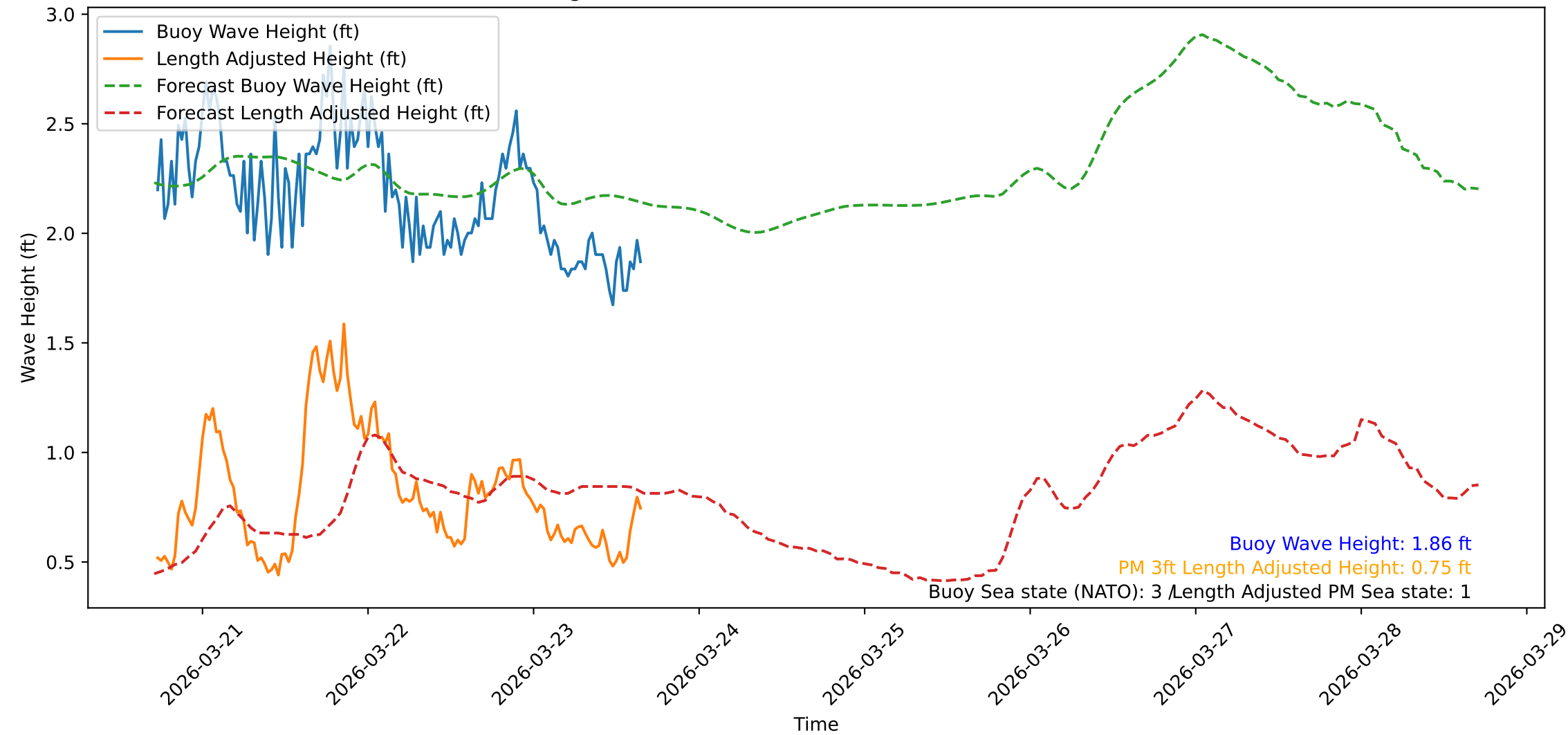
Wave Heights over Time for Red Beach at 2026-03-23 17:10:47
