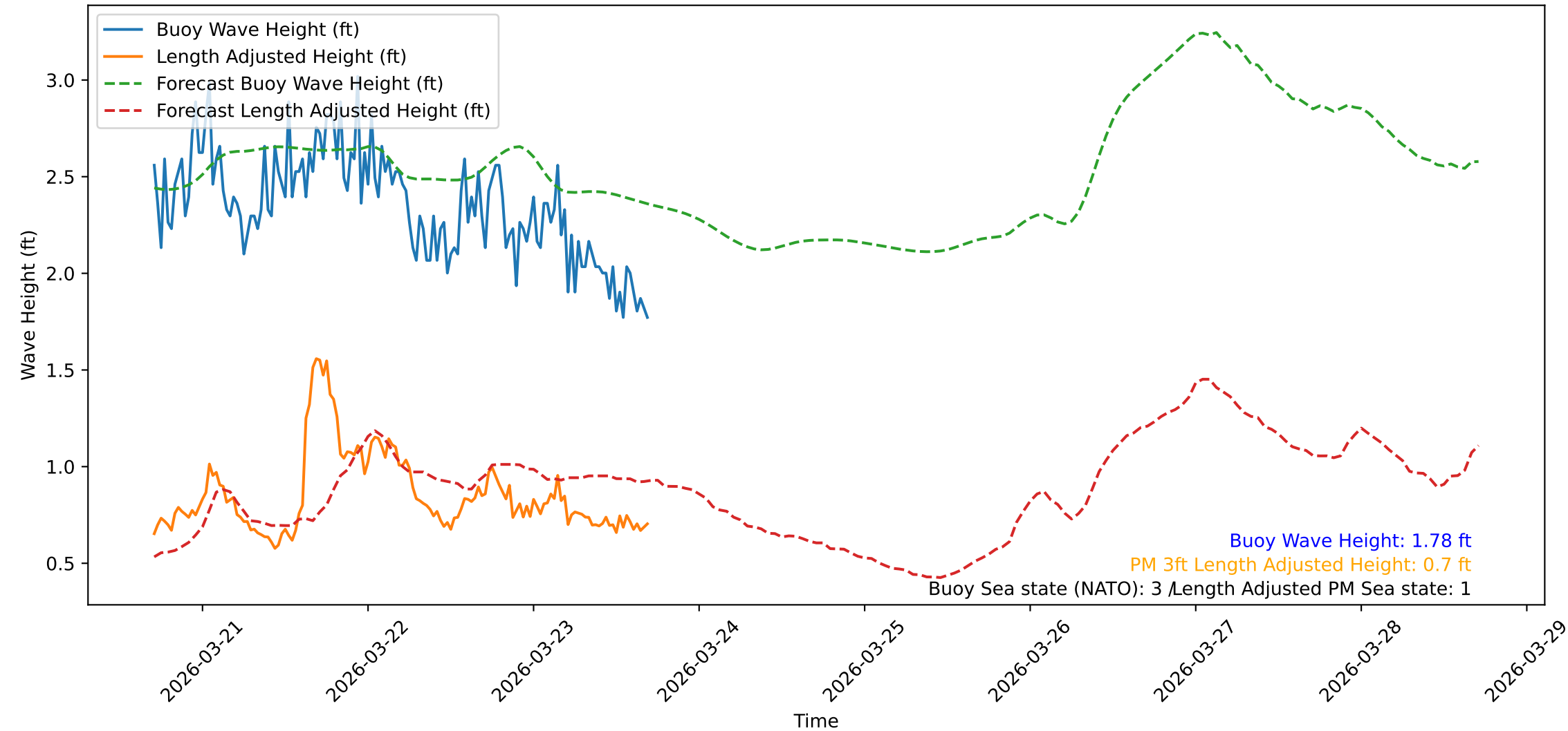
Wave Heights over Time for Oceanside Harbor at 2026-03-23 17:10:32
