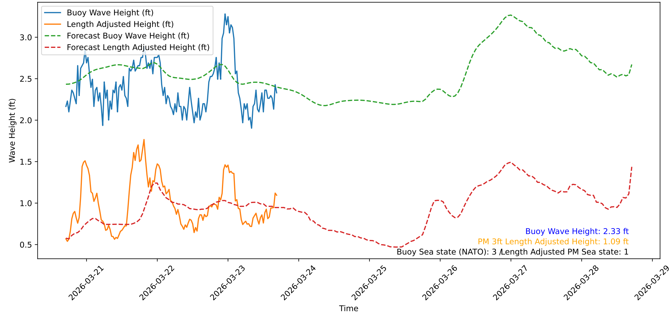
Wave Heights over Time for Green Beach at 2026-03-23 17:11:09
