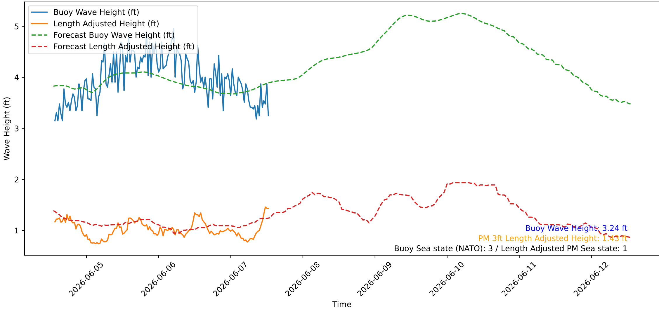
Wave Heights over Time for Red Beach at 2026-06-07 13:20:46
