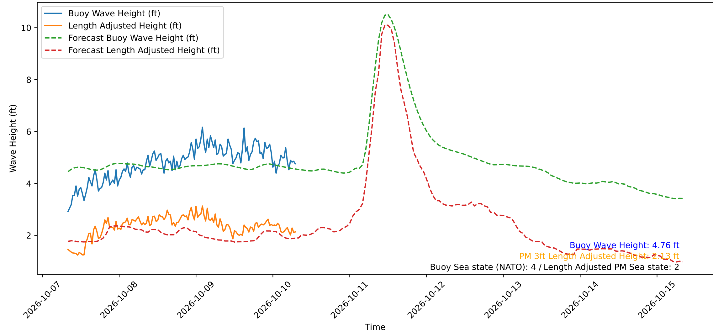
Wave Heights over Time for Green Beach at 2026-10-10 07:41:12
