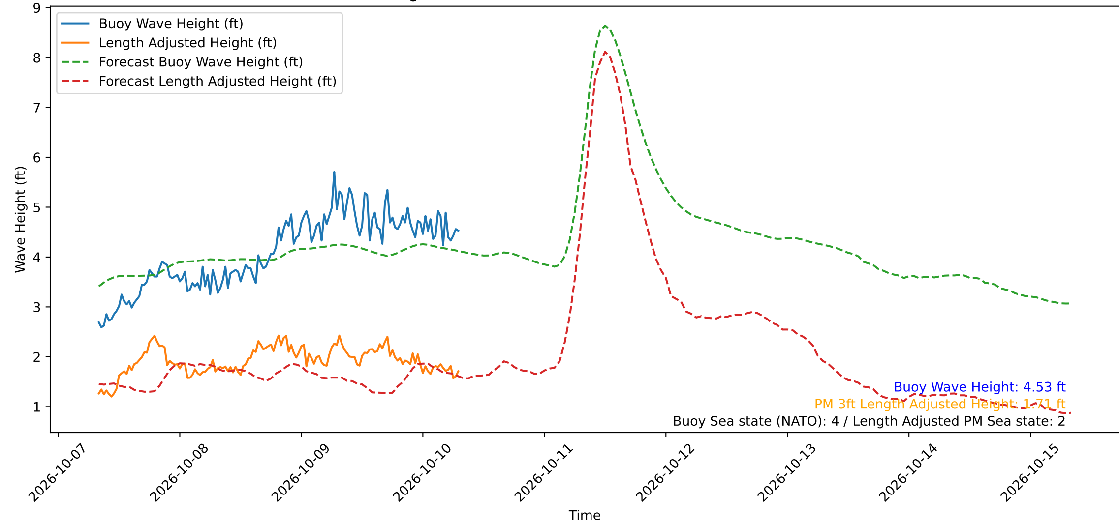
Wave Heights over Time for Red Beach at 2026-10-10 07:40:49
