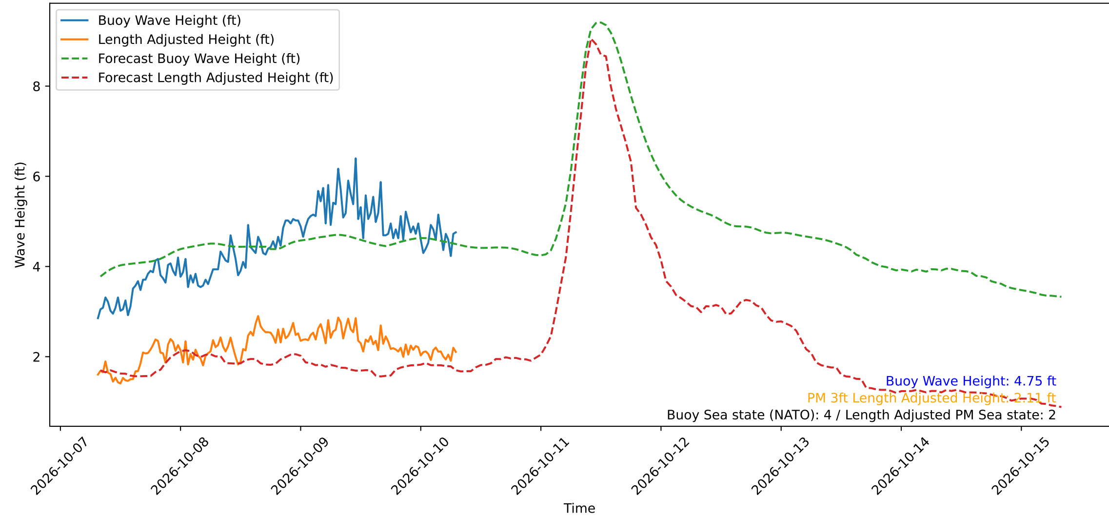
Wave Heights over Time for Oceanside Harbor at 2026-10-10 07:40:30
