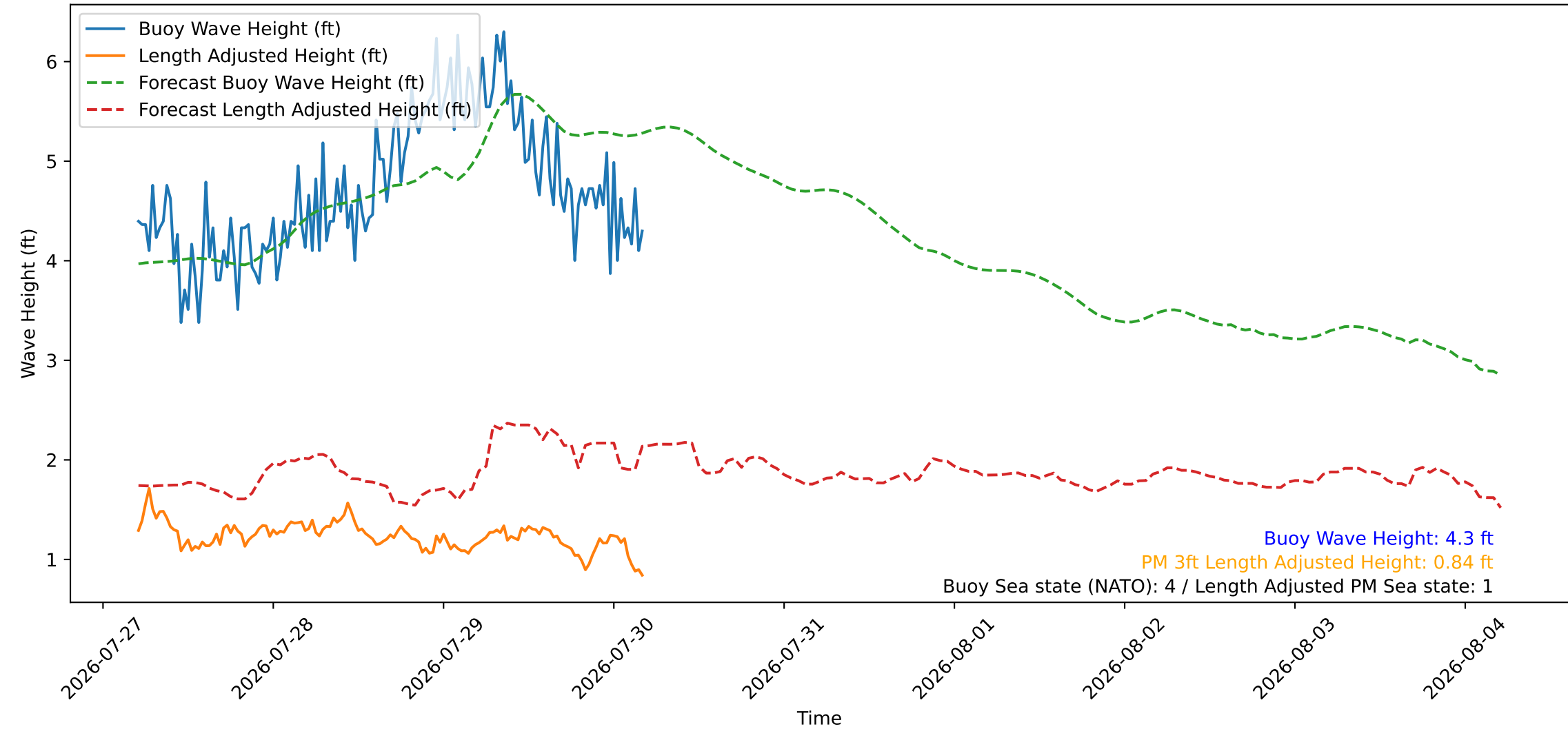
Wave Heights over Time for Green Beach at 2026-07-30 05:01:08
