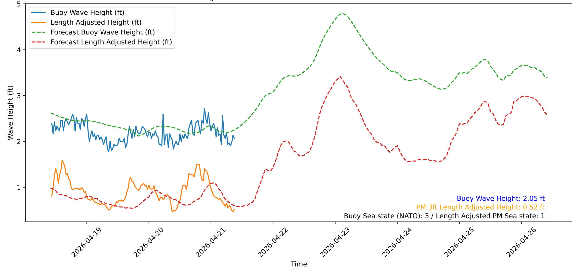
Wave Heights over Time for Red Beach at 2026-04-21 10:00:51
