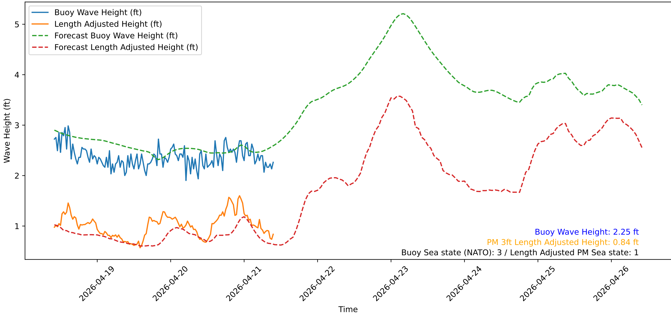
Wave Heights over Time for Oceanside Harbor at 2026-04-21 10:00:32
