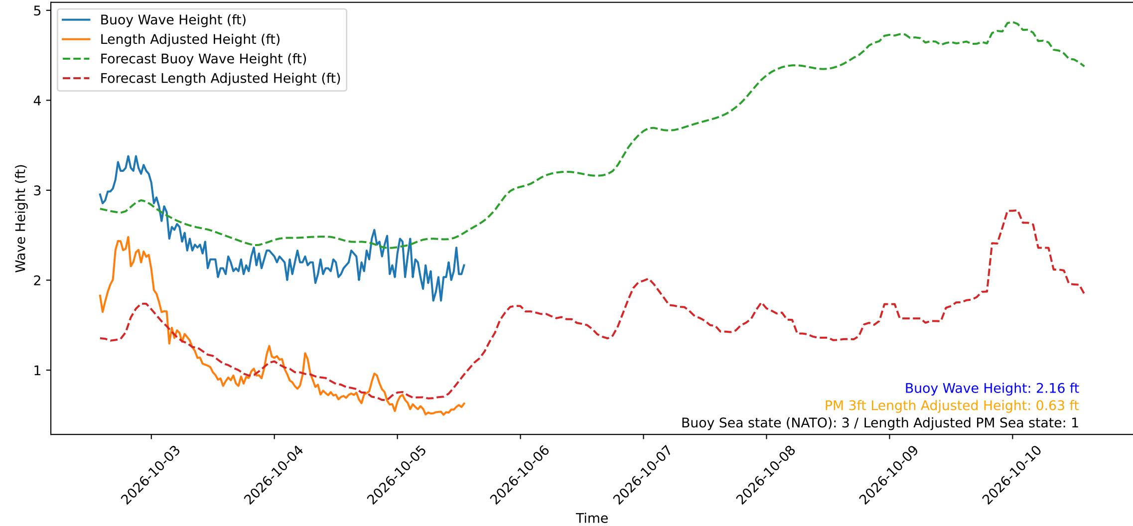
Wave Heights over Time for Green Beach at 2026-10-05 13:51:14
