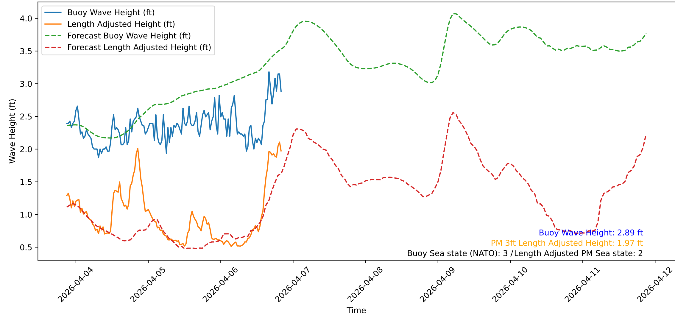
Wave Heights over Time for Red Beach at 2026-04-06 20:50:47
