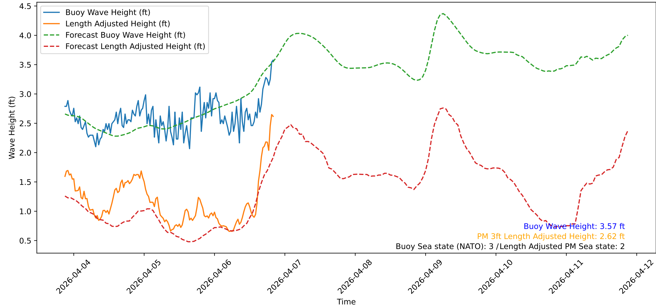
Wave Heights over Time for Oceanside Harbor at 2026-04-06 20:50:31
