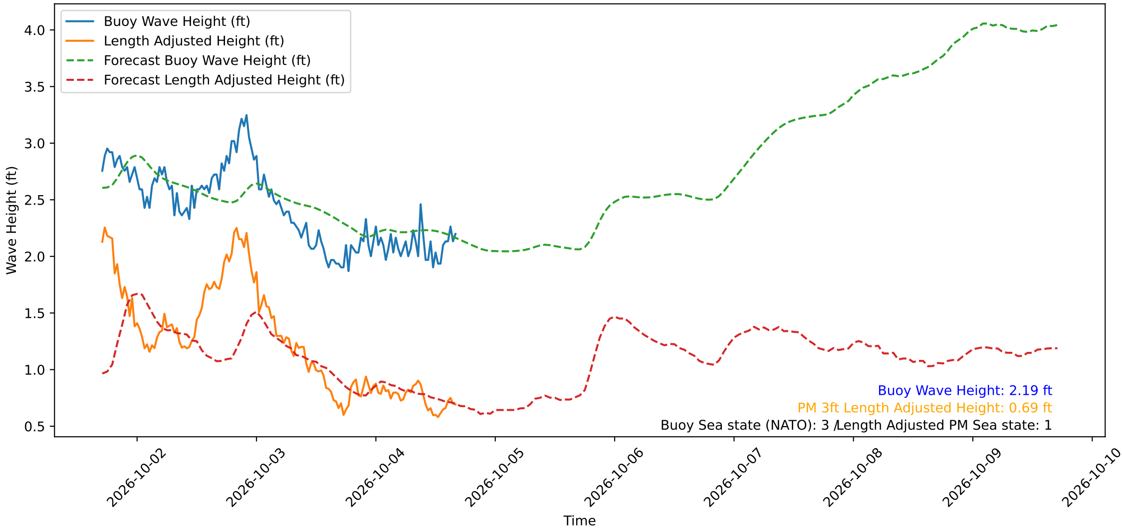
Wave Heights over Time for Red Beach at 2026-10-04 16:40:50
