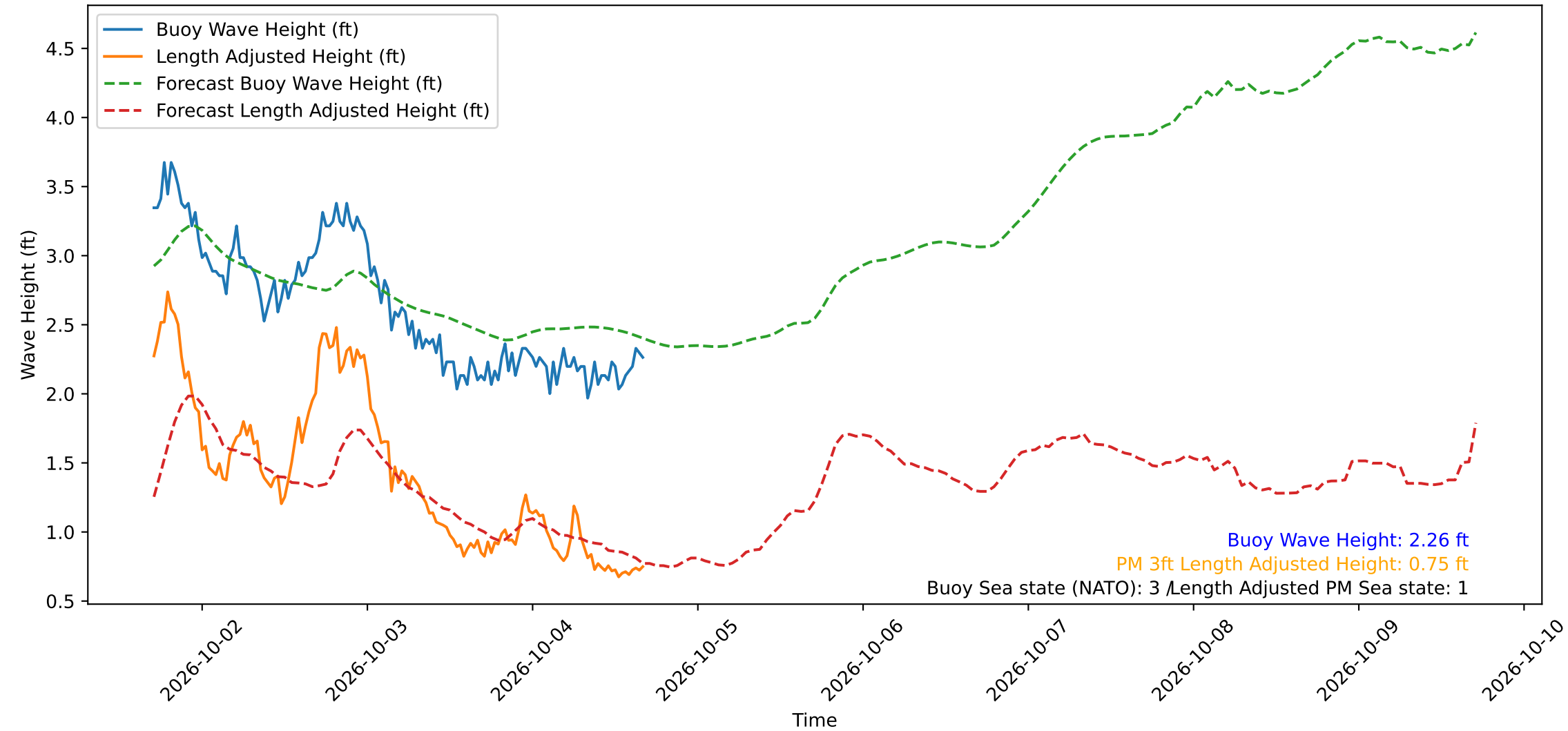
Wave Heights over Time for Green Beach at 2026-10-04 16:41:12
