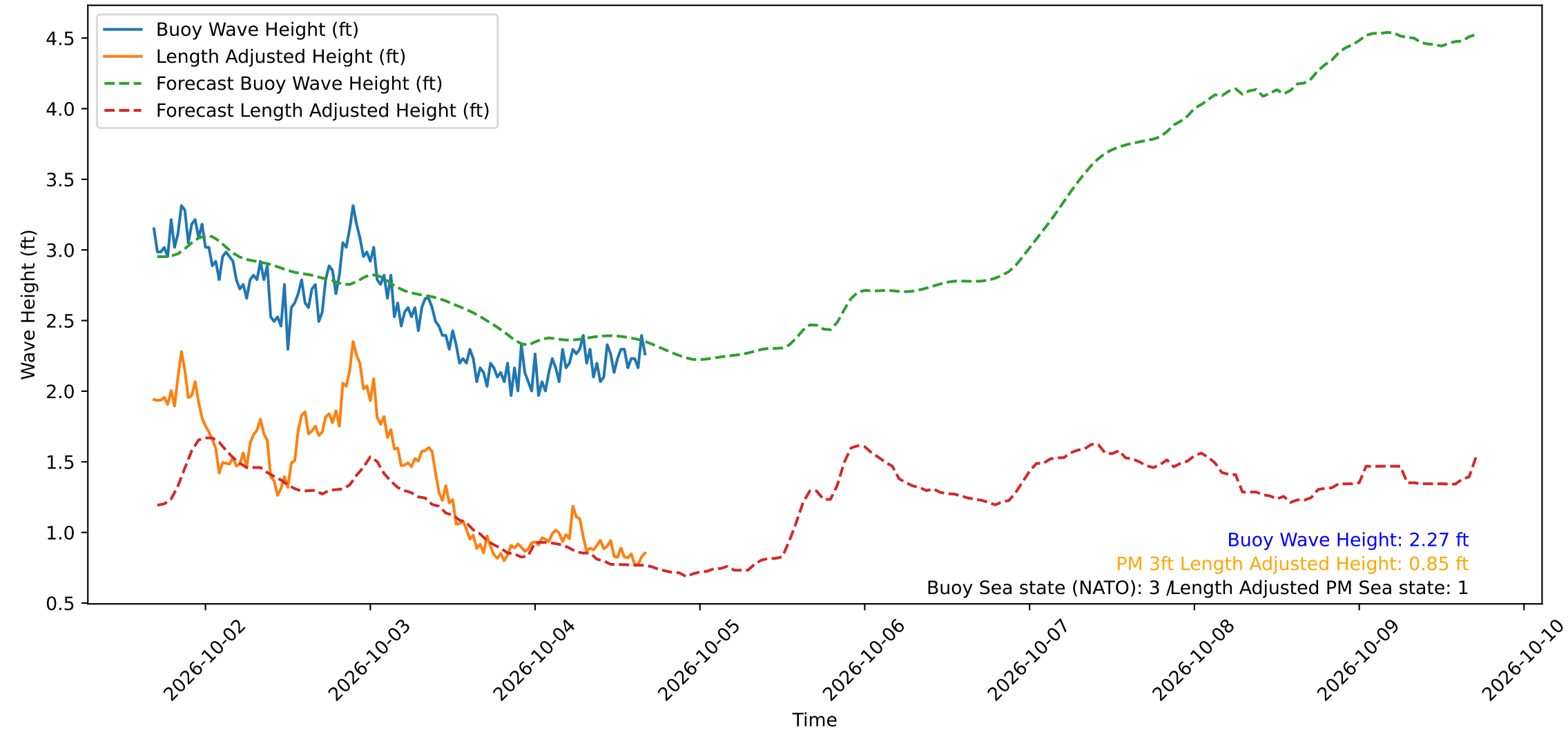
Wave Heights over Time for Oceanside Harbor at 2026-10-04 16:40:30
