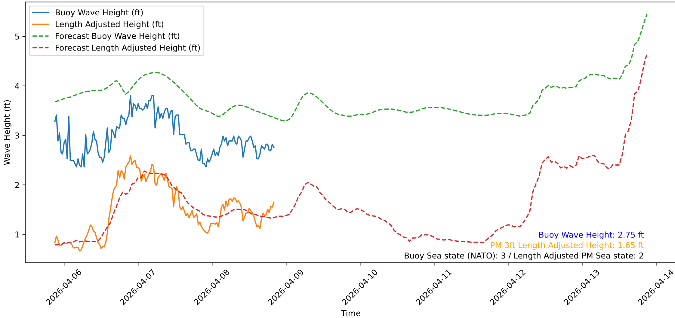
Wave Heights over Time for Green Beach at 2026-04-08 20:51:12
