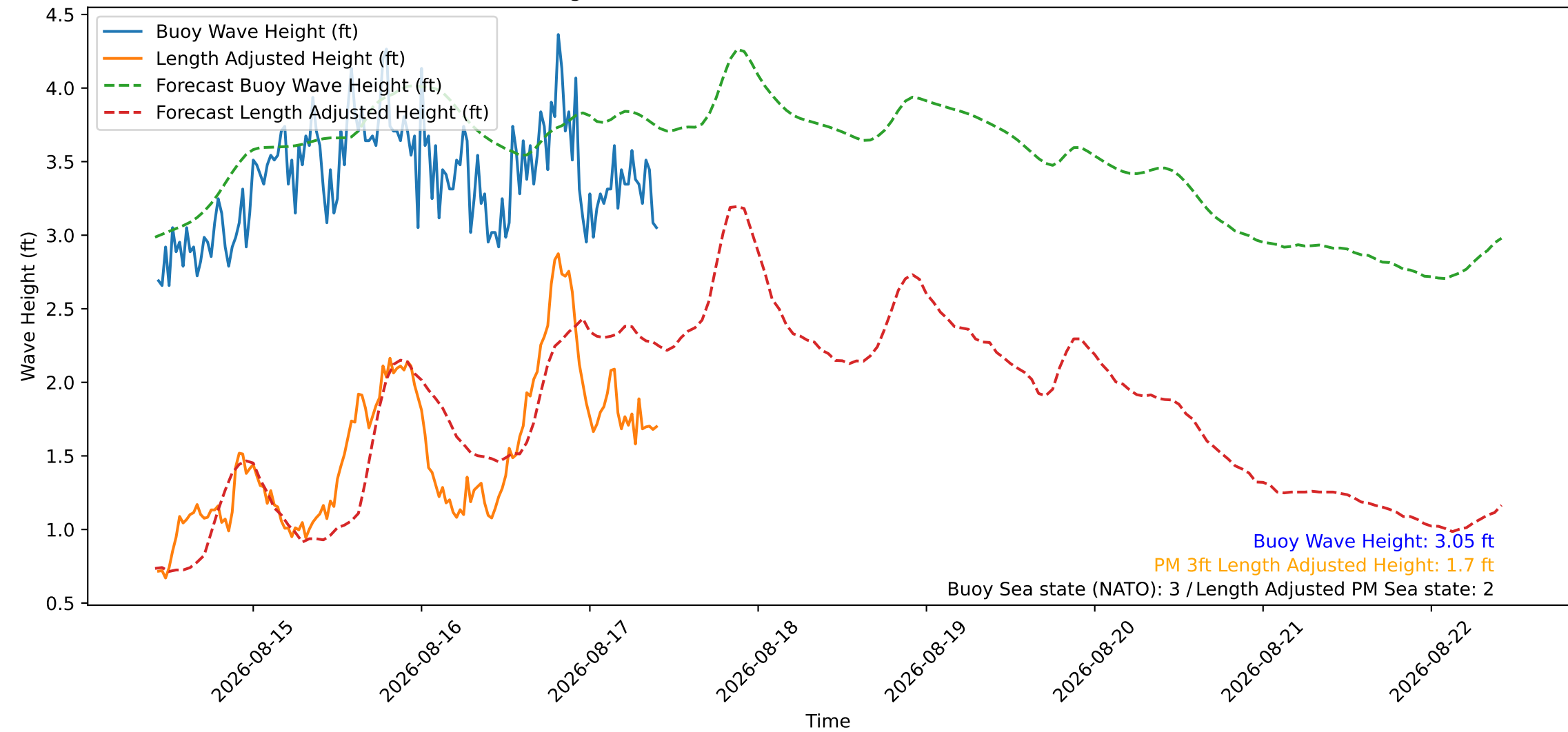
Wave Heights over Time for Green Beach at 2026-08-17 10:21:11
