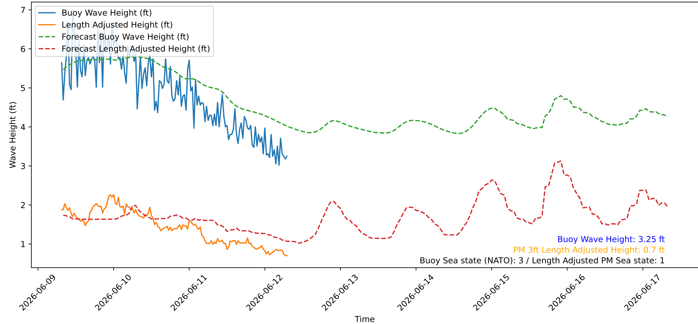
Wave Heights over Time for Green Beach at 2026-06-12 07:41:09
