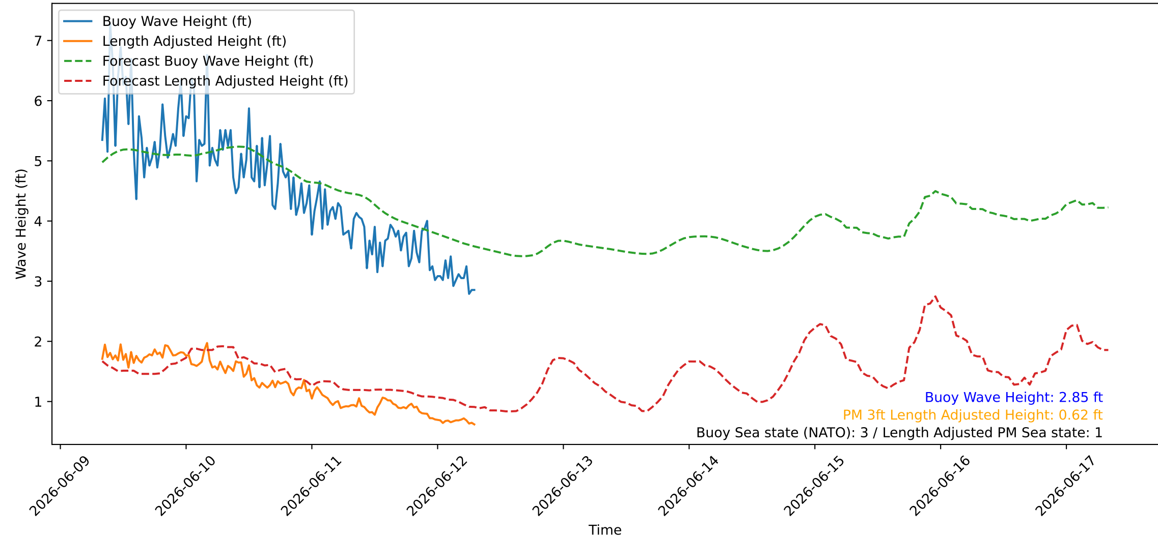
Wave Heights over Time for Red Beach at 2026-06-12 07:40:45
