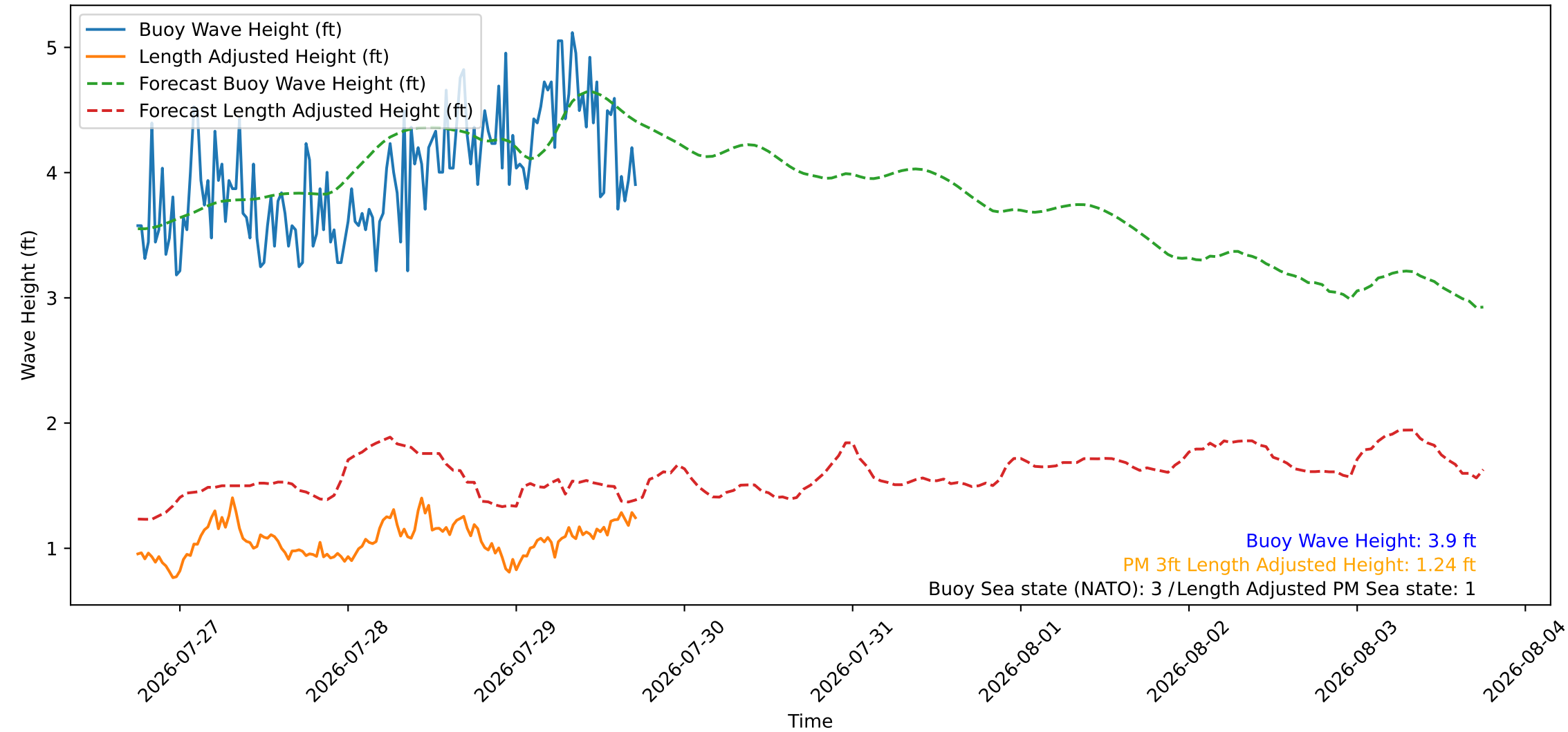
Wave Heights over Time for Red Beach at 2026-07-29 17:50:48
