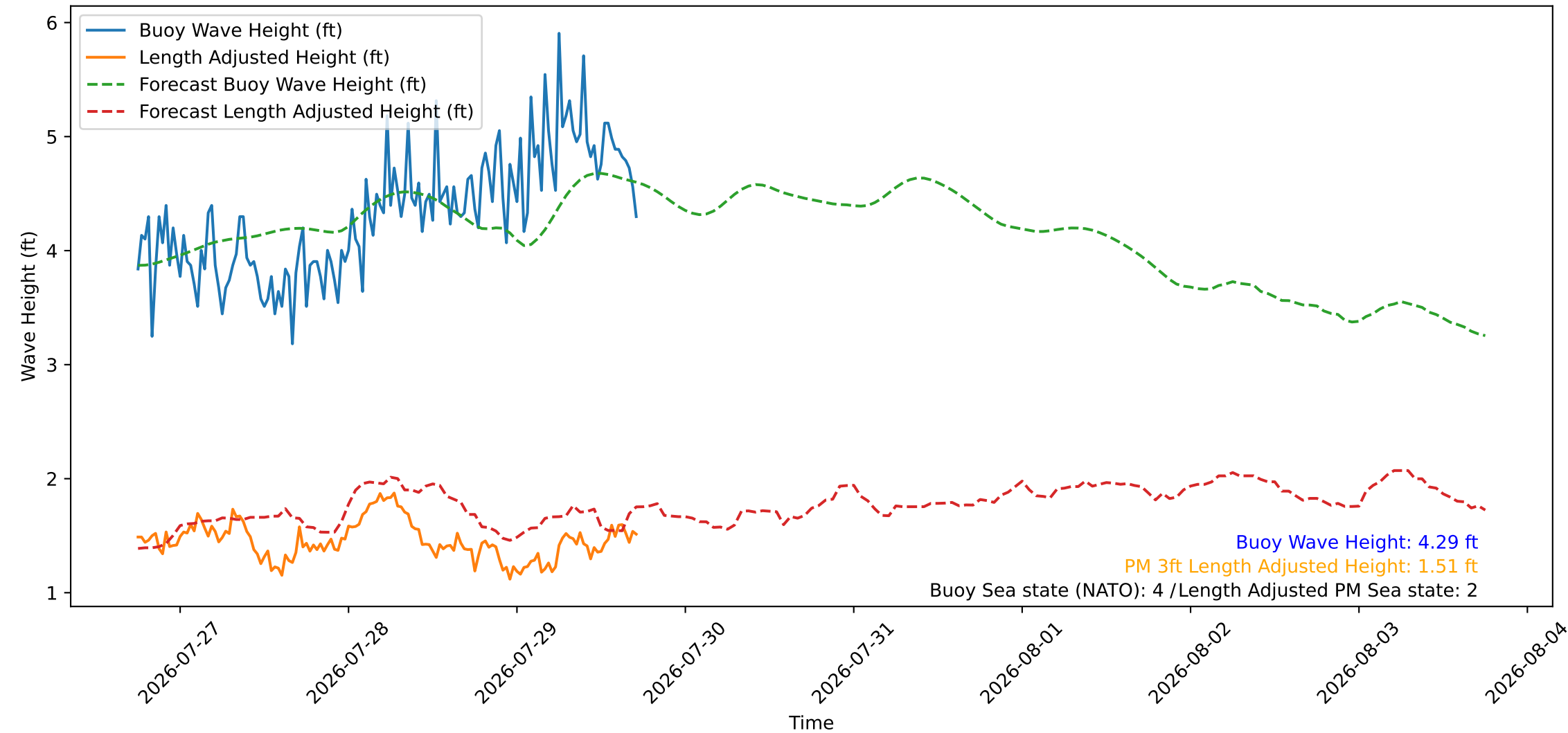
Wave Heights over Time for Oceanside Harbor at 2026-07-29 17:50:27
