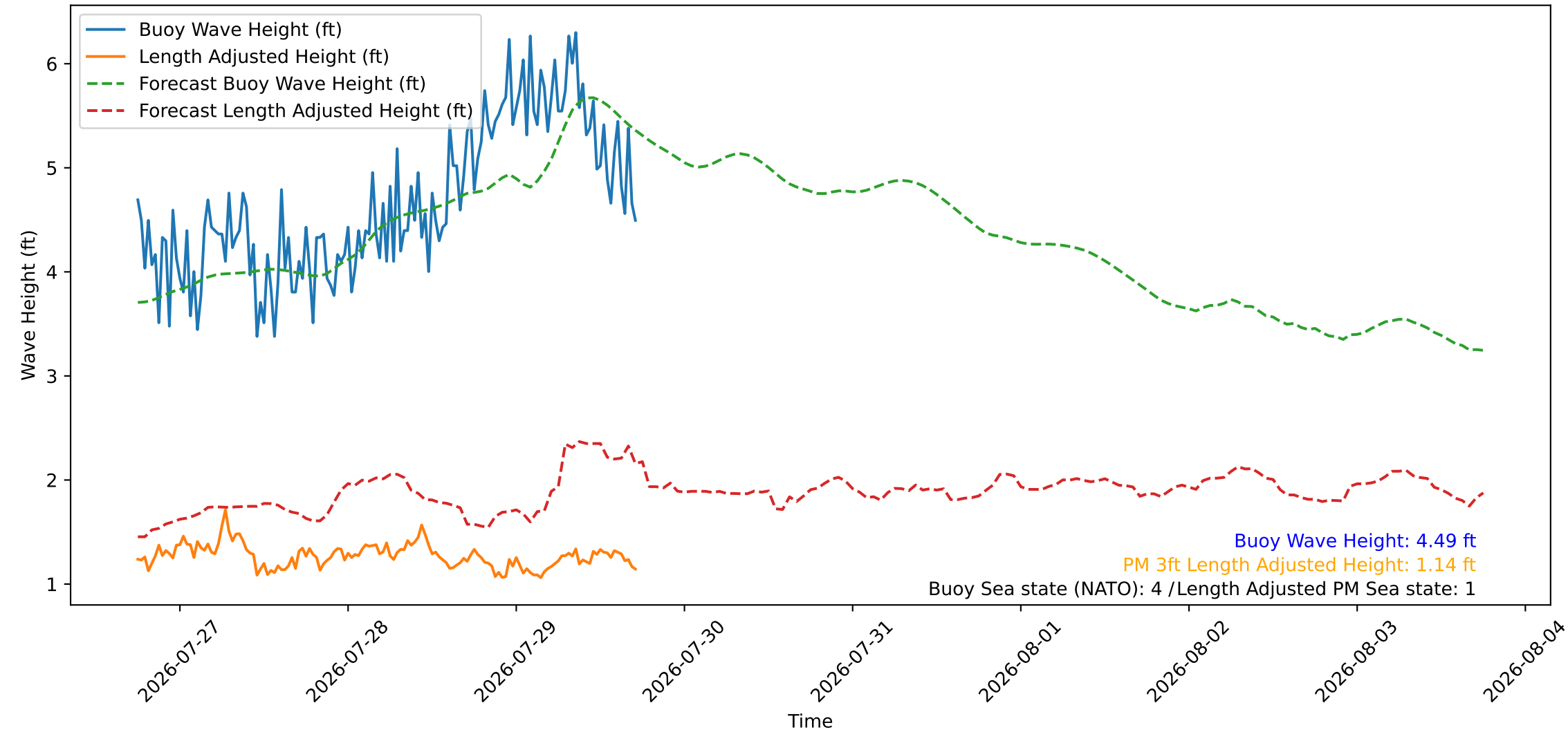
Wave Heights over Time for Green Beach at 2026-07-29 17:51:11
