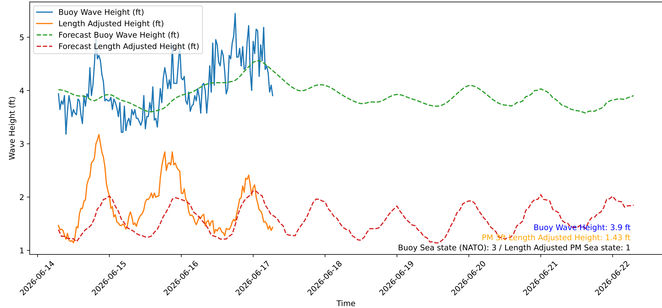
Wave Heights over Time for Oceanside Harbor at 2026-06-17 07:10:26
