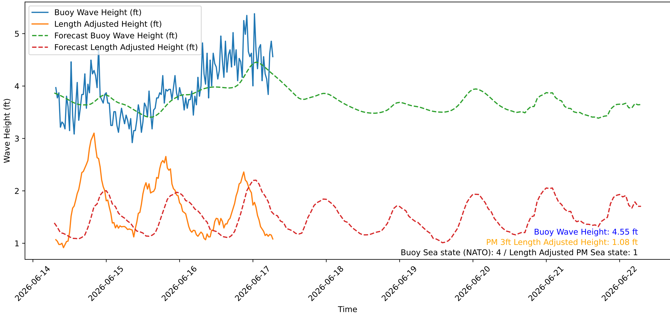
Wave Heights over Time for Red Beach at 2026-06-17 07:10:46
