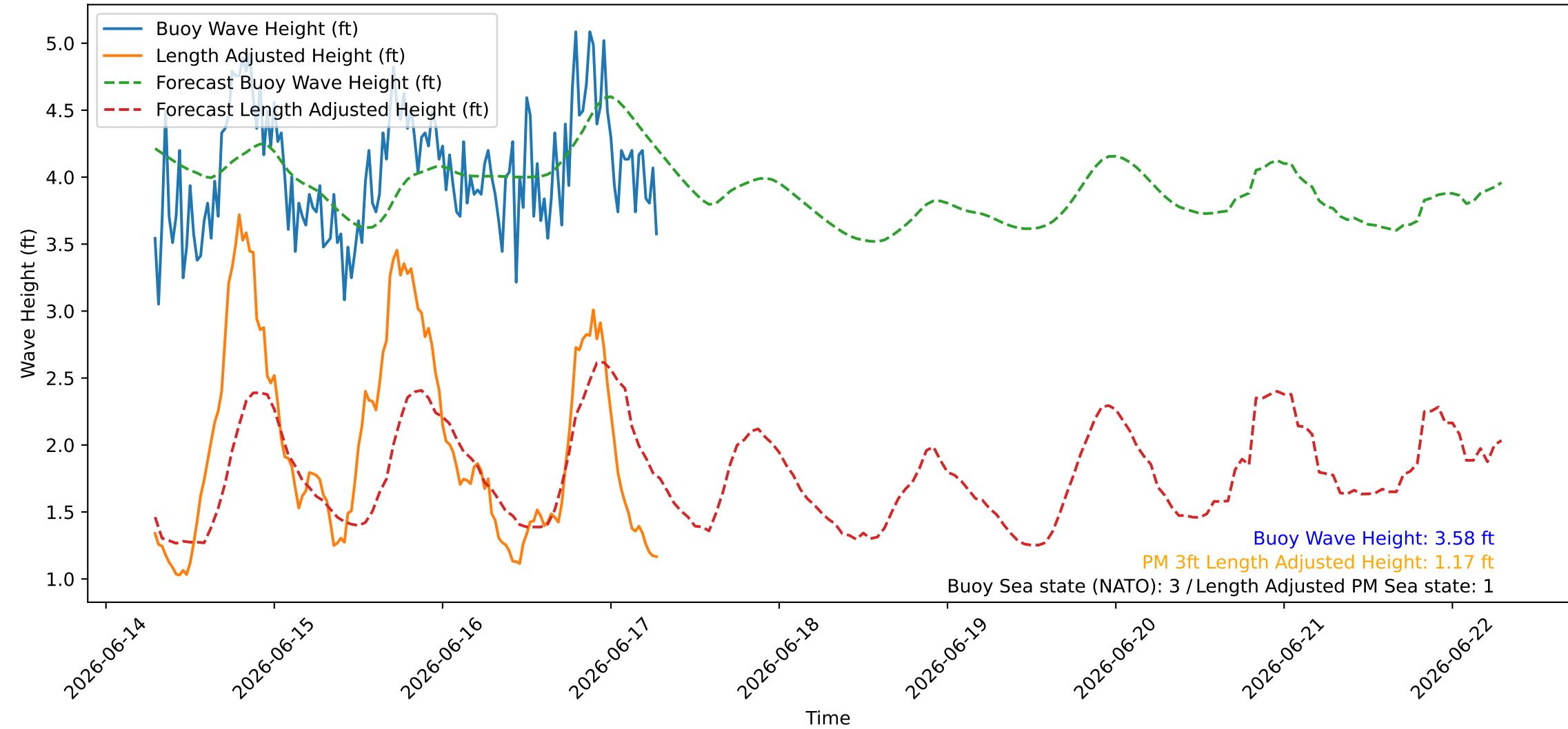
Wave Heights over Time for Green Beach at 2026-06-17 07:11:09
