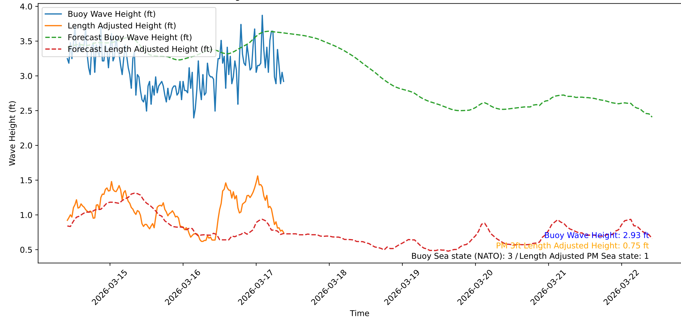
Wave Heights over Time for Oceanside Harbor at 2026-03-17 09:50:47
