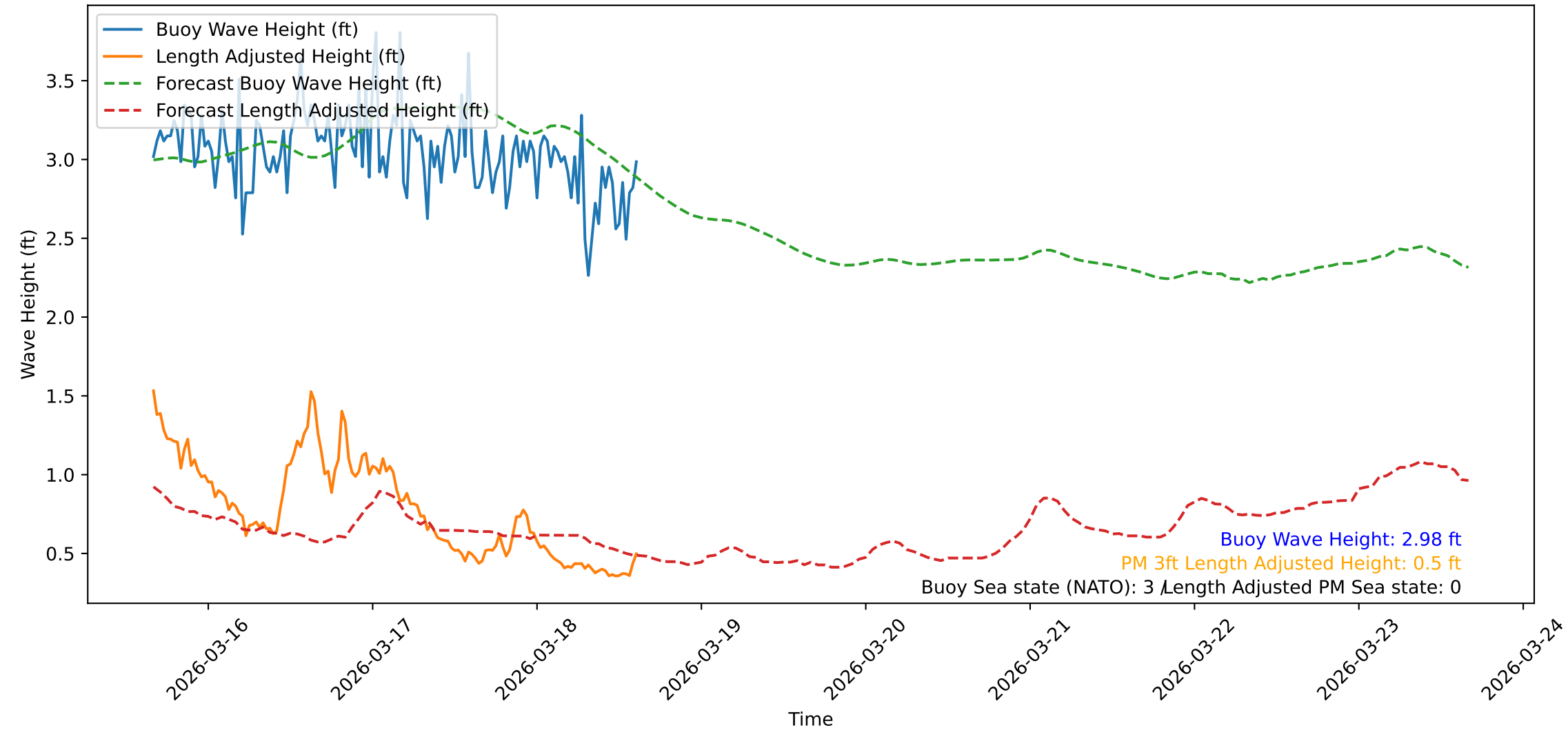
Wave Heights over Time for Red Beach at 2026-03-18 15:30:47
