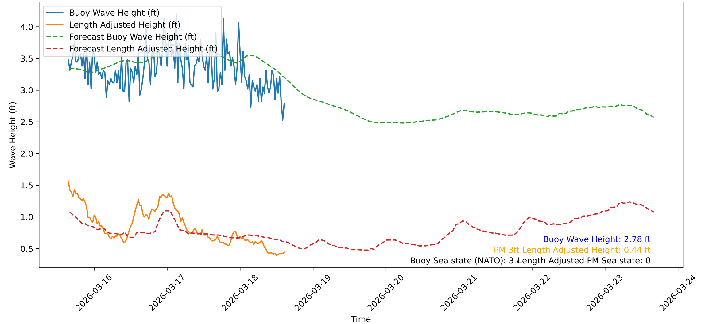
Wave Heights over Time for Green Beach at 2026-03-18 15:31:10
