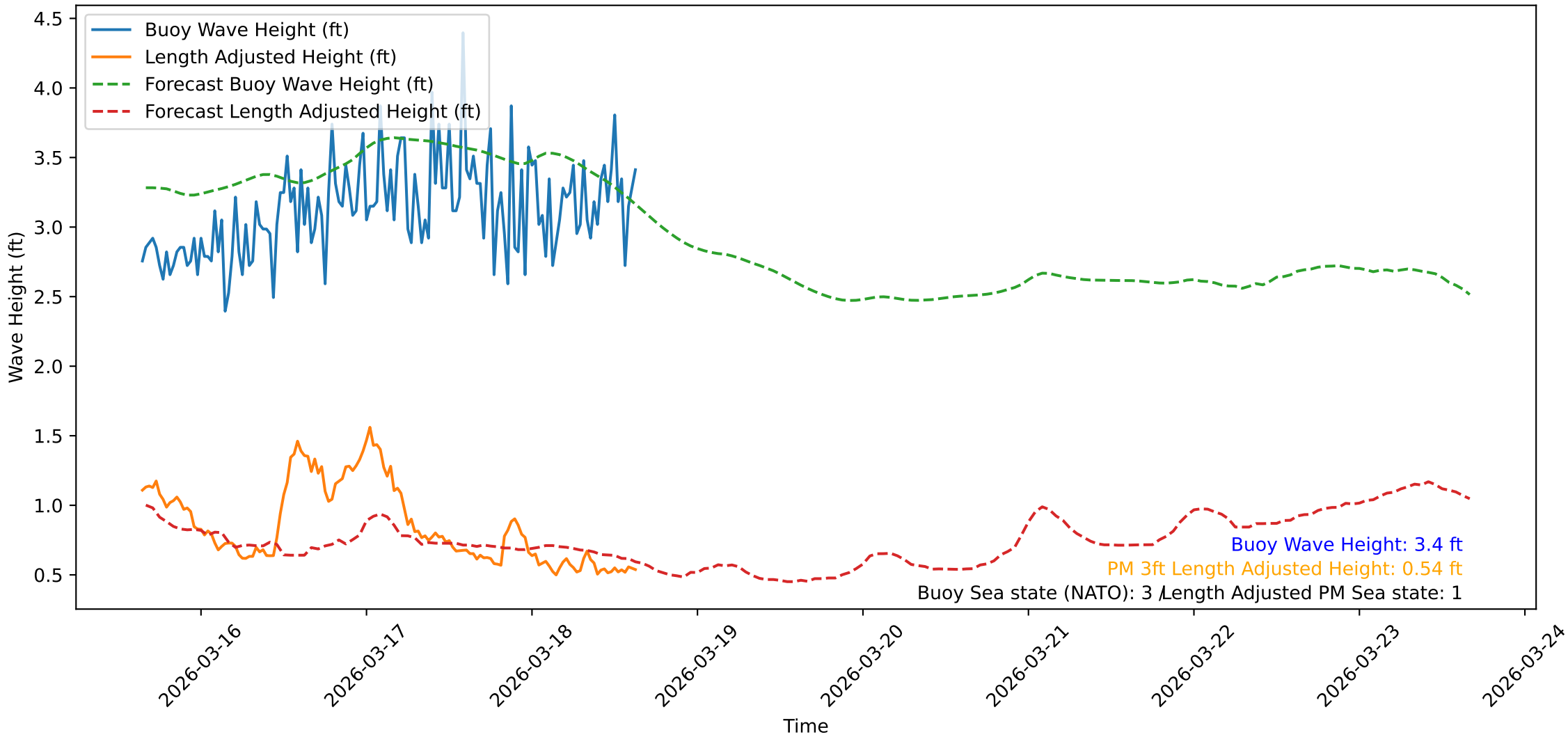
Wave Heights over Time for Oceanside Harbor at 2026-03-18 15:30:31
